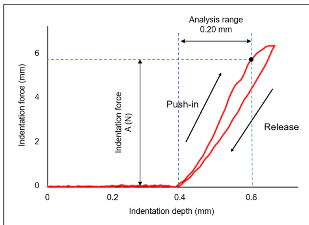
Figure 3. Graph for indentation depth and indentation force depicted on the dedicated application. Elastic modulus (N/mm) was calculated as A \text{ (N)}/0.2 \text{ (mm)} .
