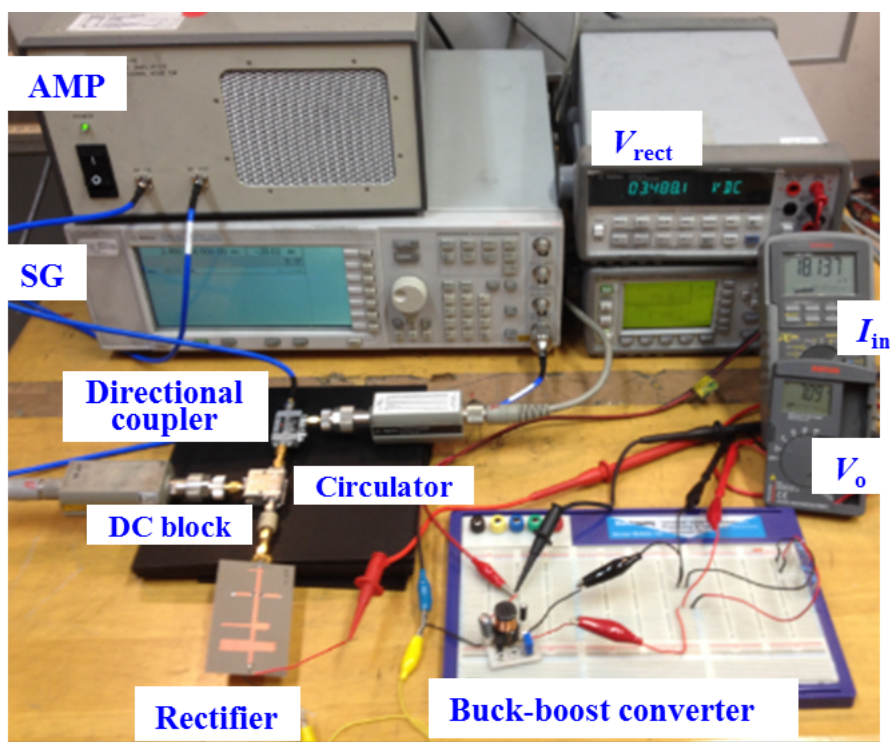
Figure 4.12: Experiment setup for measuring the efficiency of the self-powered RF-DC-DC circuit. (a) Experiment setup. (b) Experiment photograph.
