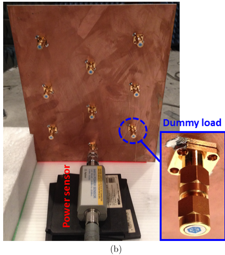
Figure 5.16: Experiment setup for measuring the receiving power of the antenna array. (a) Experiment setup. (b) Photograph of the antenna array setup. Power sensor measures the receiving power of each antenna with all other antennas connected to a 50\ \Omega dummy load.
