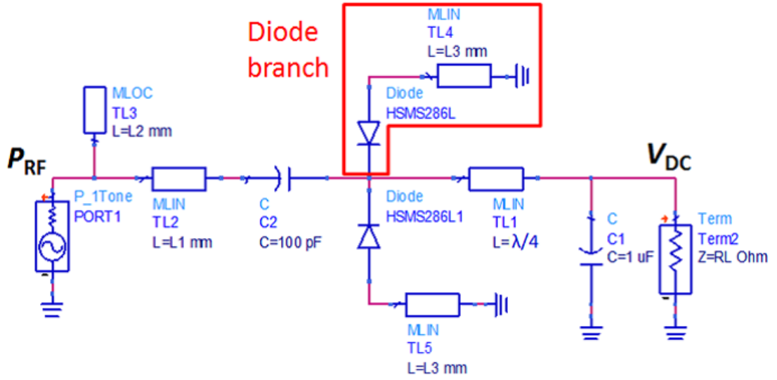
Figure 2.1: Circuit diagram of a simple quarter-wave single shunt rectifier.
