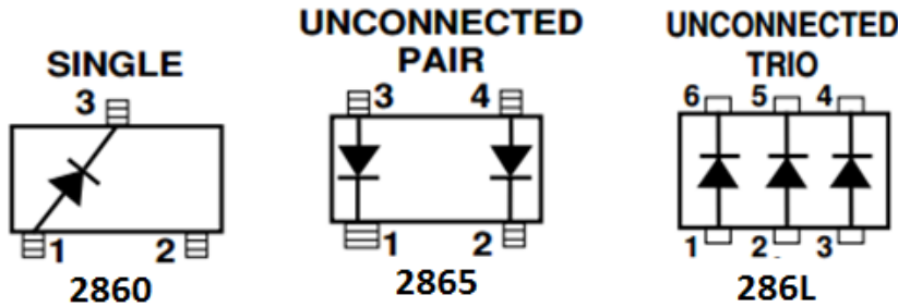
Figure 2.2: Top view of three rectifying diodes.
