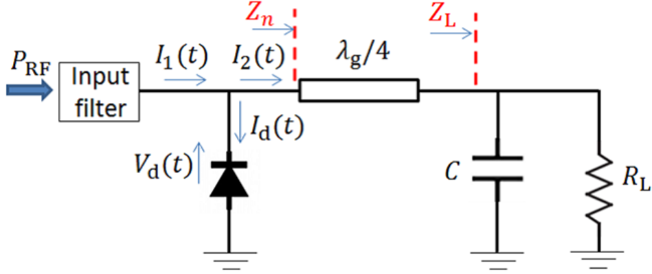
Figure A.2: Block diagram of a single shunt rectifying circuit. It usually contains an input filter, a rectifying diode, a \lambda_g/4 line, a capacitor and a load.
