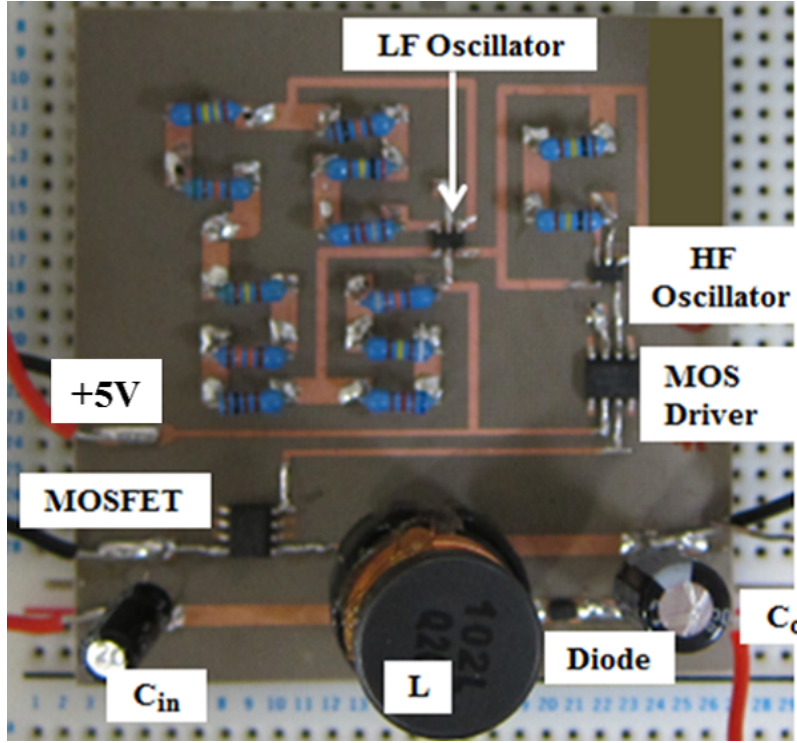
Figure 3.5: Photograph of the inverting DCM buck-boost converter.
