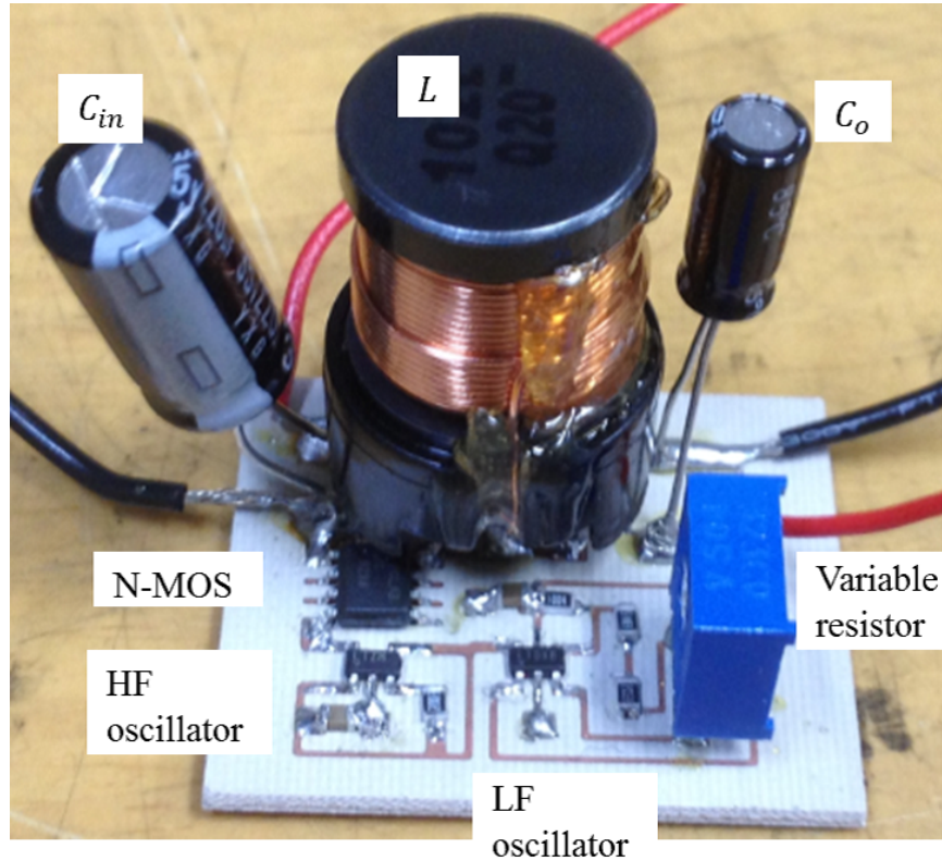
Figure 4.8: Photograph of the self-powered non-inverting buck-boost converter.
