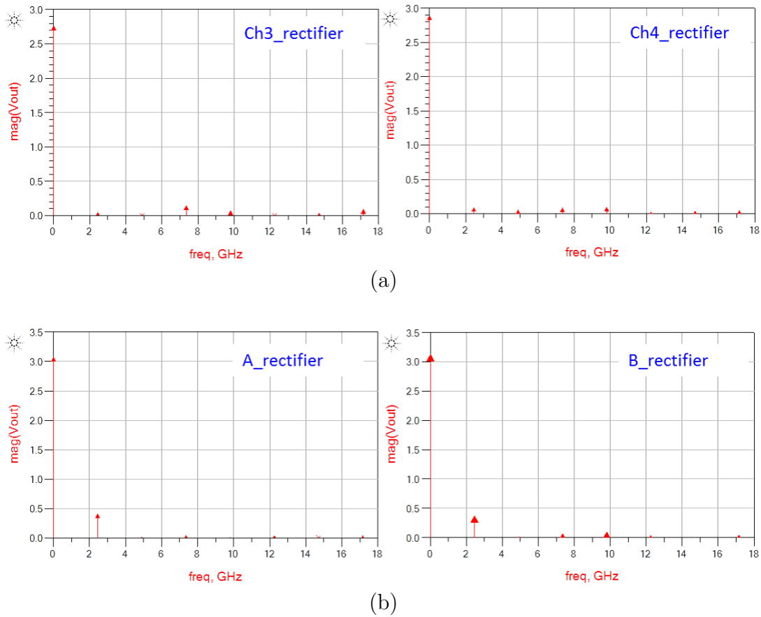
Figure 5.6: Simulated output voltage spectrum of rectifiers. (a) Ch3_rectifier and Ch4_rectifier are the rectifiers (with \lambda/4 line) designed in Chapter 3 and Chapter 4, respectively. (b) A_rectifier and B_rectifier are the rectifiers (without \lambda/4 line) designed in this chapter.
