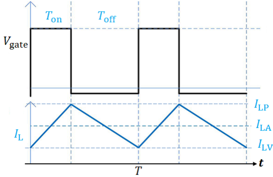
Figure 3.1: Operating waveforms of the inductor current ( I_L ) and gate control voltage ( V_{\text{gate}} ) for a DC-DC converter in CCM.
