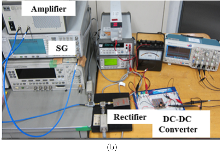
Figure 3.13: Experimental setup for measuring the efficiency of the RF-DC-DC circuit. (a) Block diagram. (b) Experiment photograph.
