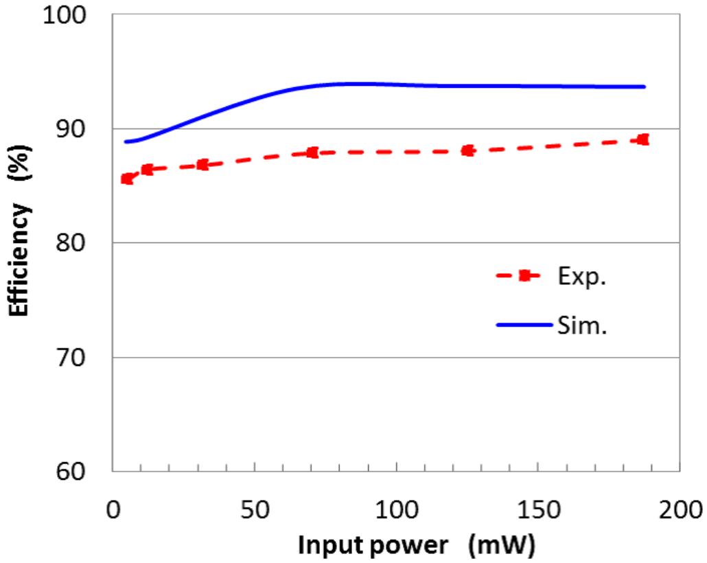
Figure 3.10: Simulation and experimental results of the efficiency vs. input power for a fixed load resistance of 1000\ \Omega .
