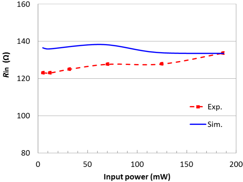
Figure 3.8: Simulation and experimental results of the input resistance R_{in} vs. input power for a fixed load resistance of 1000 \Omega .
