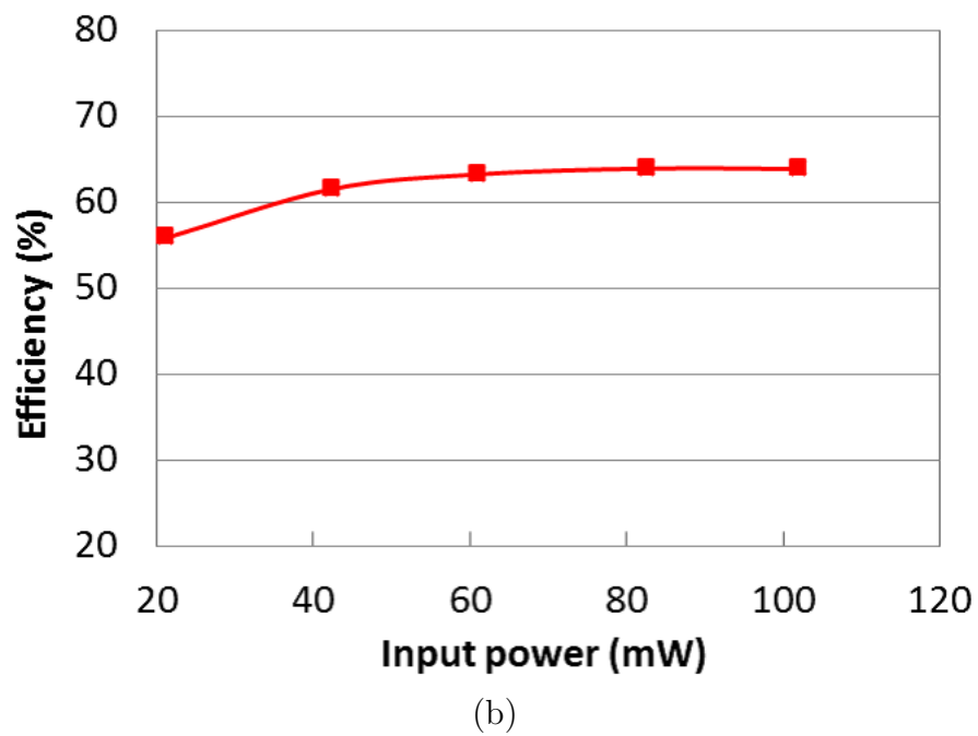
Figure 3.14: Measured overall efficiency of the RF-DC-DC circuit. (a) Efficiency comparison of the RF-DC-DC circuit and the general rectifier for a constant input power of 82 mW. (b) Overall efficiency vs. input power for a constant load of 1000 \Omega .
