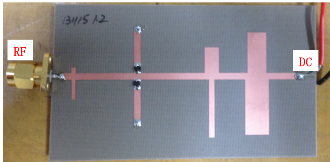
Figure 4.1: Proposed positive output voltage rectifier. (a) Structure and size. (b) Photograph.
