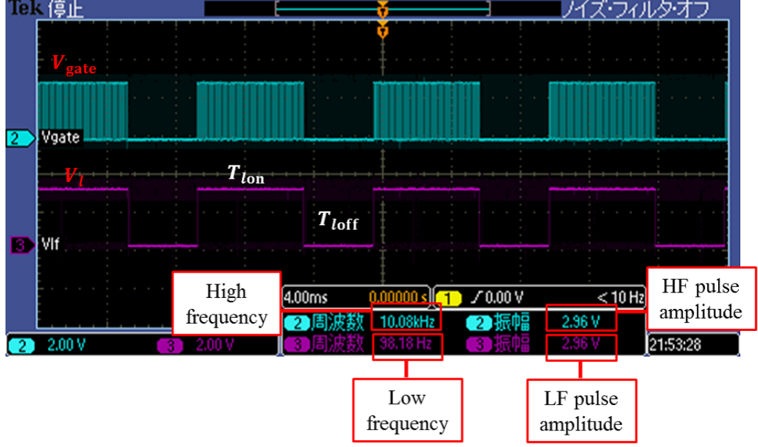
Figure 4.5: Measured waveforms of the control-pulse circuit.
