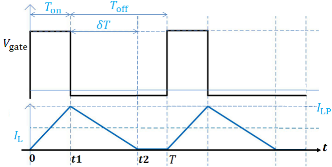
Figure 3.3: Operating waveforms of the inductor current ( I_L ) and gate control voltage ( V_{\text{gate}} ) for a DC-DC converter in DCM.
