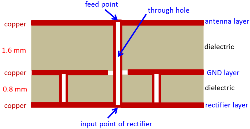
Figure 5.14: Side-view diagram of the multilayer substrate.
