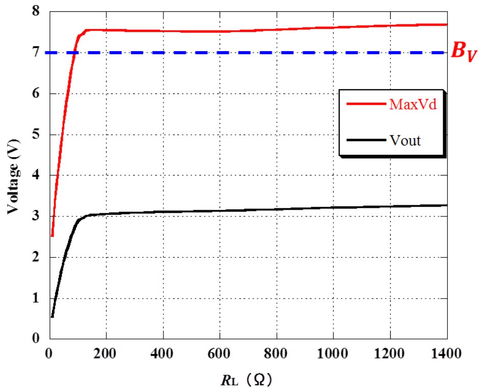
Figure 2.5: Maximum voltage applied on the rectifying diode ( \text{Max}V_d ), output voltage of the rectifier ( V_{out} ).
