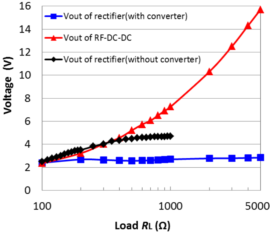
Figure 3.16: Measured output voltage vs. load resistance for a constant input power of 82 mW.
