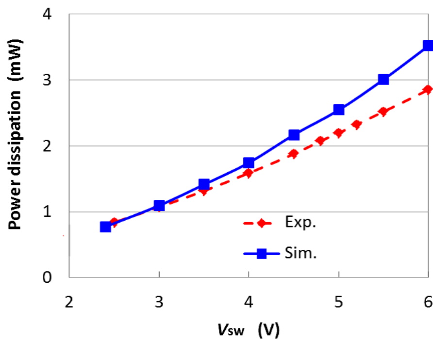
Figure 4.6: Simulation and experimental results of the control-pulse circuit. (a) Impedance Z_{sw} . (b) Power consumption.
