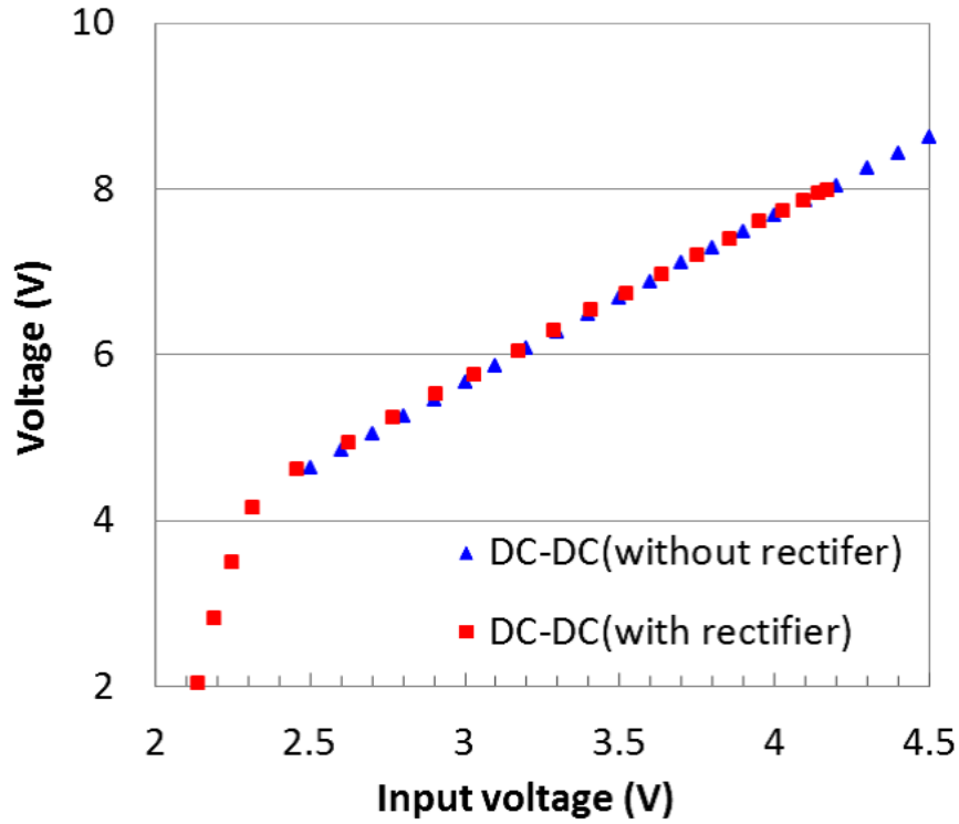
Figure 4.18: Input/output voltage relationships of the buck-boost converter in RF-DC-DC circuit.
