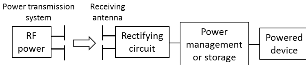
Figure 1.4: Block diagram of a MPT system. An RF power transmission system transmits microwave incident on a receiving antenna (array). After rectification and management, the DC power can afford to power an electrical device.
