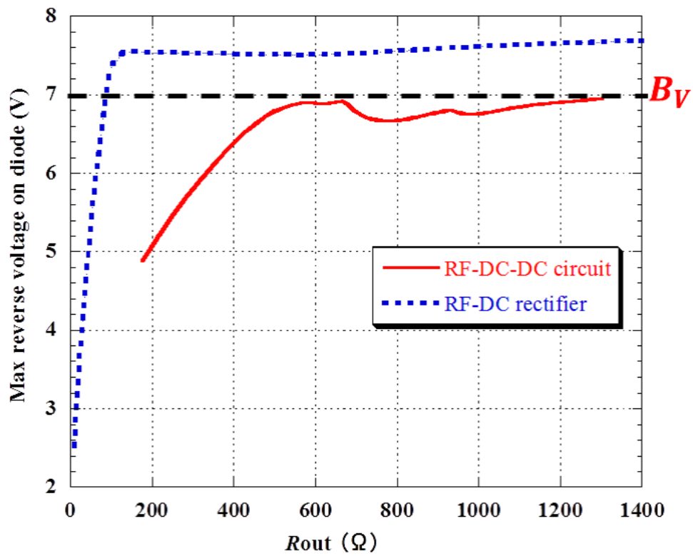
Figure 2.13: Maximum reverse voltage on the rectifying diode ( \text{Max}V_d ) comparison: \text{Max}V_d of the RF-DC-DC circuit is under breakdown voltage (7 V).
