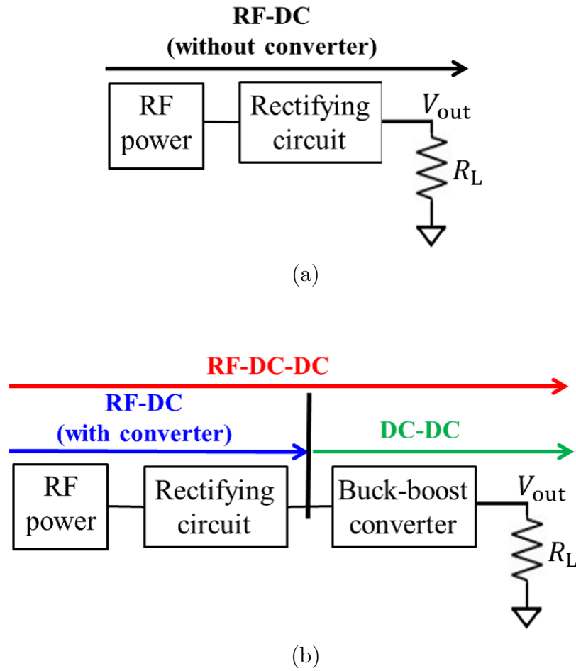
Figure 4.14: Illustration for the efficiency of each part in RF-DC-DC circuit. (a) General rectifier. (b) RF-DC-DC circuit.
