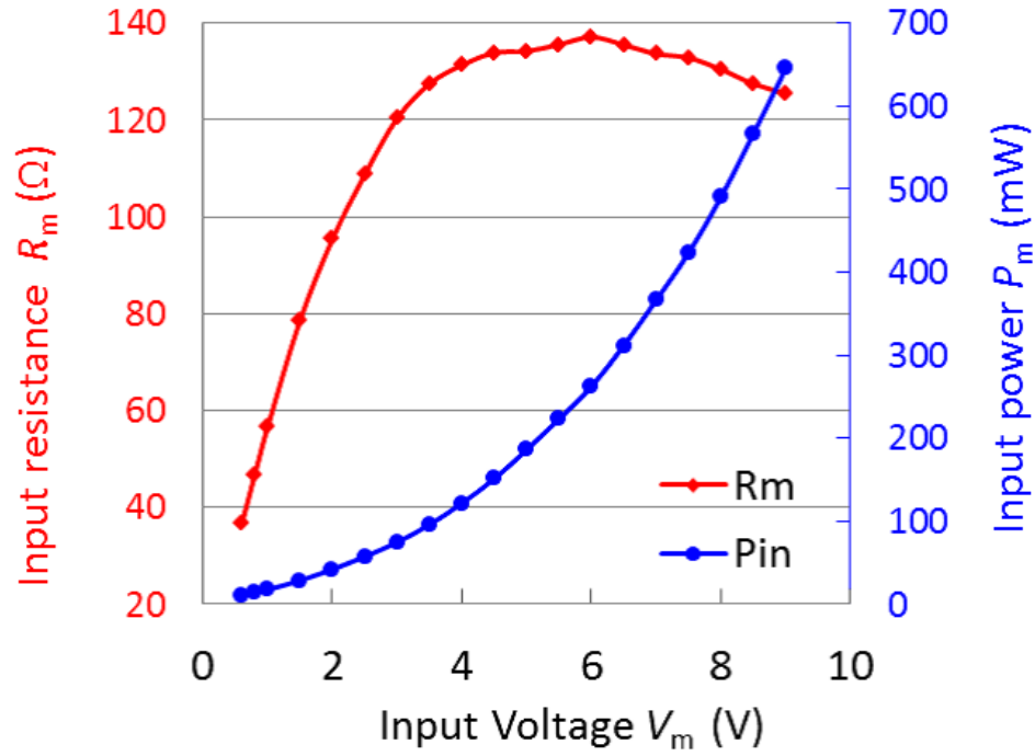
Figure 5.2: Measured input load characteristics of the DC motor.
