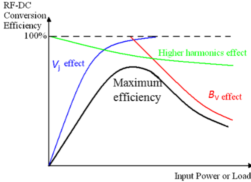
Figure 1.5: Efficiency characteristics of a general rectenna. The efficiency strongly depends on the input power or the load resistance [44].
