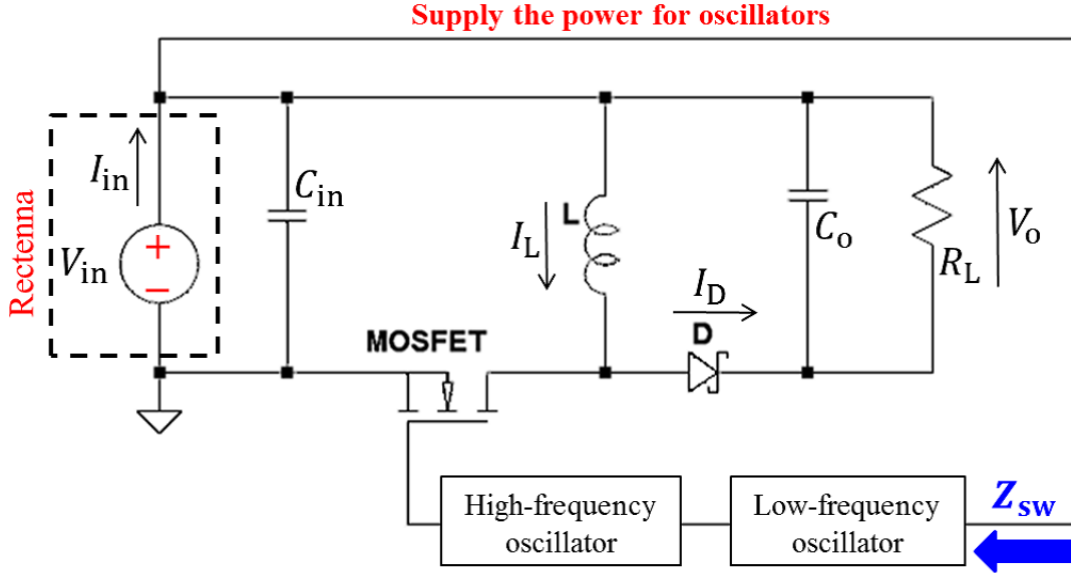
Figure 4.3: Block diagram of the self-powered non-inverting buck-boost converter.
