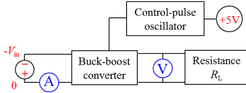
Figure 3.6: Measurement setup of the externally-powered buck-boost converter. An extra +5 V power source is required.
