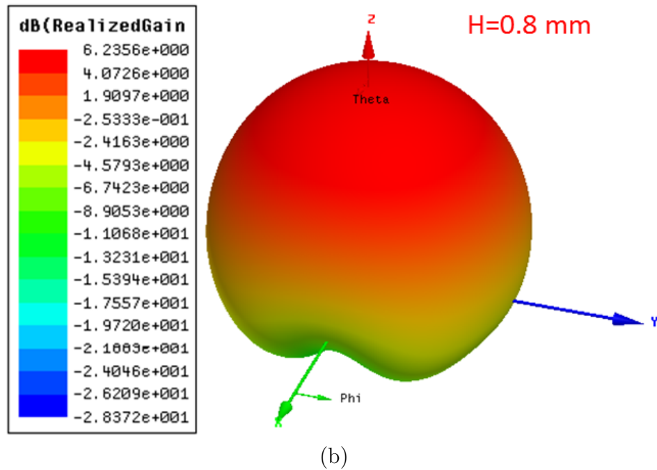
Figure 5.5: Simulated gains of antennas. (a) The gain of H16 antenna is 7.04 dBi. (b) The gain of H08 antenna is 6.24 dBi.
