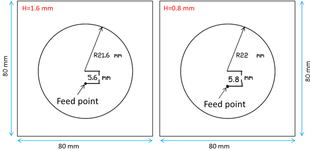
Figure 5.3: Designed antenna sizes.
