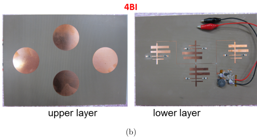
Figure 5.15: Photograph of the compact rectenna array and buck-boost converter. (a) 9AO power-receiving device. (b) 4BI power-receiving device.
