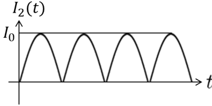
Figure A.4: Current waveform of I_2 .
