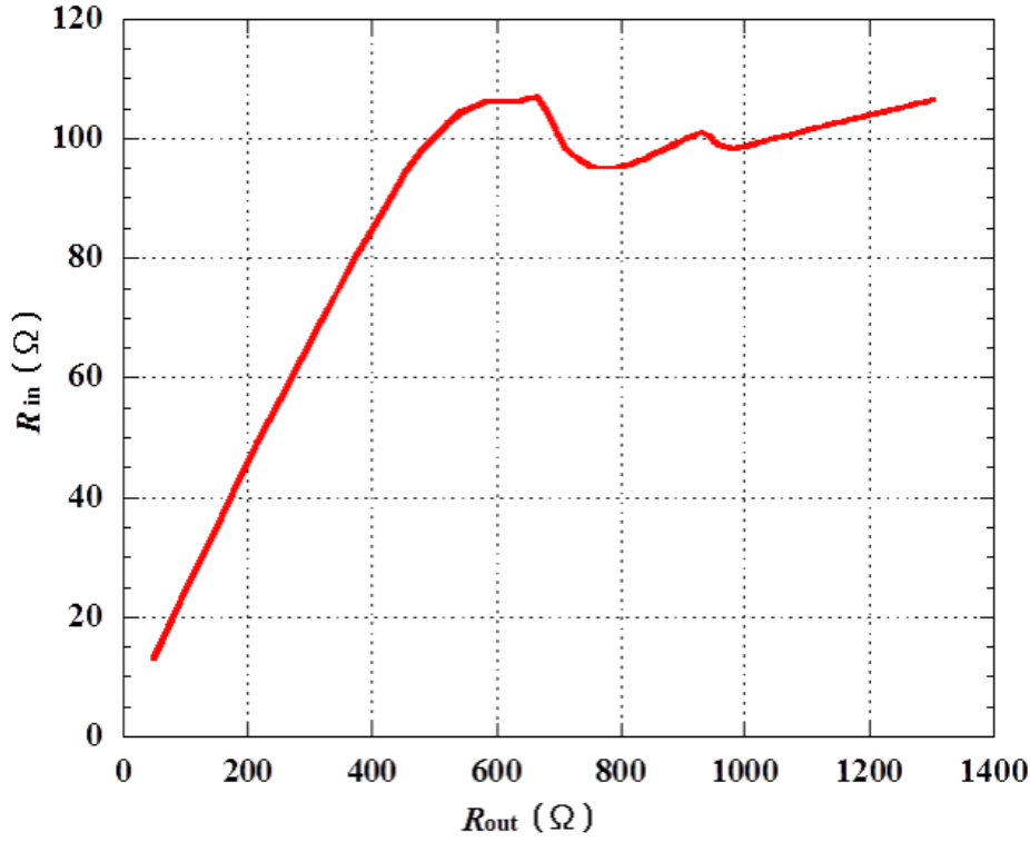
Figure 2.8: Simulation results of the boost converter such as the input resistance ( R_{in} ) vs. load resistance.
