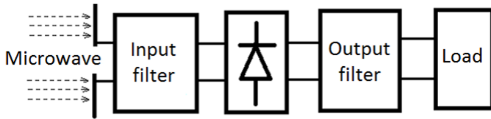
Figure A.1: Block diagram of a general rectenna. It usually contains an antenna, an input filter, a rectifying component, an output filter and a load.
