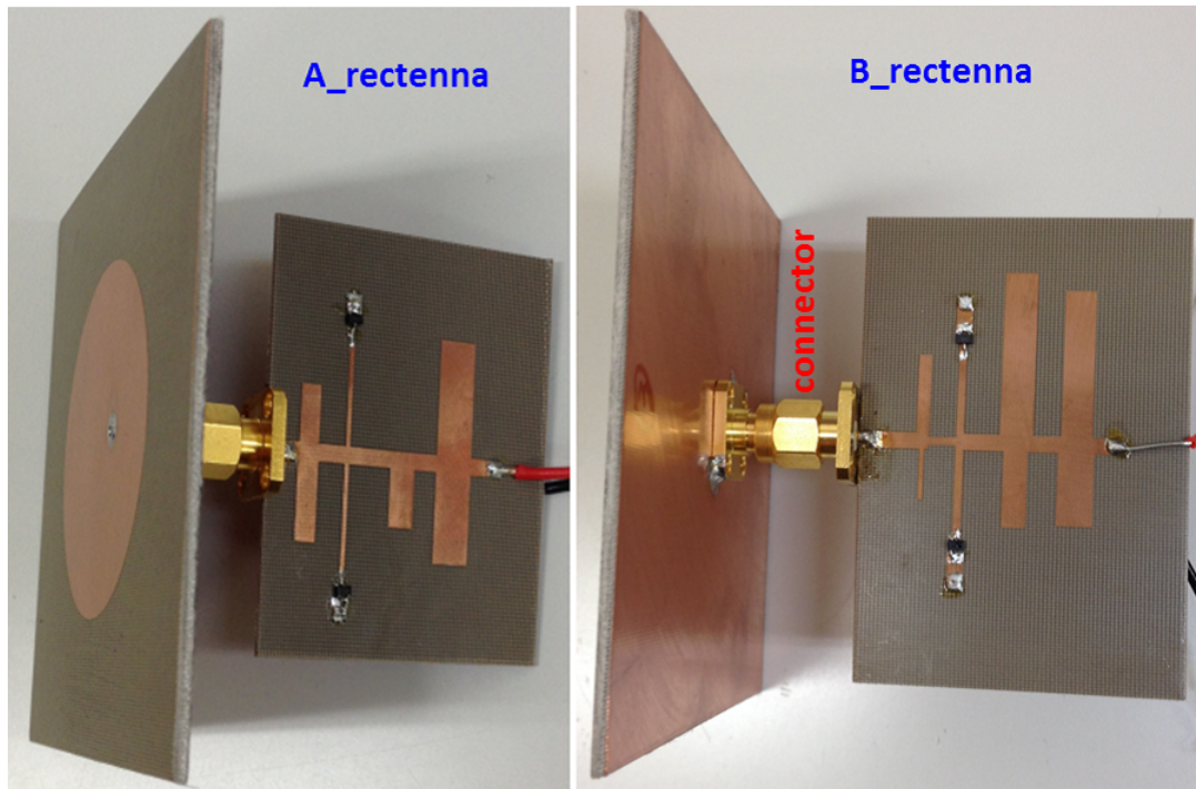
Figure 5.13: Photograph of a single A rectenna and B rectenna.
