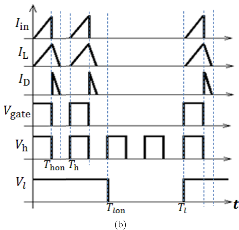
Figure 3.4: Inverting DCM buck-boost converter. An extra +5 V power source is required for the control-pulse circuit. Input a negative voltage to obtain a positive output voltage. (a) Structure. (b) Operating waveforms.
