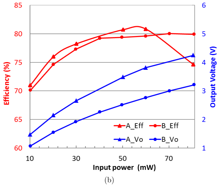
Figure 5.9: Comparison of the measured efficiency and the output voltage. (a) Efficiency and output voltage vs. load for a fixed input power of 50 mW. (b) Efficiency and output voltage vs. input power for the optimal load of 300 \Omega (rectifier A) and 160 \Omega (rectifier B), respectively. A_Eff, A_Vo are the efficiency and output voltage of the rectifier A; B_Eff, B_Vo are the efficiency and output voltage of the rectifier B.
