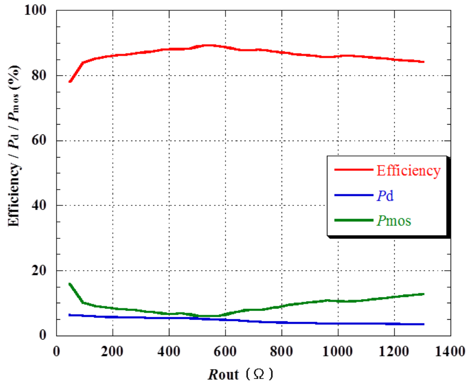
Figure 2.7: Simulation results of the boost converter such as Efficiency, MOSFET loss ( P_{mos} ), diode loss ( P_d ) vs. load resistance.
