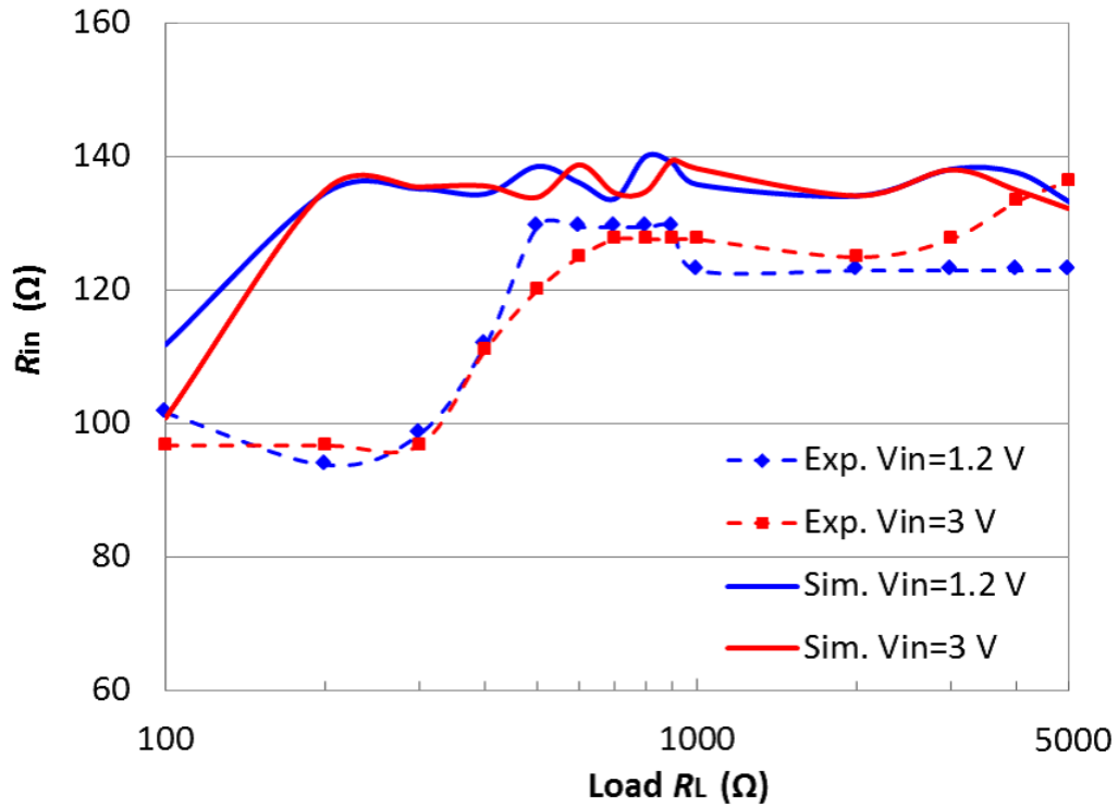
Figure 3.7: Simulation and experimental results of the input resistance R_{in} vs. load resistance for an input voltage of 1.2 or 3 V.
