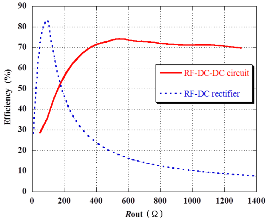
Figure 2.11: Efficiency comparison of the RF-DC-DC circuit and general rectifier.
