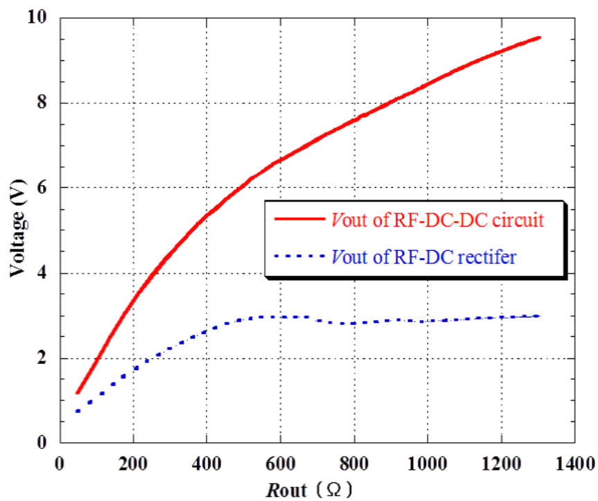
Figure 2.14: Output voltage of the RF-DC-DC circuit and the voltage at the output port of RF-DC rectifier.
