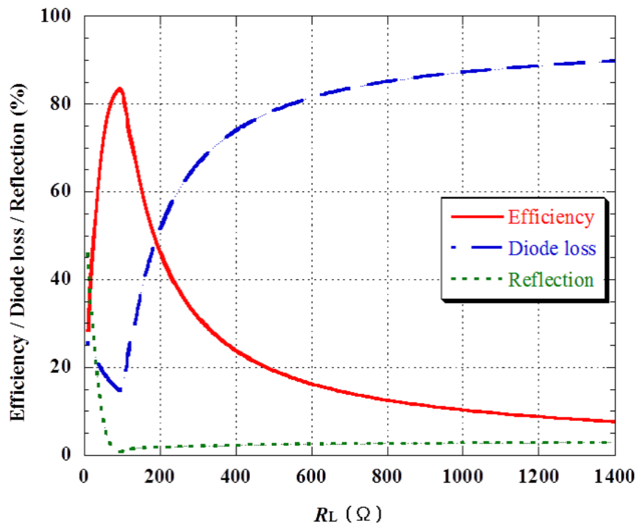
Figure 2.4: Efficiency, diode loss, reflection vs. load resistance of the 6D rectifier (two HSMS286L diode branches).
