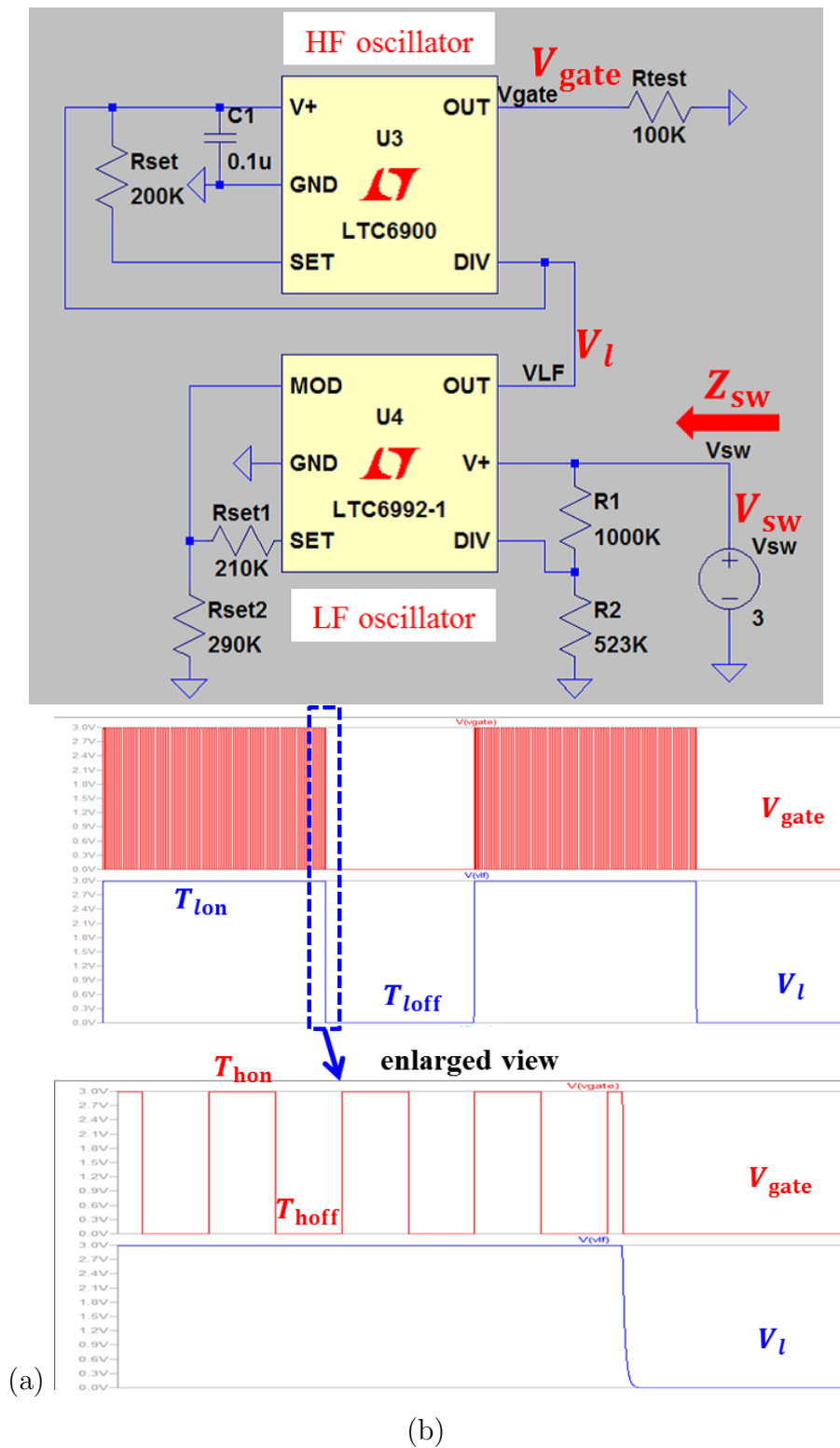
Figure 4.4: Control-pulse circuit of the buck-boost converter in simulation (LT-spice). (a) Simulation circuit: LTC6992 is the LF oscillator; LTC6900 is the HF oscillator. (b) Simulated waveforms.
