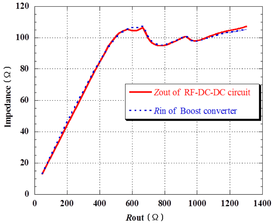
Figure 2.12: Impedance comparison: Z_{out} of the RF-DC-DC circuit is almost the same as R_{in} of the boost converter.
