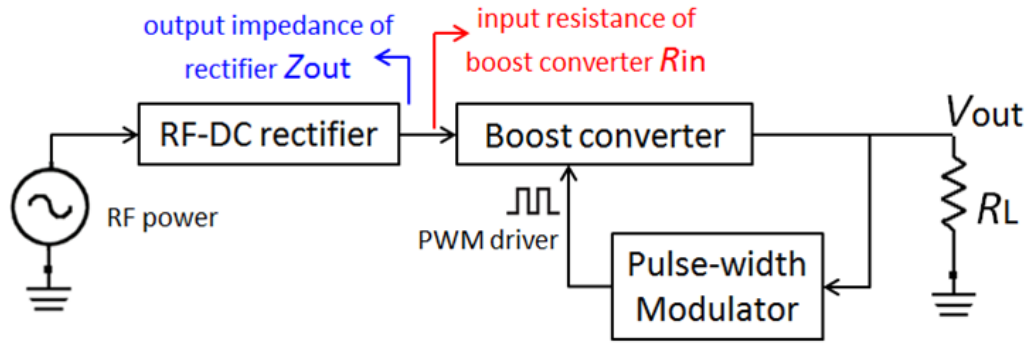
Figure 2.9: Block diagram of the RF-DC-DC circuit: the boost converter is connected to the RF-DC rectifier.
