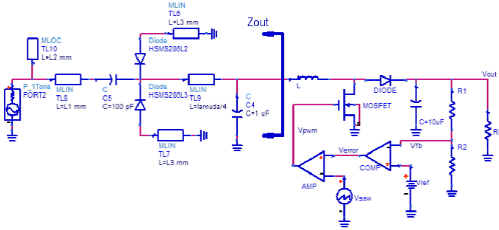
Figure 2.10: Circuit diagram of the RF-DC-DC. Simulate it with two fundamental frequencies of 2.45 GHz and 1.8 MHz using HB analysis in ADS.
