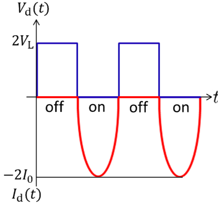
Figure A.5: Voltage and current waveforms of the diode: V_d , I_d .
