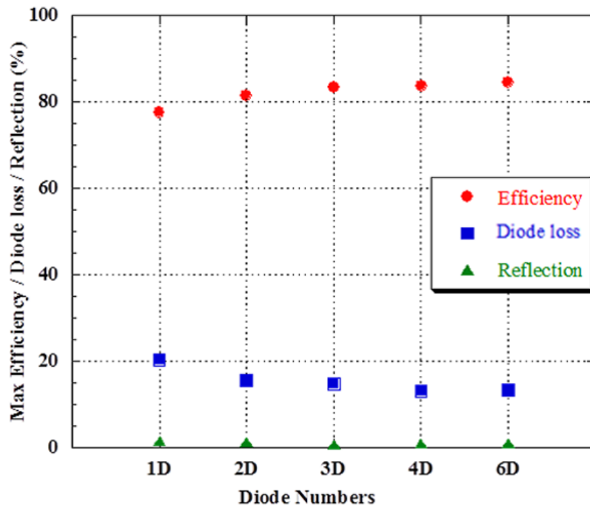
Figure 2.3: Maximum efficiency, diode loss and reflection comparison of five rectifiers.
