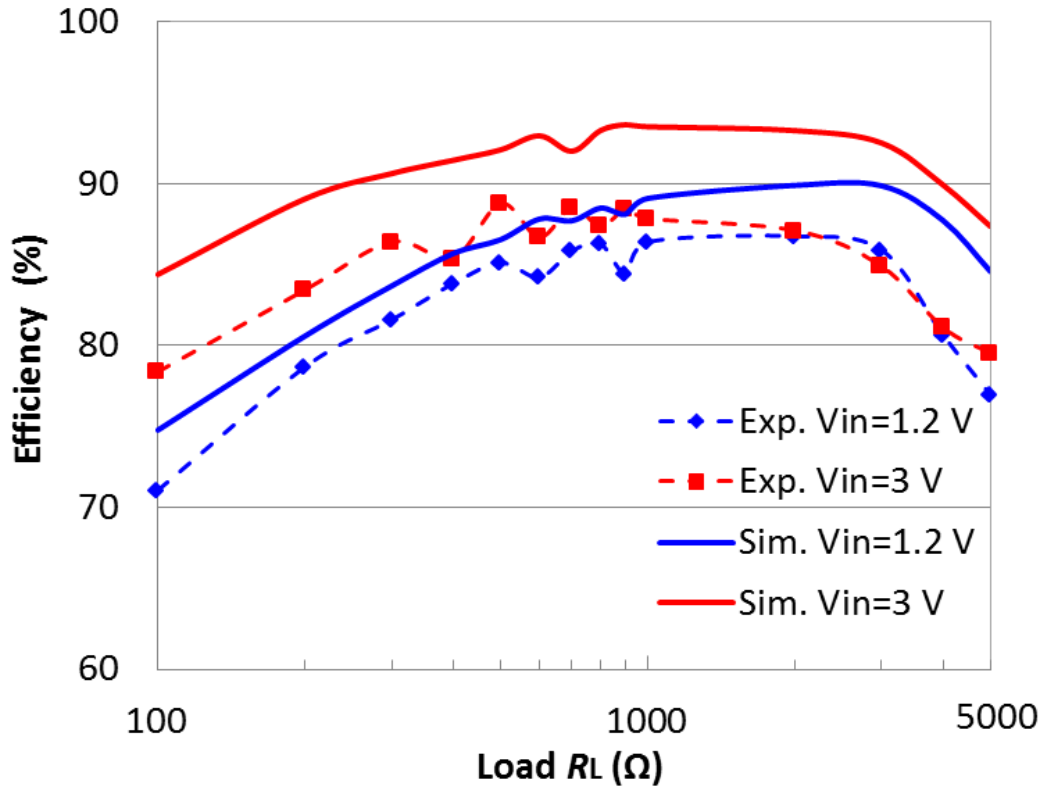
Figure 3.9: Simulation and experimental results of the efficiency vs. load resistance for an input voltage of 1.2 or 3 V.
