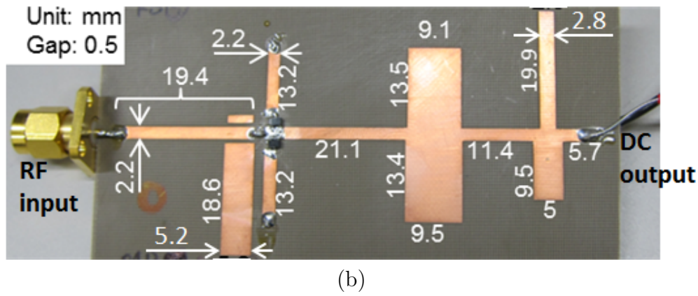
Figure 3.11: Proposed negative output voltage rectifier. (a) Structure. (b) Photograph.
