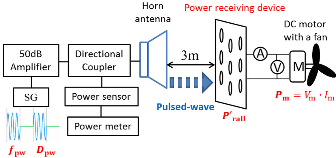
Figure 5.23: Experiment setup for driving DC motor by MPT using pulsed-wave.
