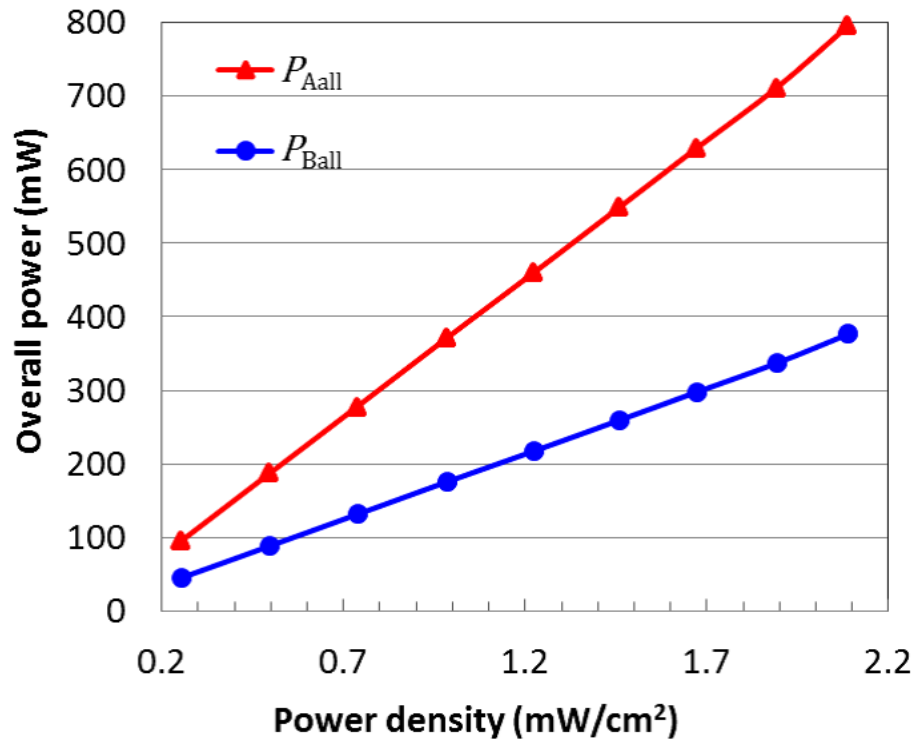
Figure 5.18: Overall powers received by 9 and 4 antennas array such as P_{Aall} and P_{Ball} .
