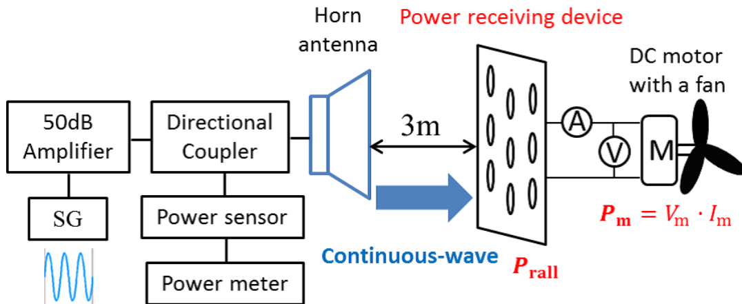
Figure 5.19: Experiment setup for driving DC motor by MPT using CW.
