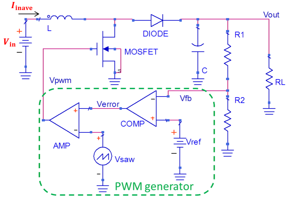
Figure 2.6: Circuit diagram of the simulated DC-DC converter: a PWM controlled boost converter.
