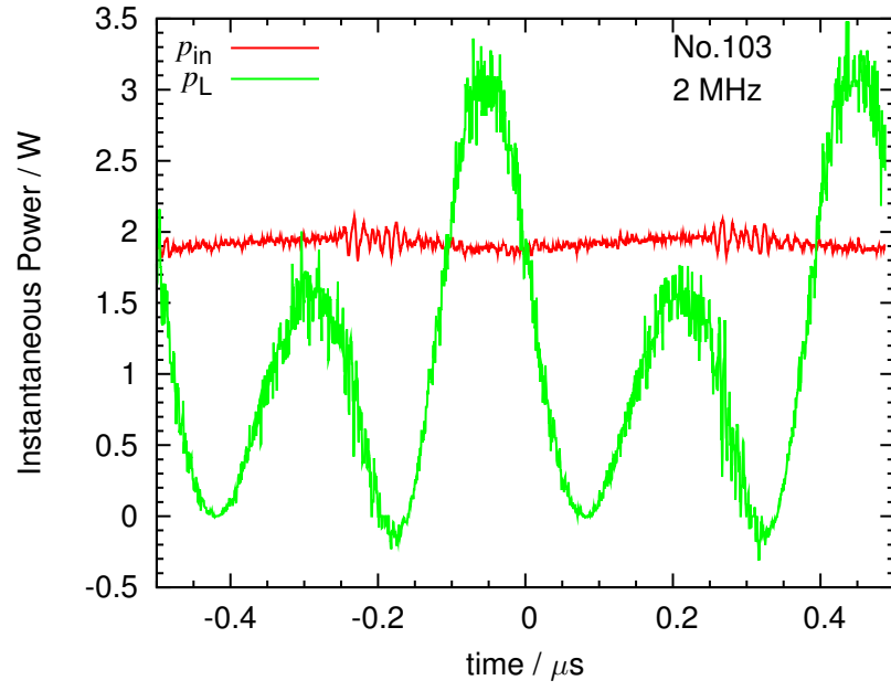
Figure 4.4: Instantaneous power waveforms of input and load. Red line is input power p_{\text{in}} and green is load power p_{\text{L}} .
