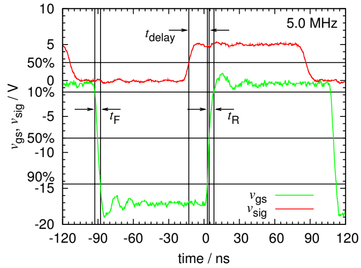
Figure 2.8: Measured waveforms of v_{\text{sig}} (red) and v_{\text{gs}} (green) at 5 MHz.
