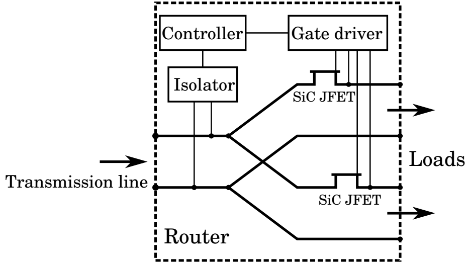
Figure 5.13: Schematic diagram of the router, which has one input terminal and two outputs.
