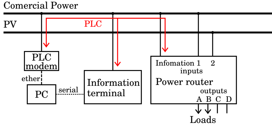
Figure 5.8: Schematic diagram of configuration of experiments. The routing of two inputs by two outputs is examined. The output C and D are not in use during the experiments. The routing rules are configured and programmed in PC in advance. Hence switching order go through the information terminal.
