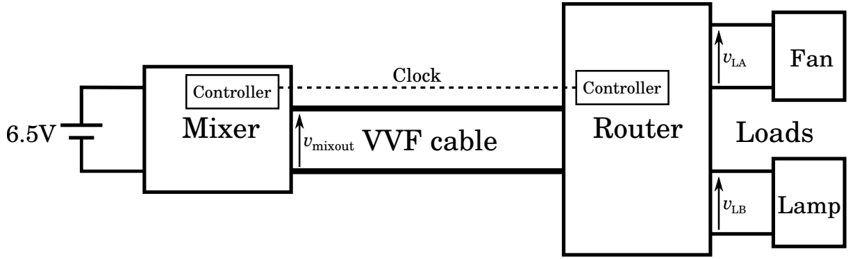
Figure 5.14: Experimental configuration of dc packet dispatching system.
