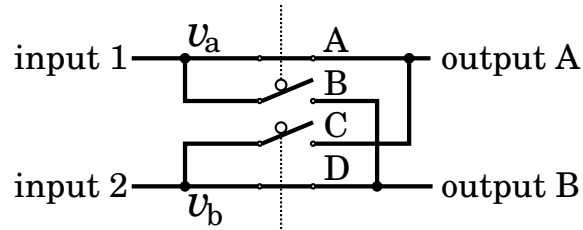
Figure 5.6: Schematic diagram of circuit exchange switches. Switch A interlocks switch B and switch C does D. A circle on the switch represents inverted operational logic, which means that switch A is close while switch B is open.
