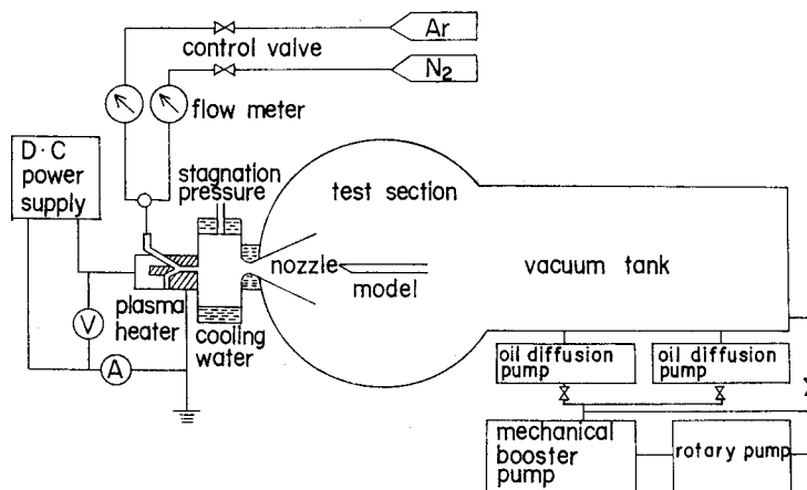
Fig. 2. Schematic of a plasma jet wind tunnel.
