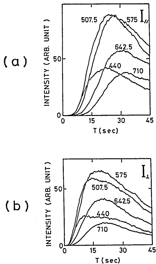
Fig. 4.13 (a) Recorder traces showing the changes of the scattered light intensities I_{\parallel} at five wavelengths, obtained in the experiment J5 (the \text{Ar}^+ laser: 50 mW and 15 mm i.d.; the white light: 5 mm i.d.; the cell temperature: 330^{\circ}\text{C} ). (b) The same as in (a), but for I_{\perp} .
