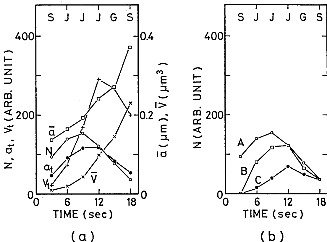
Fig. 4.19 (a) The temporal changes of the number density N (arb. unit), the total radius a_t (arb. unit), the total volume V_t (arb. unit), the mean radius \bar{a} ( \mu\text{m} ), and the mean volume \bar{V} ( \mu\text{m}^3 ), obtained in the experiment J1 (the \text{Ar}^+ laser: 50 mW and 2 mm i.d.; the white light: 10 mm i.d.; the cell temperature: 330^\circ\text{C} ). The symbols G, S, and J indicate the best fit-test functions: G-Gauss, S-Stevenson, and J-Junge distribution functions. (b) The number densities in the size range of 0.1 \mu\text{m} to 1 \mu\text{m} (A), 0.15 \mu\text{m} to 1 \mu\text{m} (B), and 0.2 \mu\text{m} to 1 \mu\text{m} (C) for the experiment J1.
