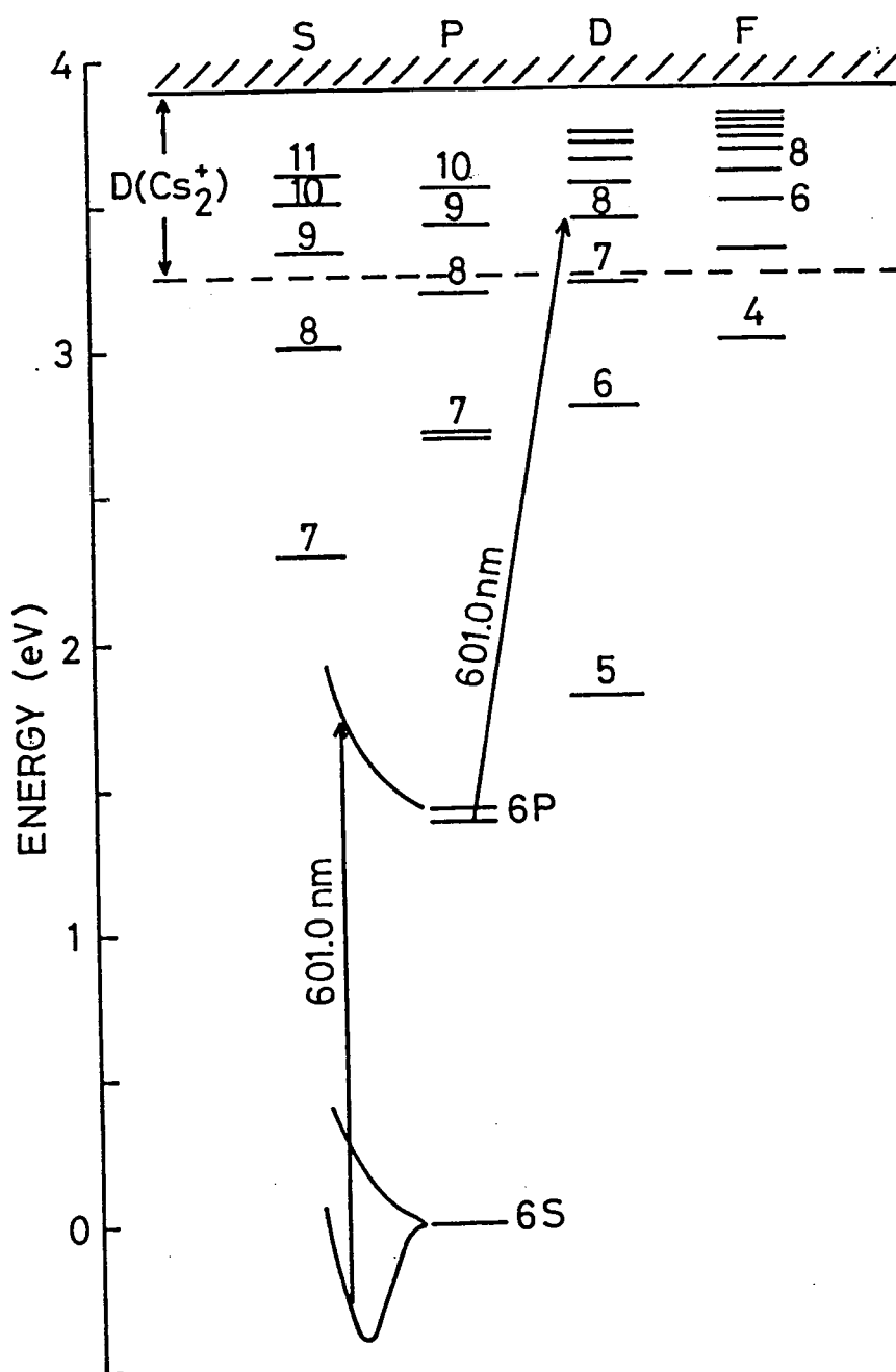
Fig. 3.14 Energy level diagram of Cs. 75) The mechanism of the excitation to the 8D_{3/2} state by the dye laser beam at \lambda = 601.0 \text{ nm} is also shown.
