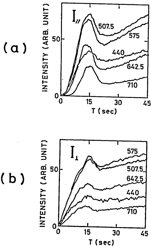
Fig. 4.10 (a) Recorder traces showing the changes of the scattered light intensities I_{//} at five wavelengths, obtained in the experiment J2 (the \text{Ar}^+ laser: 50 mW and 0.2 mm i.d.; the white light: 10 mm i.d.; the cell temperature: 330°C). (b) The same as in (a), but for I_{\perp} .
