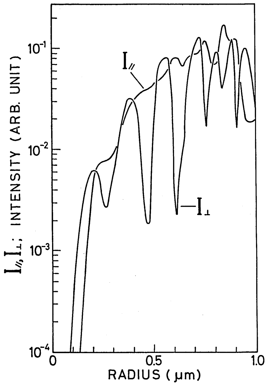
Fig. 4.3 Intensities I_{//}(\lambda, a; \theta) and I_{\perp}(\lambda, a; \theta) as functions of particle radius a in the case that \lambda = 642.5 nm, \theta = 85^\circ , and \hat{n} = 1.48 .
