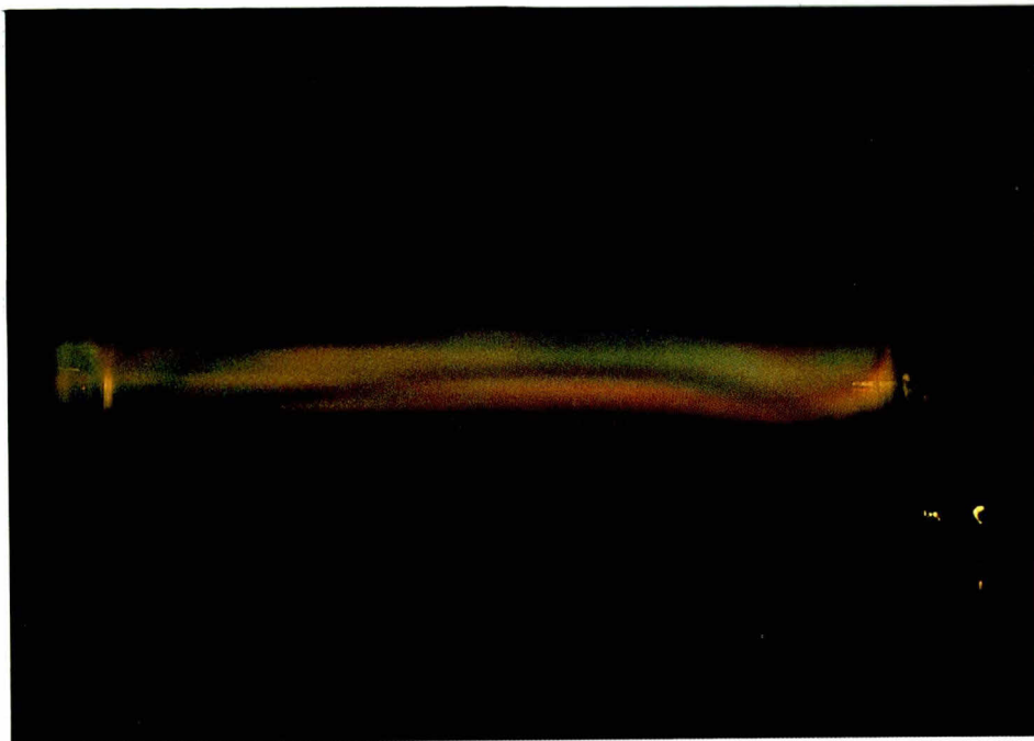
Fig. 3.20 A photograph of the white light scattering by CsH laser snow produced by the \text{Ar}^+ laser 457.9 nm line. The white light beam diameter was about 10 mm and the \text{Ar}^+ laser beam diameter was about 15 mm. The cell temperature was 334°C and the \text{Ar}^+ laser power was 210 mW. In this figure, we can see both the stripes of the scattered light intensity and the changes of color or wavelength. This means that there are spatial distributions of both the particle density and the particle size. (See pages 75 and 134.)
