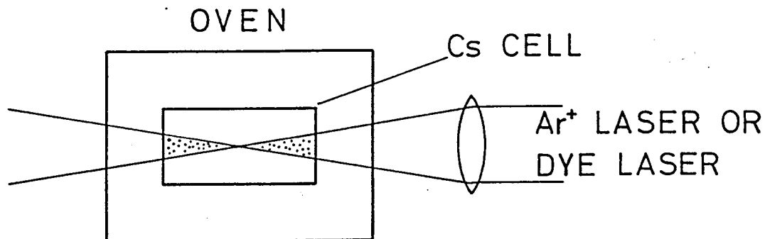
Fig. 3.17 Experimental setup of CsH laser snow formation.
