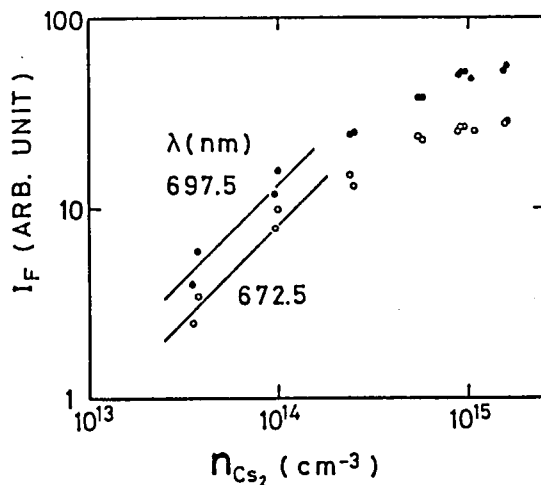
Fig. 3.16 The intensities of Cs atomic fluorescence ( I_F ) at 672.5 nm ( 6P_{1/2} + 7D_{3/2} ) and 697.5 nm ( 6P_{3/2} + 7D_{5/2} ) vs. the densities of (a) Cs and (b) Cs_2 . In the low density region, the fluorescence shows (a) the quadratic dependence on the density of Cs and (b) the linear dependence on the density of Cs_2 . But, in the high density region, the fluorescence becomes insensitive to the change of the densities of Cs and Cs_2 .
