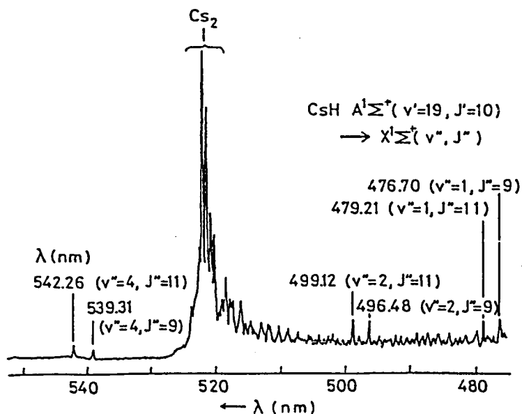
Fig. 3.22 Observed laser-induced fluorescence of CsH and Cs 2 excited by the Ar + laser 457.9 nm line at 200 mW. The cell C-1 (P H 2 = 27 Torr) was used and the cell temperature was 360°C.
