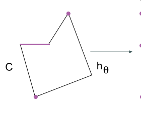
Figure 2: Singular points (bold) of h_\theta|C
