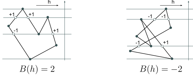
Figure 4: Sample computations of B(h)
