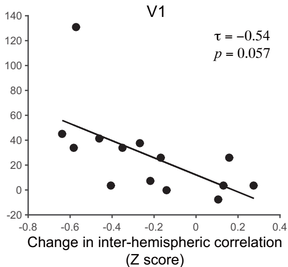
Figure 7. The relationship between inter-hemispheric correlation and SSQ score. A scatter plot of the change in inter-hemispheric correlation vs. change in SSQ total score for each subject between the local and global motion conditions (global - local). Each point represents the data of one subject ( n = 14 ). Kendall's correlation coefficient ( \tau ) and Bonferroni-corrected p value are shown. (a) for MT+ and (b) for V1.
