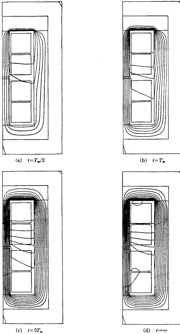
Fig. 15. Flux distributions for T_m = 0.051 s, \sigma_r = 1 \text{ MS/m} and \Delta A_{st} = 0.5 \text{ mWb/m} .
