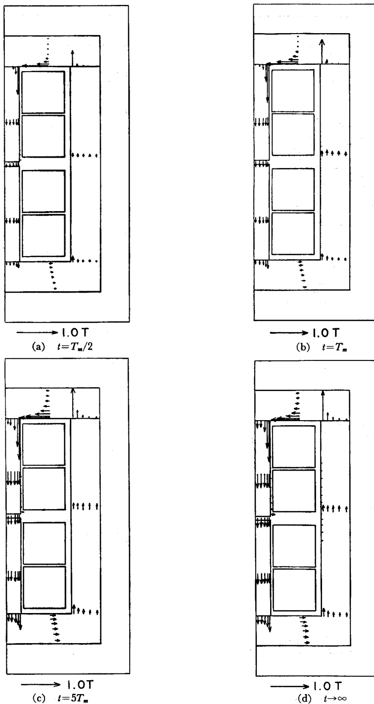
Fig. 16. Distributions of magnetic flux density for T_m = 0.051 s and \sigma_s = 1 MS/m.
