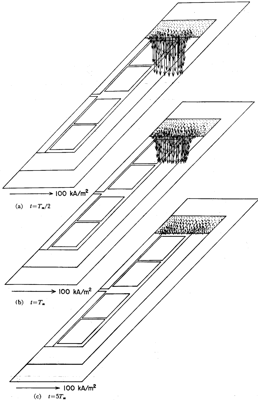
Fig. 17. Distributions of induced eddy current for T_m = 0.051 \text{ s} and \sigma_y = 1 \text{ MS/m} .
