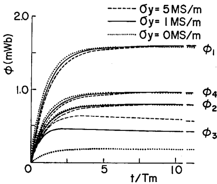
Fig. 19. Influence of \sigma_y on transient response of magnetic flux.
