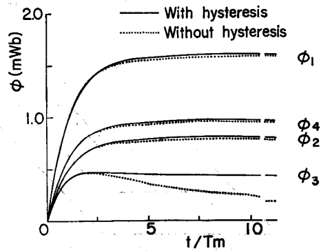
Fig. 20. Influence of magnetic hysteresis on transient response of magnetic flux.
