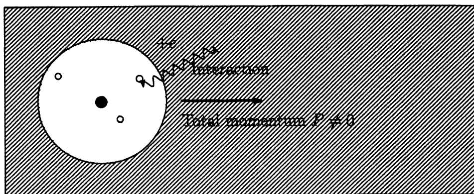
Moving ion in QED
