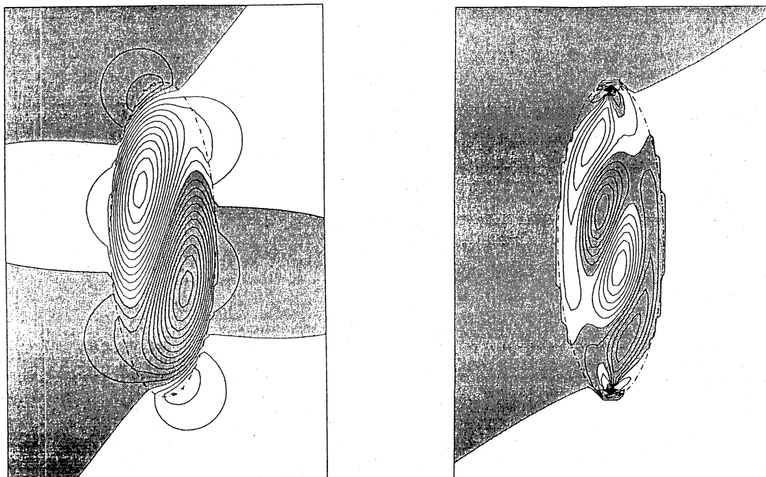
Fig.2a,b Axial velocity distributions in the x-y plane of a) the lowest eigenmode k=0.42 and b) the second eigenmode k=1.0 , for a/b=3 . The contour interval is arbitrary.
