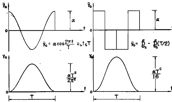
(a) Versed-sine Pulse
