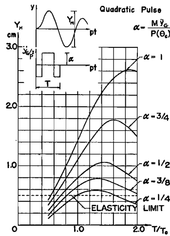
Fig. 11 Period-Amplitude Responses or Spectra of Maximum Distortion for the Full-cycle Quadratic Pulse.
