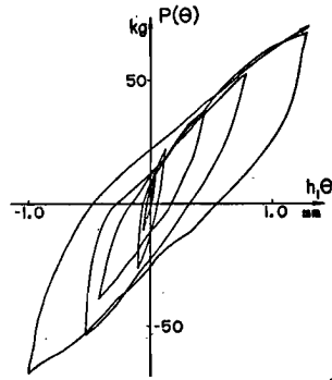
Fig. 5 Load-Distortion Hysteresis Curve of a Bridge Pier Model.
