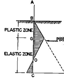
Fig. 2 Idealized Distribution of Reaction of the Ground.
