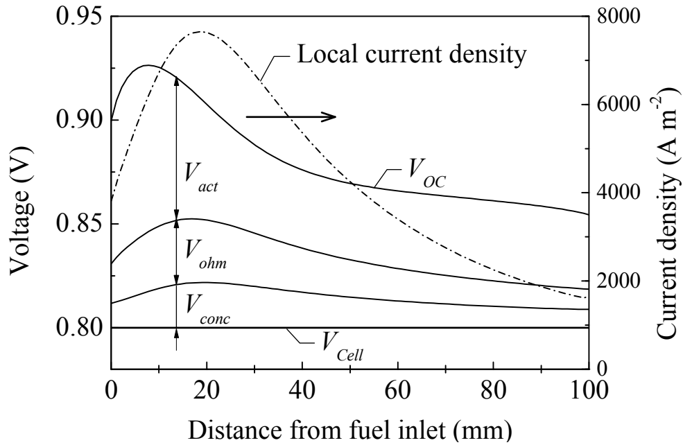
Fig. 4-6: Open-circuit voltage, polarization terms and local current density distributions, counter-flow operation.
