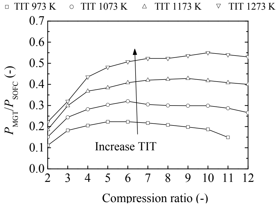
Fig. 6-11: Influence of compression ratio and TIT on P_{\text{MGT}}/P_{\text{SOFC}} .
