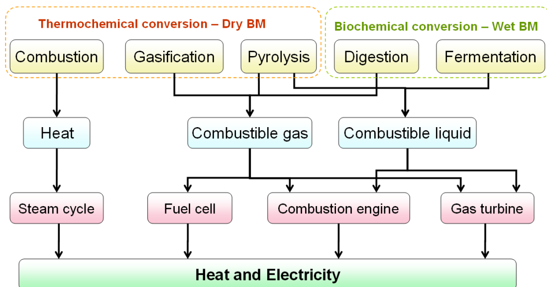
Fig. 2-3: Ways from biomass to electricity.
