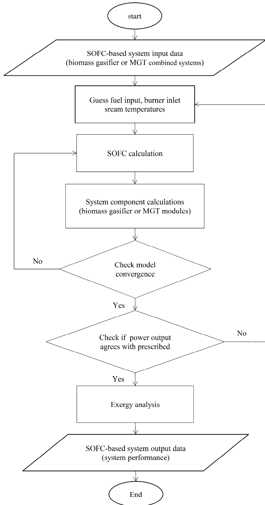
Fig. 3-7: Computational flowchart of SOFC-based system modeling.
