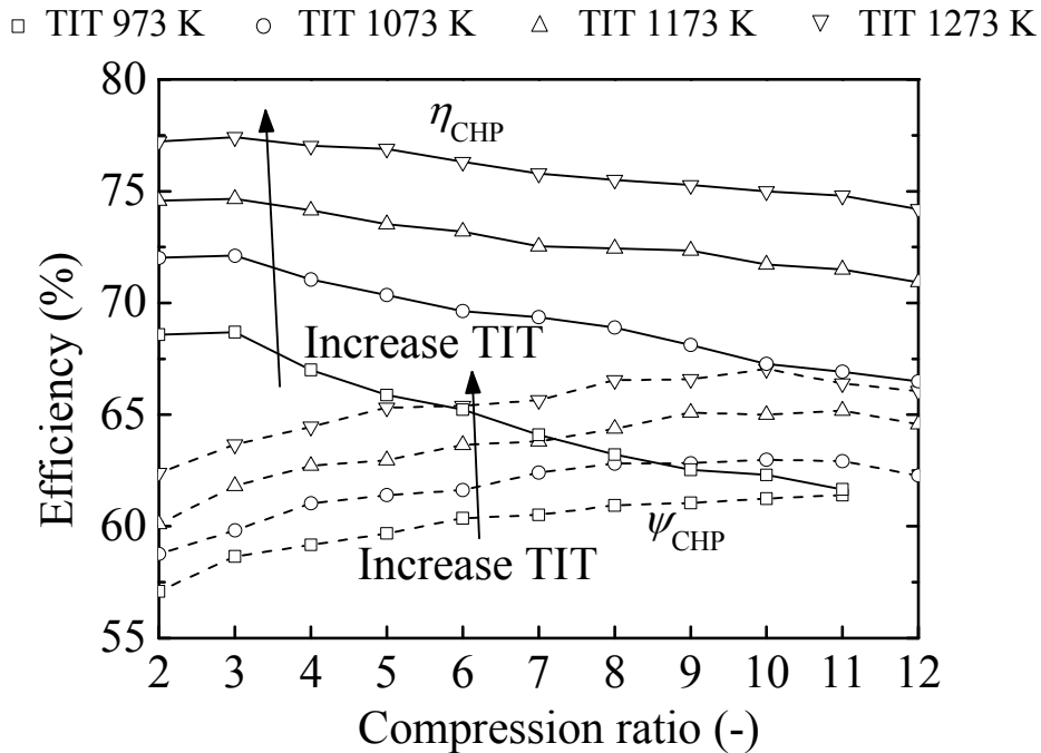
Fig. 6-8: \eta_{CHP} and \psi_{CHP} versus compression ratio and TER.
