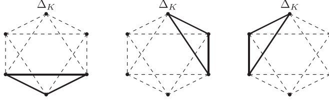
FIGURE 13. Three (same) classes in H^4(Q_4) .
