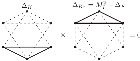
FIGURE 14. \Delta_K(M_I^2 - \Delta_K) = 0 .
