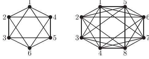
FIGURE 1. The graph induced from the T^3 -action on Q_4 (left) and the T^4 -action on Q_6 (right).
