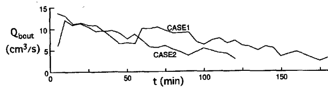
Fig. 14 Temporal variation in the sediment discharge at the by-pass tunnel
