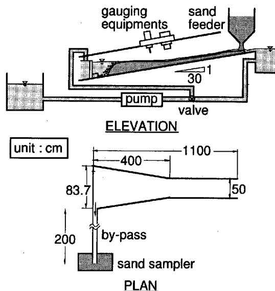
Fig. 2 Experimental flume
