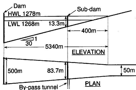
Fig. 1 Configuration of Takase reservoir
