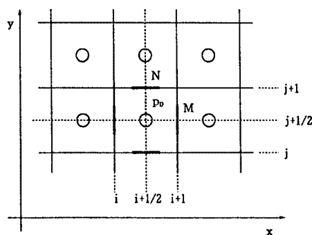
Fig. 5. Control volume for derivation of Eq. (11).
