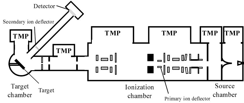
Figure 3.2: The experimental setup for size-selected SIMS
