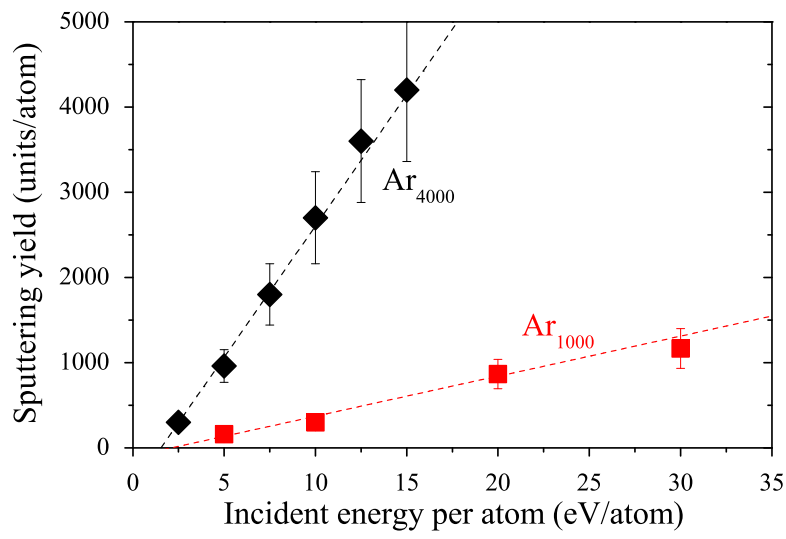
Figure 2.23: Variation in PMMA sputtering yield with varying energy per atom for \text{Ar}_{1000} and \text{Ar}_{4000} clusters.
