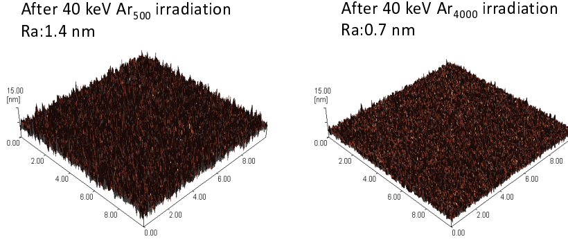
Figure 5.1: AFM images of a Si surface (a) after 40 keV \text{Ar}_{500} and (b) \text{Ar}_{4000} irradiation
