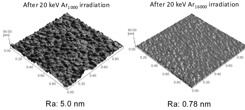
Figure 5.8: AFM images of the PMMA films after 20 keV GCIB irradiation with (a) Ar 1000 , with the dose of 5 \times 10^{13} ions/cm 2 ; (b) Ar 16000 ; with the dose of 1 \times 10^{14} ions/cm 2 . (Scanned area is 1 \mu\text{m} \times 1 \mu\text{m} )
