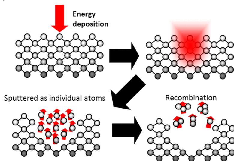
(b) Recombination model
