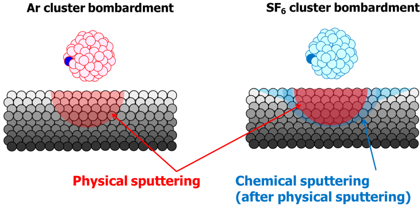
Figure 5.6: The model of sputtering for non-reactive(Ar) and reactive( \text{SF}_6 ) cluster bombardment
