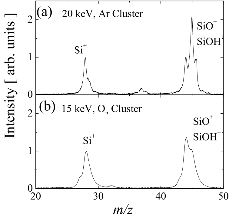
Figure 4.3: Secondary ion spectra of the Si target after oxidation obtained under irradiation with (a) 20 keV Ar cluster ion irradiation in O_2 atmosphere at 6.5 \times 10^{-3} Pa, and (b) 15 keV O_2 cluster ion.
