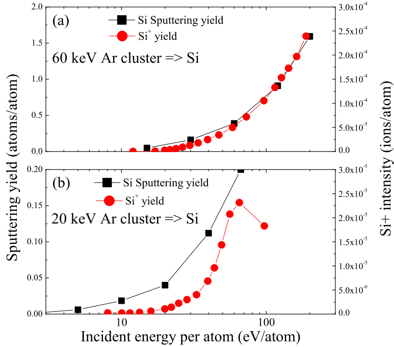
Figure 3.14: Variation of Si and \text{Si}^+ yield with incident energy per atom and cluster size for size-selected 20 and 60 keV Ar cluster ion beams.
