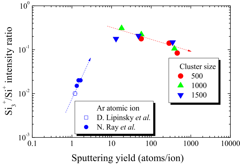
Figure 3.10: The effect of incident energy per atom on the intensity ratio \text{Si}_3^+/\text{Si}^+
