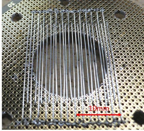
Figure 3.4: The secondary ion deflector
