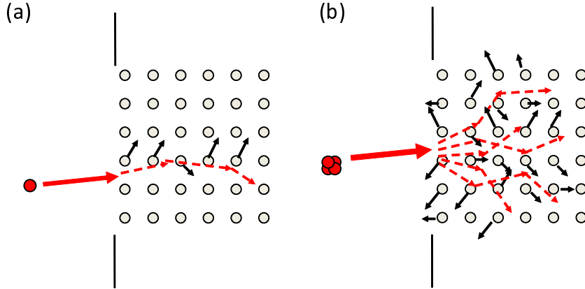
Figure 2.1: Irradiation effect with (a) atomic and (b) cluster bombardment
