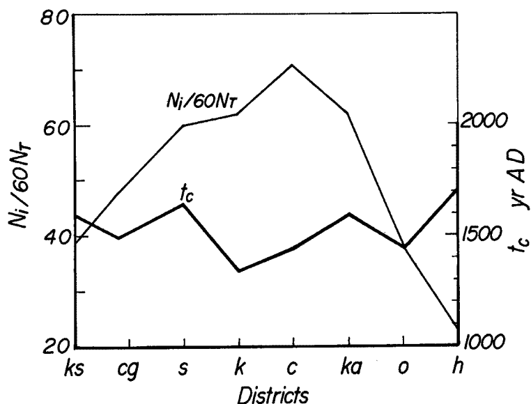
Fig. 40. Locality of typhoon disasters in terms of number of typhoons and their occurrence years.
