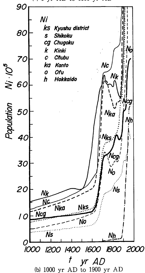
Fig. 25. Changes in population in eight districts since 0 yr AD.
