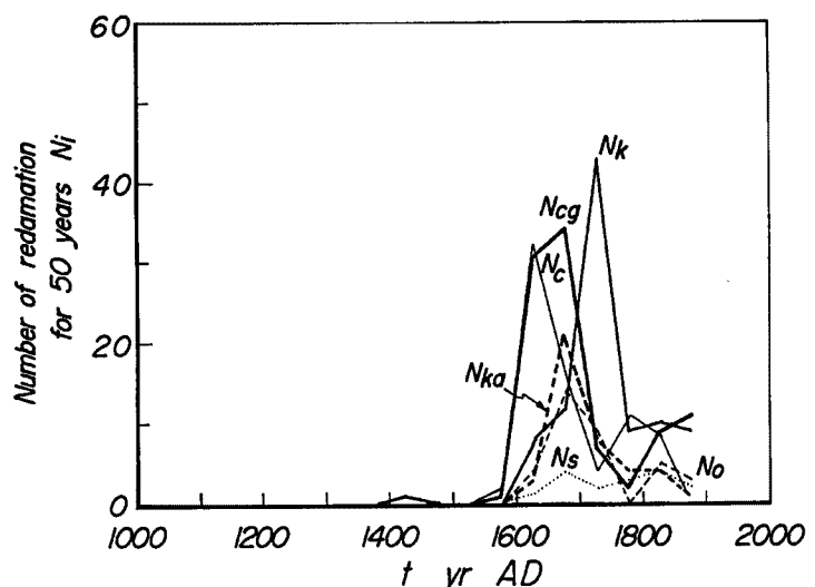
Fig. 33. Changes in number of reclamation for 50 years in eight districts.
