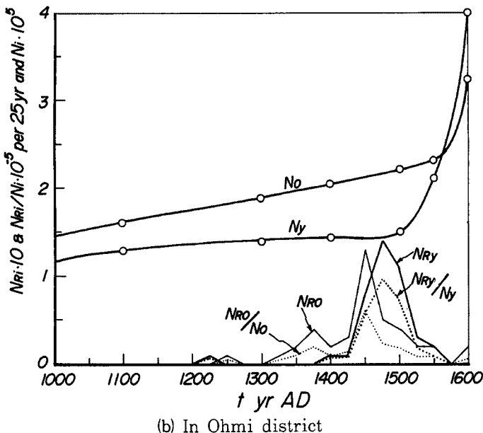
Fig. 51. Changes in population in relation to occurrence of riots in Yamashiro N_{Ry} and Ohmi N_{Ro} , and their population ratios, N_{Ry}/N_y and N_{Ro}/N_o in relation to number of typhoon N_{Dt} , heavy rainfall N_{Dr} and drought N_{Dd} disasters.
