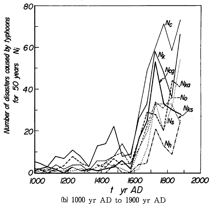
Fig. 37. Changes in number of typhoon disasters taken place for 50 years in the periods specified.
