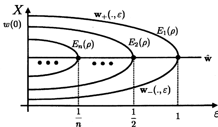
Figure 1. Global bifurcation structure.
