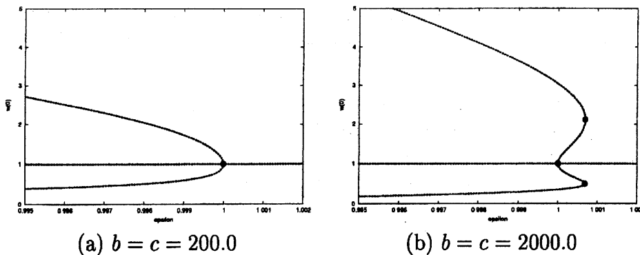
Figure 2. Bifurcation structure, where n = 1.1 and d_w = d_z .
