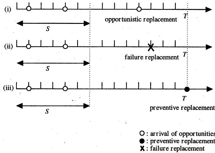
Figure 1: Configuration of the model.
