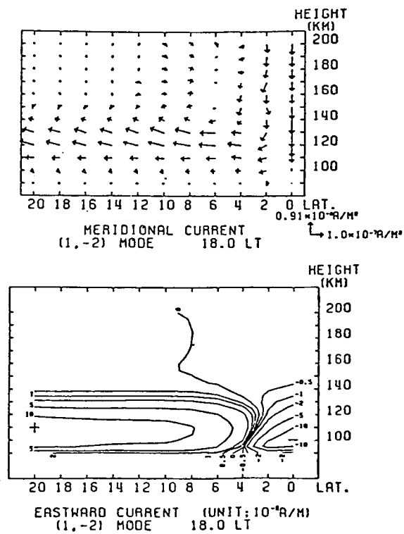
Fig. 10. Same as in Fig. 7 but at 1800 LT.
