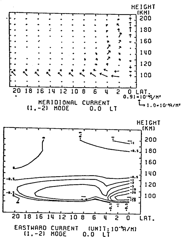
Fig. 7. Meridional current structure (top) and eastward current density (bottom) between 0^\circ and 20^\circ in latitude at 0000 LT.
