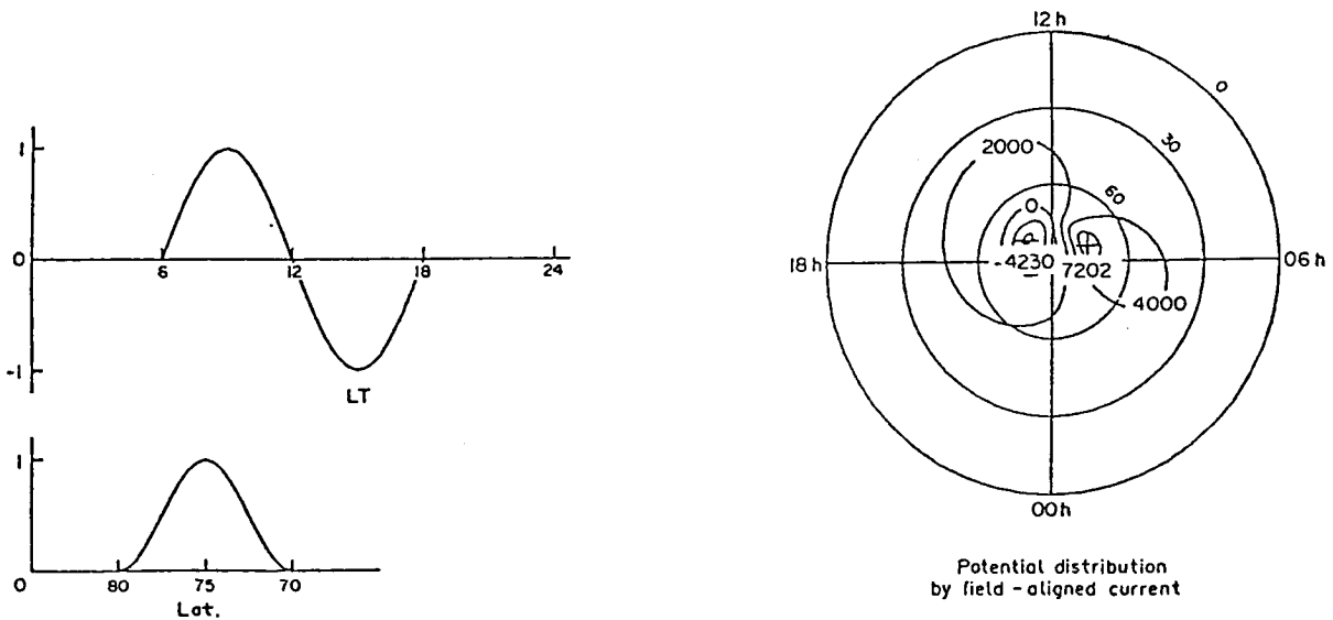
Fig. 31. Electrostatic potential at 90 km. Contours are drawn at every 2000 V. The largest circle represents the equator.
