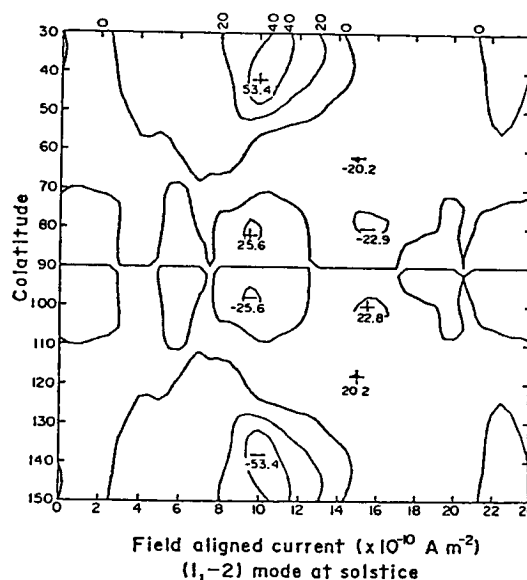
Fig. 28. Distribution of field-aligned currents into the ionosphere at solstice—
