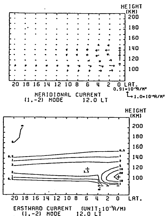
Fig. 9. Same as in Fig. 7 but at 1200 LT
