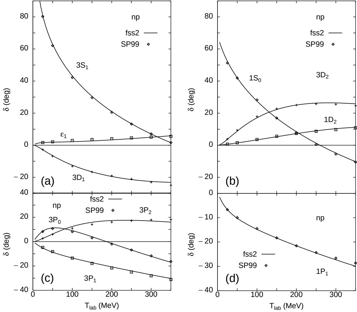
Fig. 1 Calculated np phase shifts (with I \leq 2 ) by fss2 in the isospin basis, compared with the phase-shift analysis SP99 by Arndt et al. [14]
