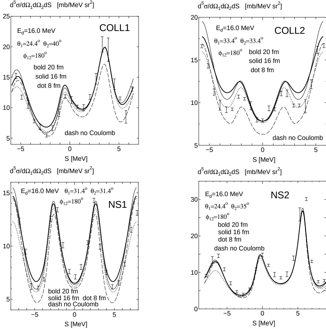
Fig. 14 Breakup differential cross sections for the reaction ^1\text{H}(\vec{d}, 2p)n with E_d = 16 MeV, compared with the experimental data [116]. The cutoff Coulomb radii, \rho = 8 (dotted), 16 (solid) and 20 fm (bold solid curves), together with I_{\text{max}} = 4 are used. No-Coulomb results are shown by the dashed curves.
