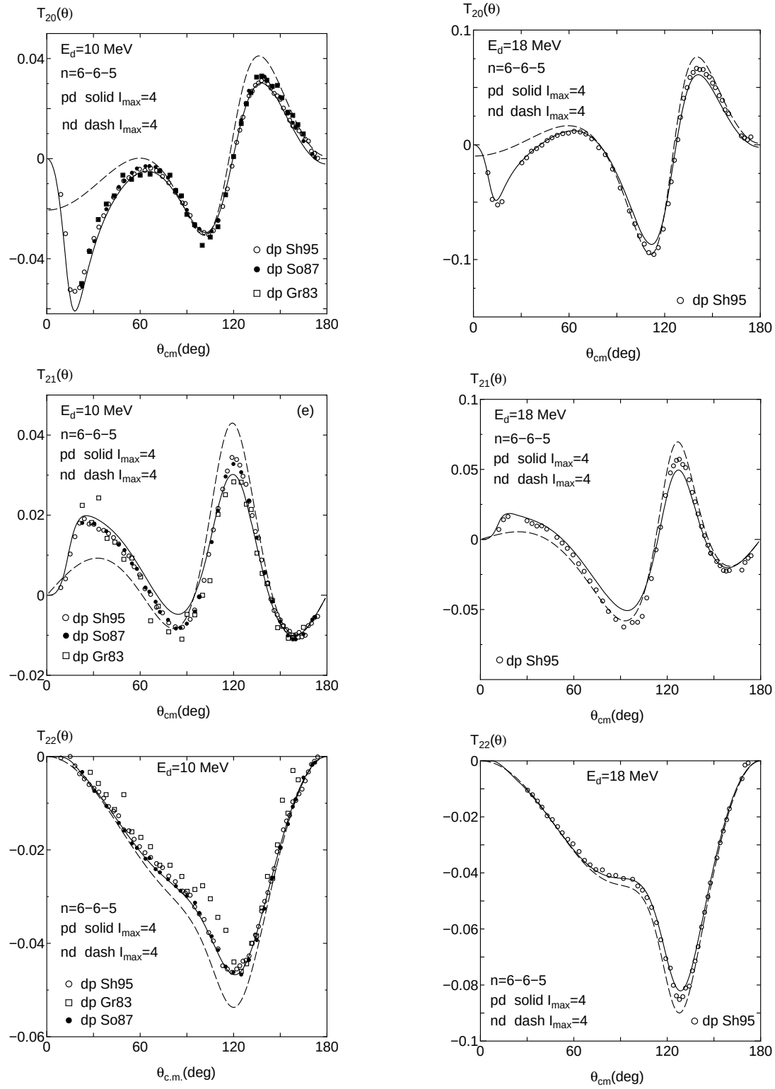
Fig. 11 Tensor-type deuteron analyzing powers iT_{2m}(\theta) with m = 0, 1 and 2 for the nd and pd elastic scattering at E/\text{nucleon} = 5 MeV (left panels) and 9 MeV (right panels), compared with the experimental data. The experimental data are taken from Refs. [86] for Sh95, [107] for So87, and Ref. [76] for Gr83.
