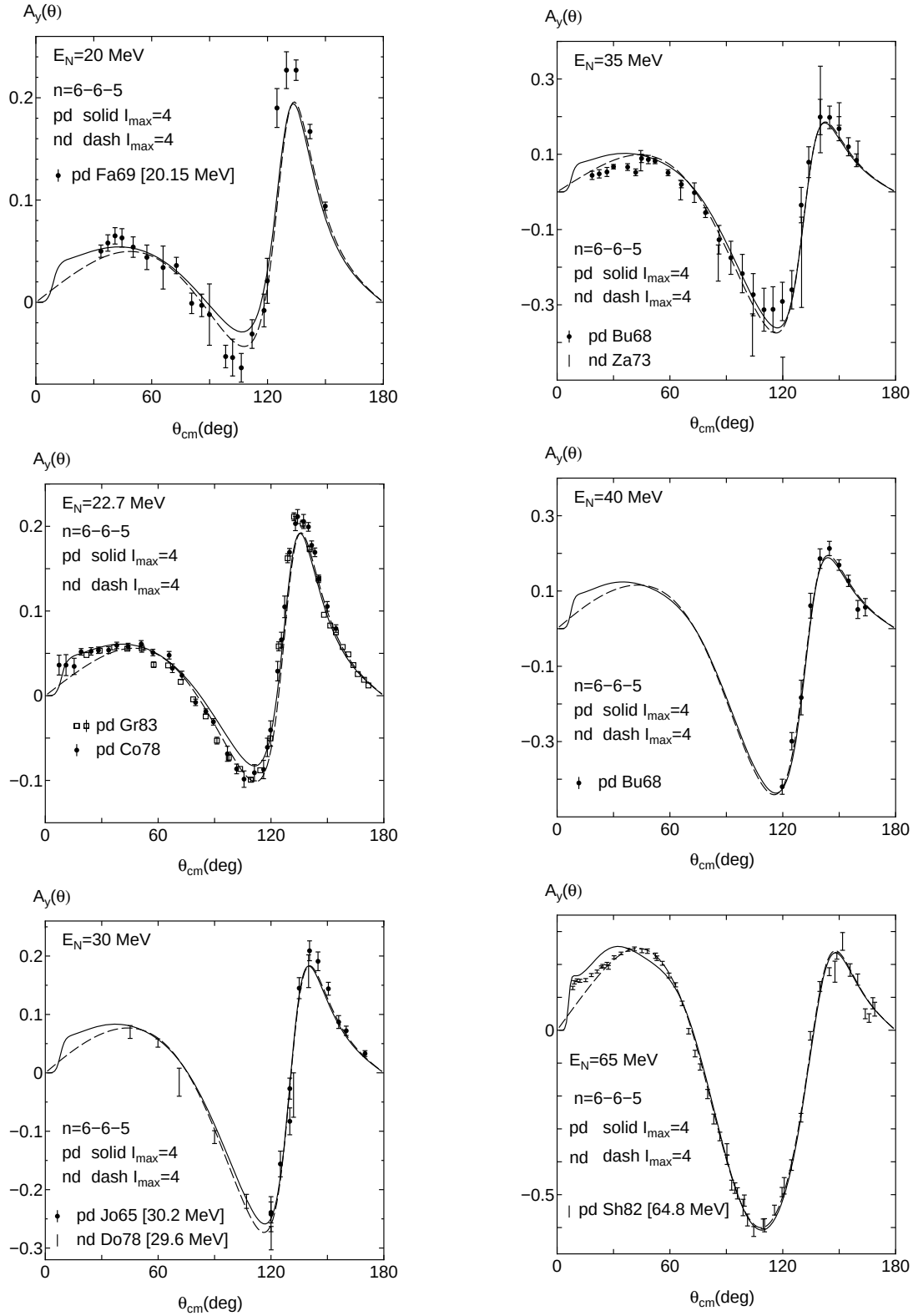
Fig. 9 Nucleon analyzing power A_y(\theta) for the nd and pd elastic scattering from E_N = 20 to 65 MeV, compared with the experimental data. The experimental data are taken from Refs. [97] for Fa69, [98] for Co78, [99] for Jo65, [100] for Do78, [79] for Bu68, [101] for Za73, and Ref. [80] for Sh82. The others are same as in Fig. 8.
