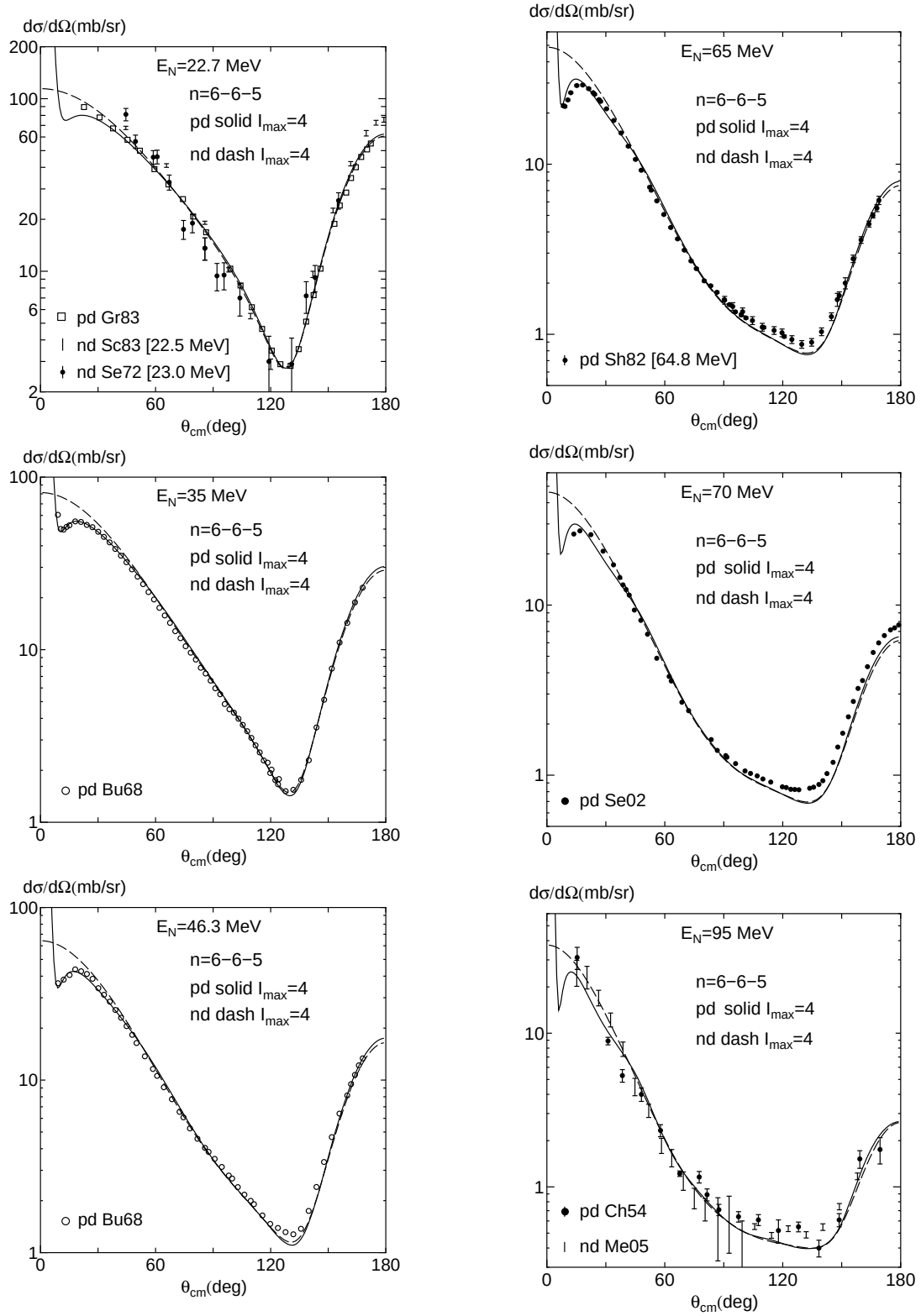
Fig. 6 nd and pd differential cross sections from E_N = 22.7 to 95 MeV, compared with the experimental data. The experimental data are taken from Refs. [56] for Se72, [79] for Bu68, [80] for Sh82, [81] for Se02, [82] for Ch54, and Ref. [83] for Me05. The others are same as in Fig. 5.
