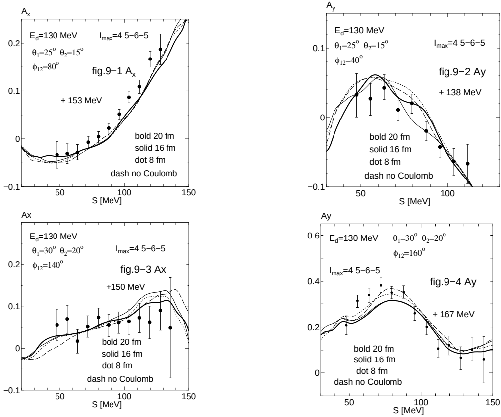
Fig. 16 Vector analyzing power of the deuteron for the reaction ^1\text{H}(\vec{d}, 2p)n with E_d = 130 MeV, compared with the experimental data [119]. The cutoff Coulomb radii, \rho = 8 (dotted), 16 (solid) and 20 fm (bold solid curves), together with I_{\max} = 4 are used. No-Coulomb results are shown by the dashed curves. The calculated curves are shifted by about 150 MeV with respect to S to fit the experimental origin.
