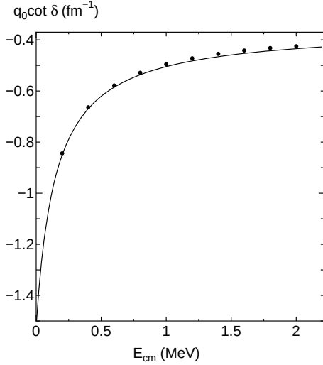
Fig. 2 The effective-range function K(q_0) = q_0 \cot \delta for the doublet S -state as a function of E_{\text{cm}} . The filled circles are the fss2 result and the solid curve shows the approximation by the effective-range parameters in Table 2 with I_{\text{max}} = 4 .
