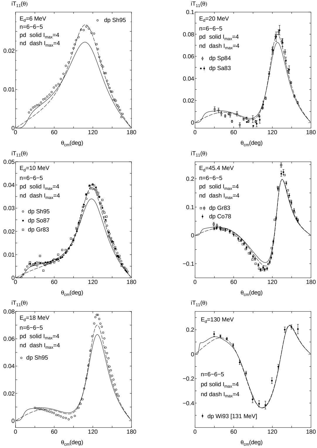
Fig. 10 Vector-type deuteron analyzing power iT_{11}(\theta) for the nd and pd elastic scattering from E/\text{nucleon} = 3 to 65 MeV, compared with the experimental data. The experimental data are taken from Refs. [86] for Sh95, [107] for So87, [76] for Gr83, [77] for Sp84, [104] for Sa83, [98] for Co78, and Ref. [108] for Wi93.
