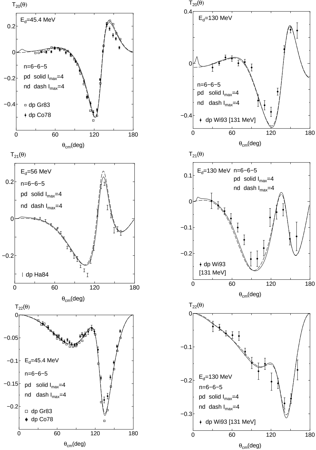
Fig. 12 Same as Fig. 11, but for E/\text{nucleon} = 22.7 MeV ( T_{20}(\theta) and T_{22}(\theta) ) or 28 MeV ( T_{21}(\theta) ) (left panels), and 65 MeV (right panels). The experimental data are taken from Refs. [76] for Gr83, [98] for Co78, [84] for Ha84, and [108] for Wi93.
