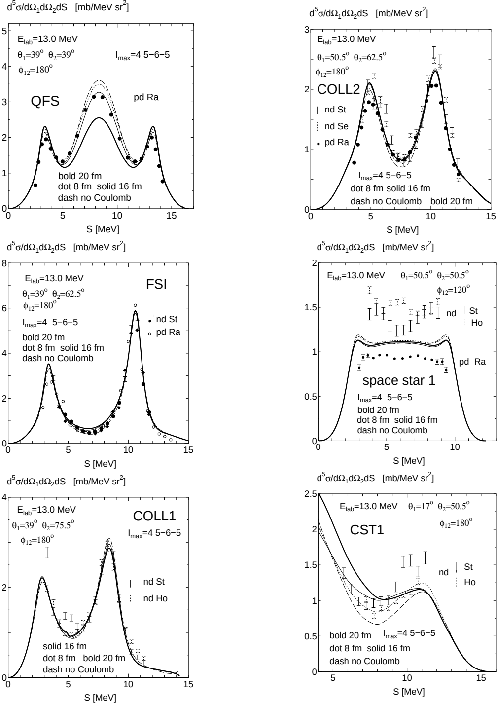
Fig. 13 Breakup differential cross sections for the nd and pd reactions at E_N = 13 MeV for the quasi-free scattering (QFS), the final state interaction (FSI), the collinear configurations (COLL1, COLL2), the symmetric space star (space star 1), and the coplanar star (CST1) configurations. The nd result is shown by the dashed curve and the pd results by the dotted ( \rho = 8 fm), solid ( \rho = 16 fm) and bold solid ( \rho = 20 fm) curves. The experimental data are taken from Ref. [109] for the quasi-free scattering, Refs. [109] ( pd ) and [110; 111; 112] ( nd ) for the final state interaction, Refs. [109] ( pd ) and [110; 111; 113] ( nd ) for the collinear configurations, Refs. [110; 111; 112; 113] ( nd ) and [109] ( pd ) for the space star configuration, and Refs. [110; 113] for the coplanar star configuration.
