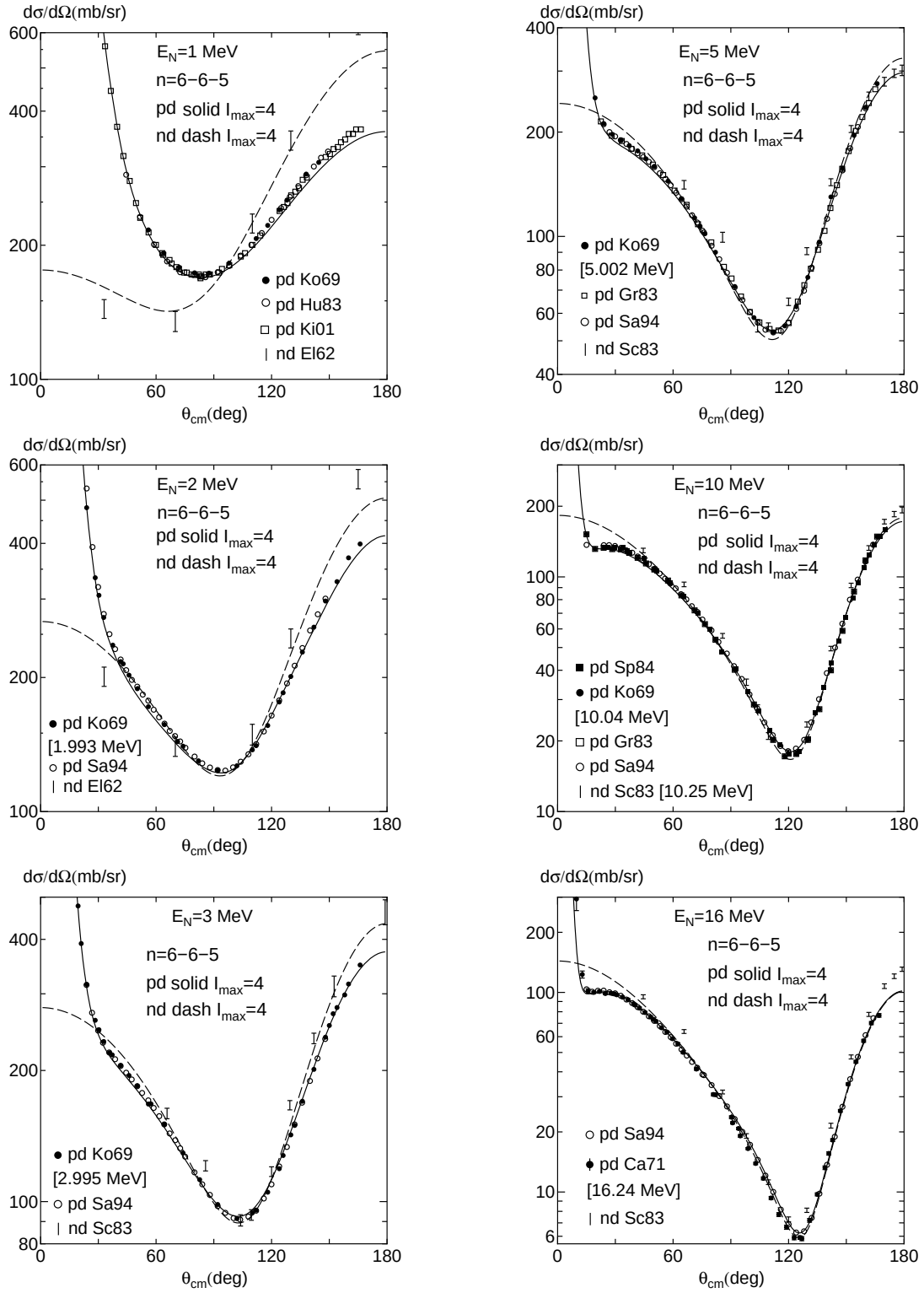
Fig. 5 nd and pd differential cross sections from E_N = 1 to 16 MeV, compared with the experimental data. The solid curve shows the pd prediction by fss2 with the screened Coulomb force and the dashed curve shows the nd calculation. The experimental data are taken from Refs. [71] for Ko69, [72] for Hu83, [73] for Ki01, [74] for El62, [75] for Sa94, [55] for Sc83, [76] for Gr83, [77] for Sp84, and Ref. [78] for Ca71.
