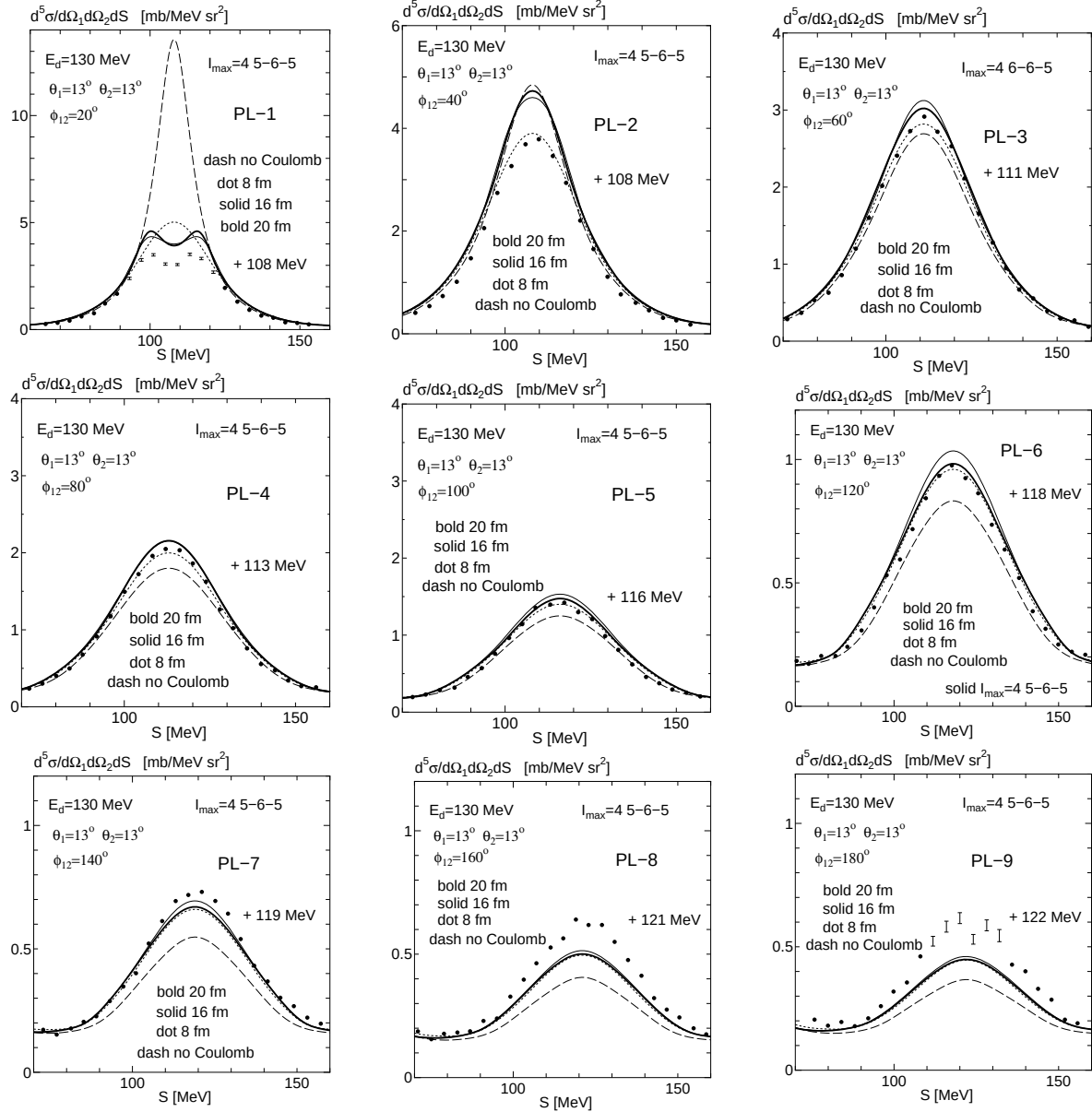
Fig. 15 Breakup differential cross sections for the reaction ^1\text{H}(\vec{d}, 2p)n at E_d = 130 MeV, compared with the experimental data [118]. The nd results are shown by the dashed curves. For the dp calculations, the Coulomb cutoff parameter \rho is chosen to be 8 (dotted), 16 (solid) and 20 fm (bold solid curves). Here, the kinematical conditions are \theta_1 = \theta_2 = 13^\circ , and \phi_{12} are changed from 20^\circ to 180^\circ with a step of 20^\circ . The calculated curves are shifted by about 100 MeV with respect to S to fit the experimental origin.
