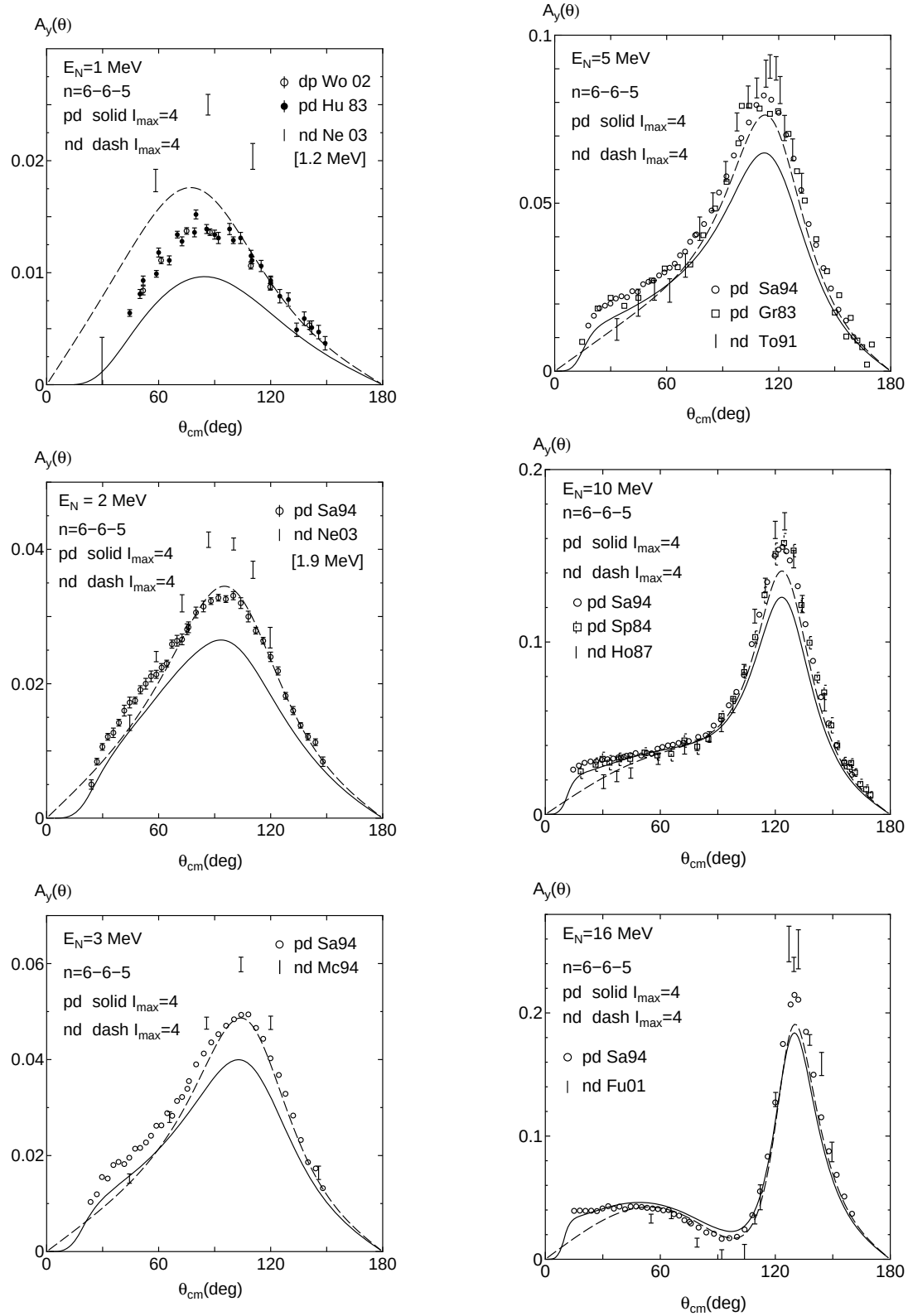
Fig. 8 Nucleon analyzing power A_y(\theta) for the nd and pd elastic scattering from E_N = 1 to 16 MeV, compared with the experimental data. The experimental data are taken from Refs. [96] for Wo02, [87] for Ne03, [88] for Mc94, [89] for To91, [90] for Ho87, and Ref. [92] for Fu01. The others are same as in Fig. 5.
