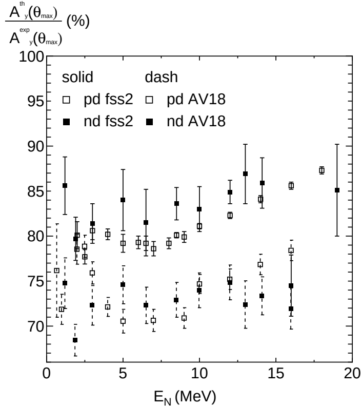
Fig. 7 Relative magnitudes of the theoretical predictions to the experimental data for the pd (open squares) and nd (filled squares) analyzing powers in the maximum angular points of A_y(\theta) . See Eq. (4.3). The experimental data are taken from Refs. [75; 86] for the pd scattering, and Refs. [87; 88; 89; 90; 91; 92; 93] for the nd scattering. The results for AV18 are also shown by open and filled squares with dashed errorbars for comparison. The nd calculations using AV18 are from Witała [94] and pd calculations from Kievsky [95].
