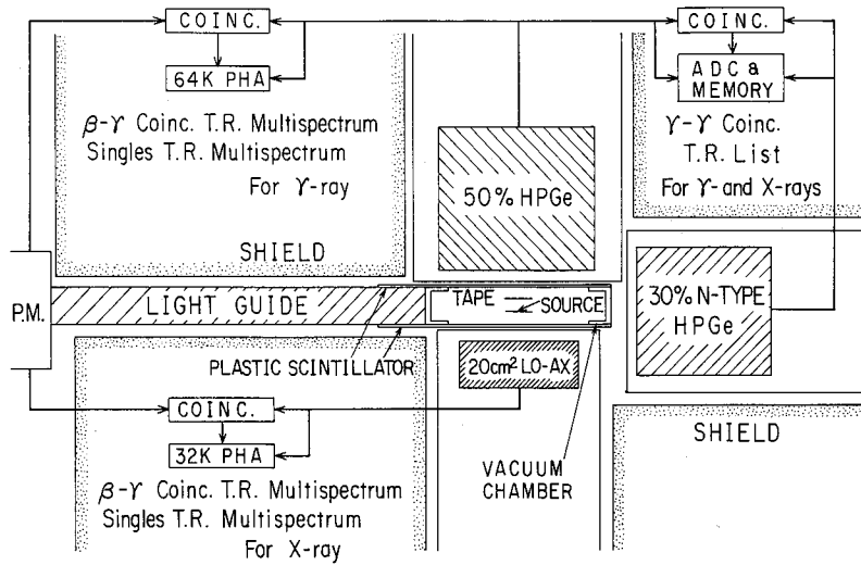
Fig. 6. Geometrical configuration of a 4\pi\beta - \gamma , 4\pi\beta -X and \gamma - \gamma coincidence measuring system using two 80\text{ mm} \times 80\text{ mm} \times 1\text{ mm} plastic scintillators, 50% and 30% HPGe \gamma -ray detectors and a HPGe low-energy photon detector.
