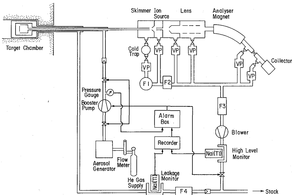
Fig. 1. Schematic diagram of the He-jet type KUR-ISOL. The helium flow path is explicitly shown: A small amount of oxygen is added to helium in the case of oxidation method. VP: vacuum pump; F1~F3: filters and cooling chambers.
