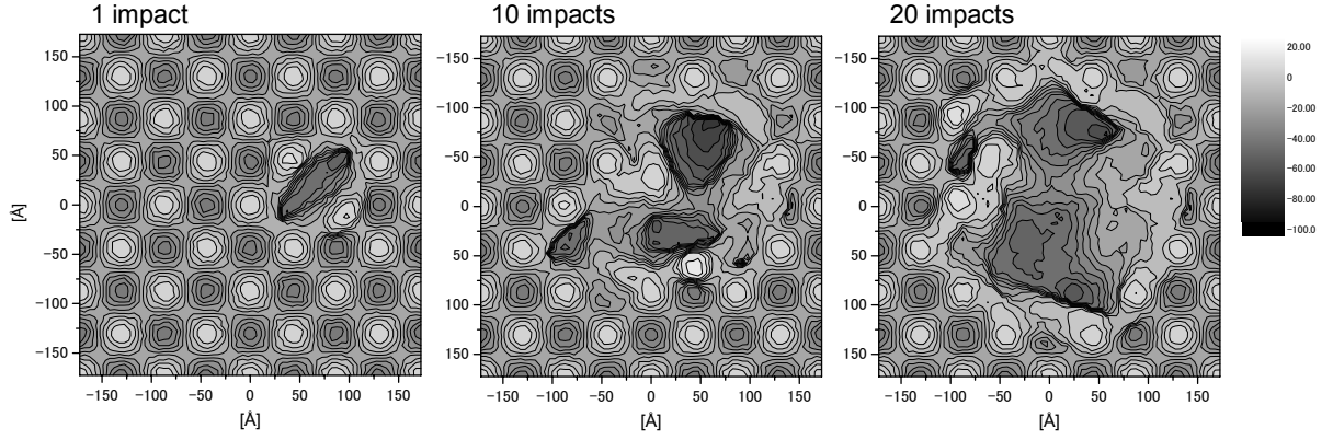
Fig. 2: Contour map of Si surface after 1, 10 and 20 impacts of \text{Ar}_{2000} 20keV. Initial surface has 2-D sine curved profile with 40Å of peak-to-valley. Lines are drawn on every 5Å.
