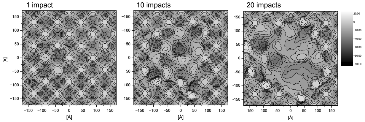
Fig. 3: Contour map of surface profile after 1, 10 and 20 impacts of \text{Ar}_{13333} 20keV.
