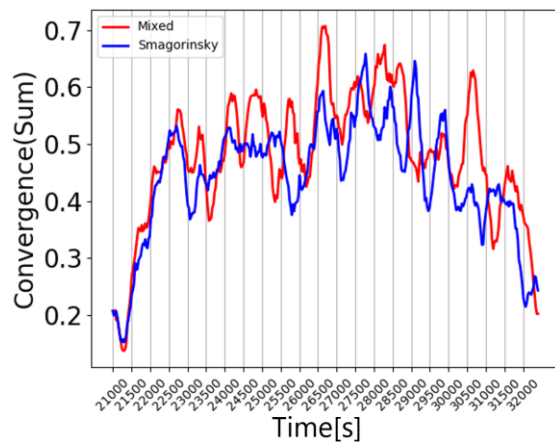
Fig. 9 Time-series data of total of horizontal convergence value in extracted grids.
