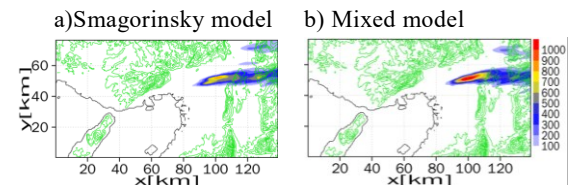
Fig. 5 Accumulation of rainwater mixing ratio[g/kg] during occurrence of line-shaped rain bands.
