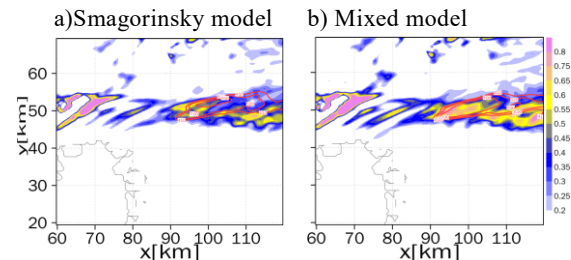
Fig. 6 Accumulation of horizontal convergence[1/s] at 1km altitude during occurrence of line-shaped rain bands. Red contour represents accumulation of rainwater mixing ratio[g/kg].
