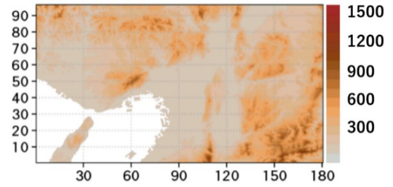
Fig. 1 Calculation domain and topography.
