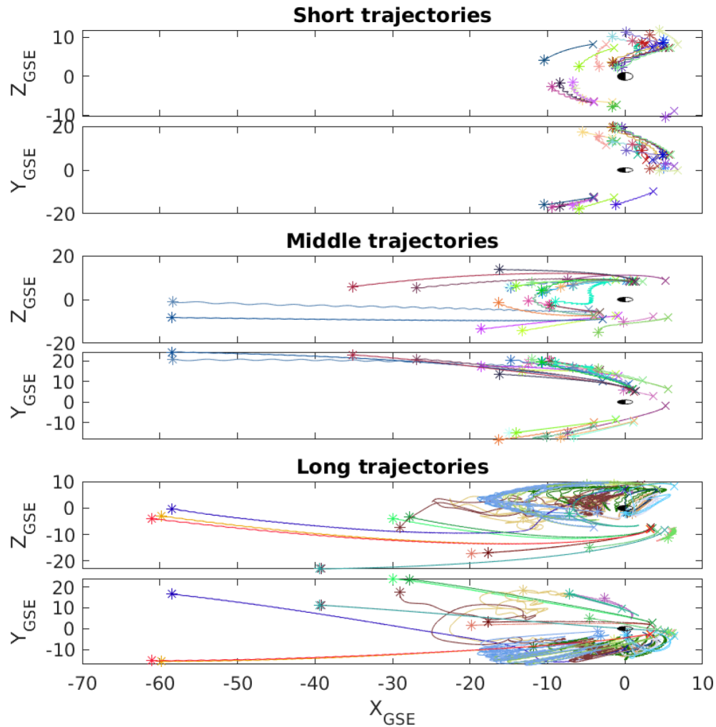
Figure 4. Sample of 25 short, middle, and long trajectories in the XZ and XY planes. Units of the axes are in R_e . Each colour represents one trajectory, and the crosses and the asterisks show the initial and final position respectively.
