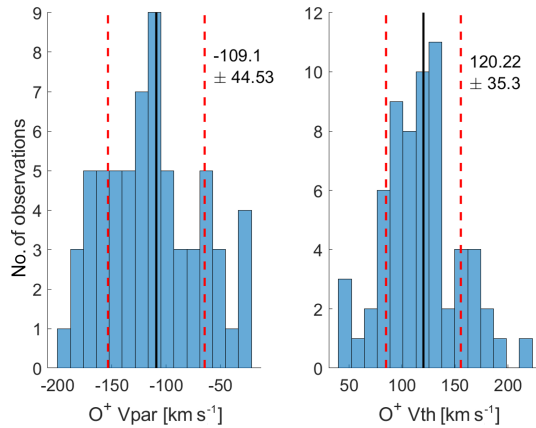
Figure 2. Cluster SC4 observations: parallel and thermal components of the O + velocity on 11 June 2001 between 01:24 and 01:29 UT. The solid black line represents the mean and the dashed red lines show the standard deviations.
