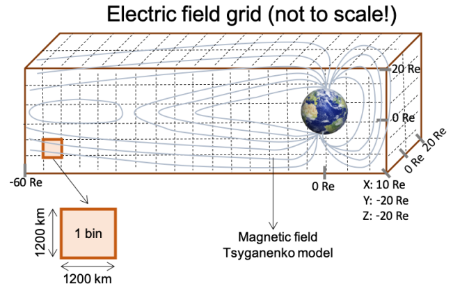
Figure 1. Schematic representation of the modelling of the Earth's environment. The Earth's magnetosphere is represented in light grey and the brown grid displays the electric field grid. Note that the illustration is not to scale.
