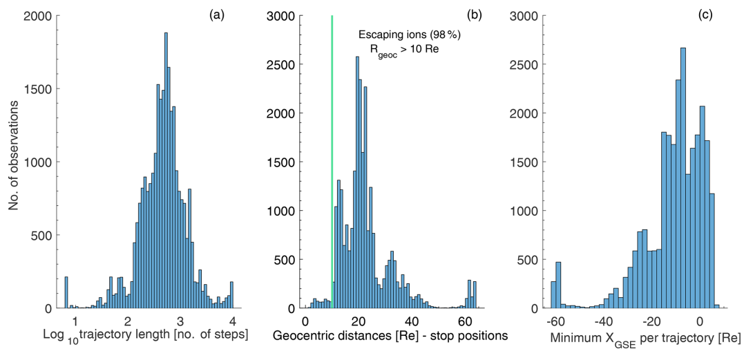
Figure 5. (a) Length of the 26 200 O^+ trajectories in our sample. Note the logarithmic scale. (b) Final positions expressed in the geocentric distance R given in R_e (see text for definition). (c) Minimum X distance for each trajectory.
