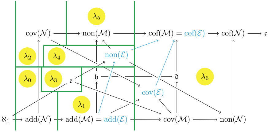
Figure 11: Constellation of Problem 4.22 (5)
