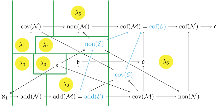
Figure 10: Constellation of Problem 4.22 (4)
