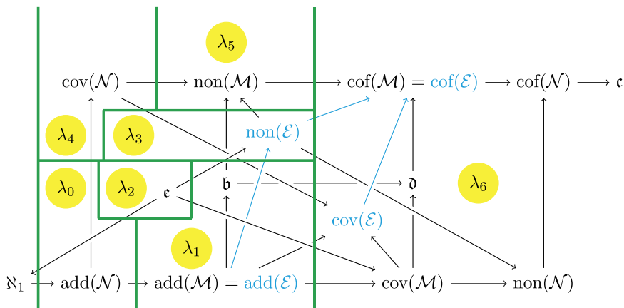
Figure 13: Constellation of Problem 4.22 (7)
