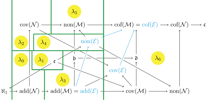
Figure 16: Constellation of Problem 4.22 (10)
