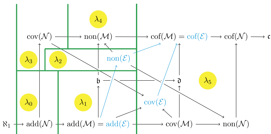
Figure 8: Constellation of Problem 4.22 (2)
