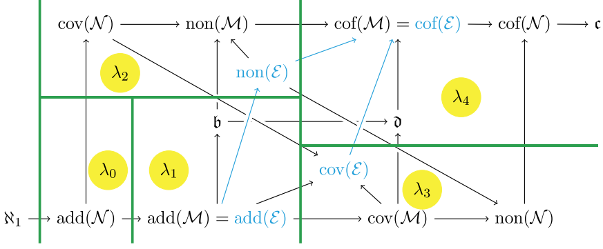
Figure 6: Constellation forced in Theorem 4.21
