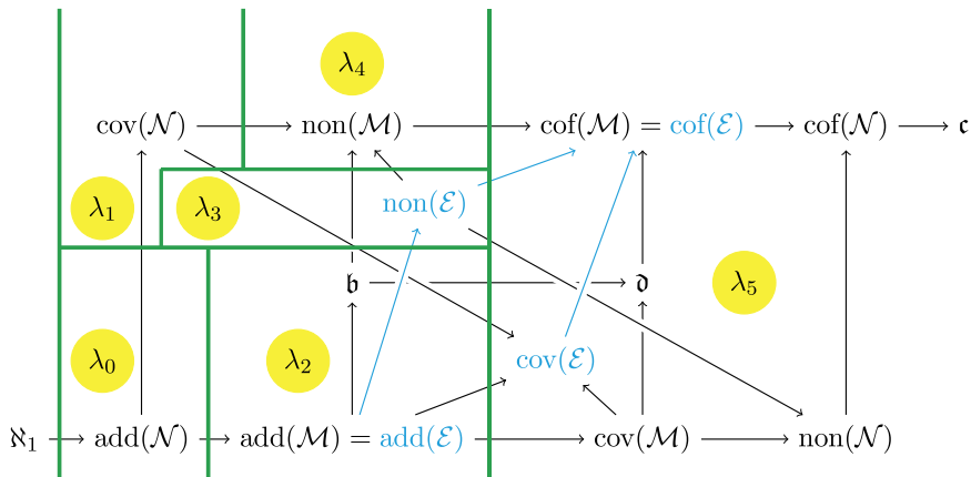
Figure 7: Constellation forced in Problem 4.22 (1)
