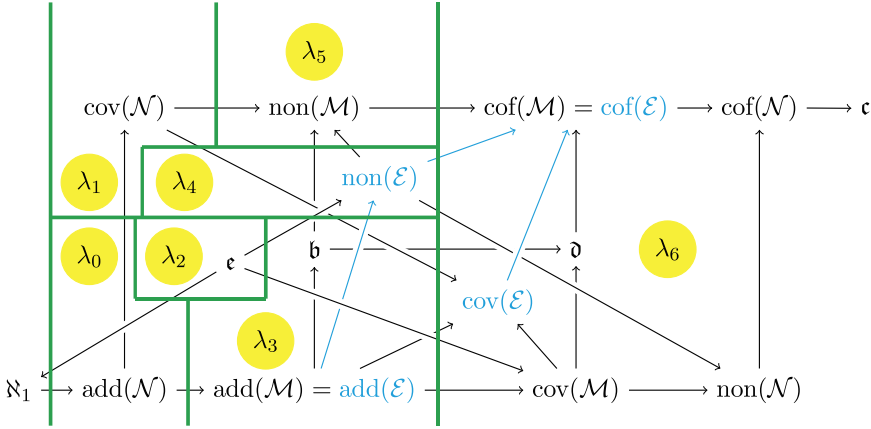
Figure 17: Constellation of Problem 4.22 (11)
