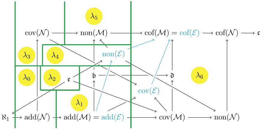
Figure 12: Constellation of Problem 4.22 (6)
