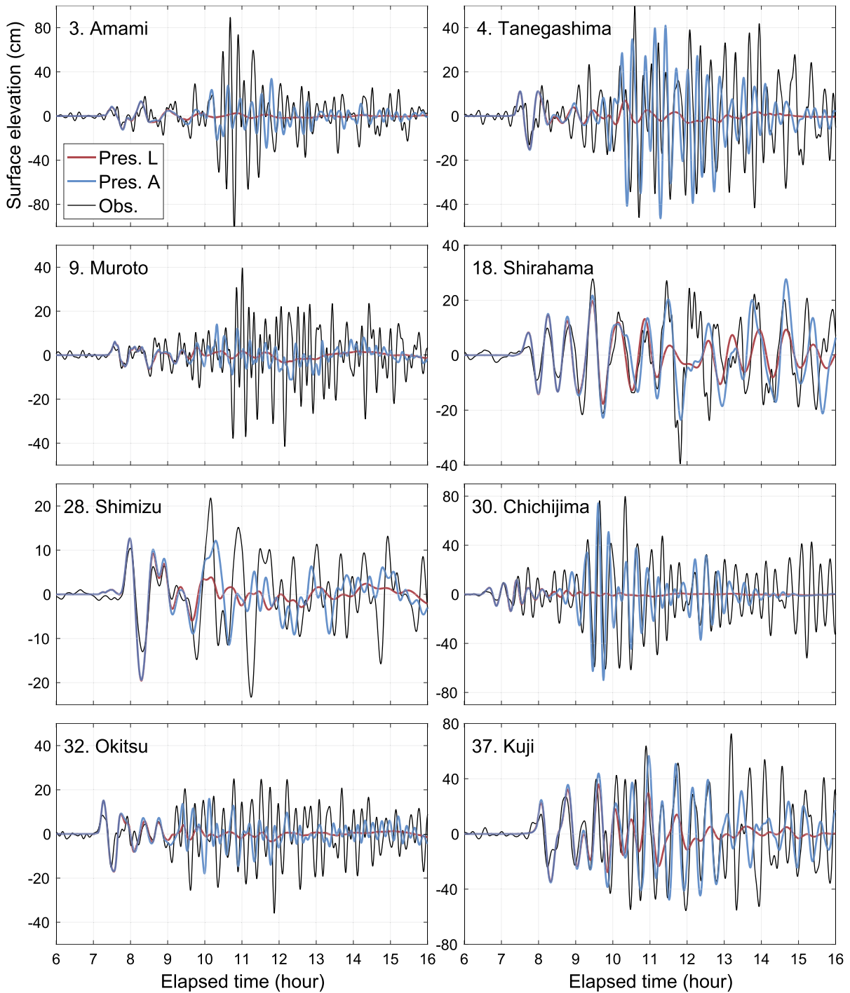
Figure 8 Comparison between simulated and observed tsunami waveforms at coastal gauges. Black lines represent observed waveforms. Red and blue lines represent simulated waveforms for Pressure L and A conditions, respectively
