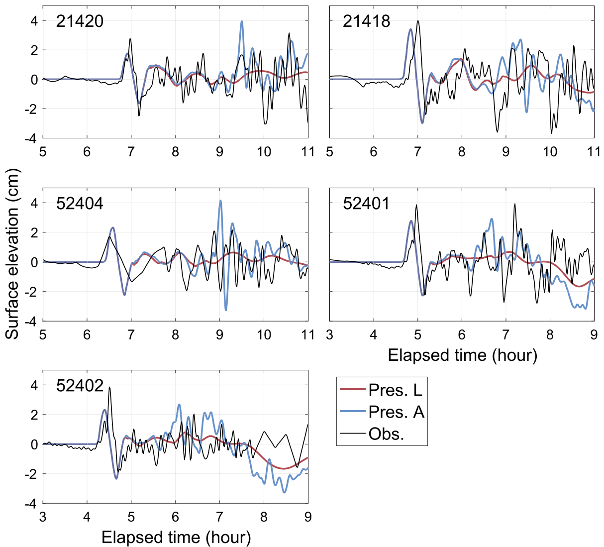
Figure 6 Comparison of simulated and observed pressure-forced waves
