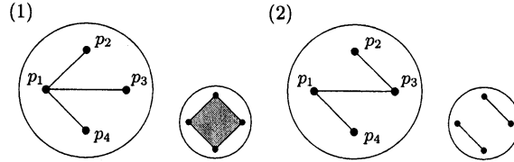
Figure 3: (1) \Gamma(a_{1,2}a_{2,3}a_{3,4}) , P_{a_{1,2}a_{2,3}a_{3,4}} and (2) \Gamma(a_{1,4}a_{2,3}) , P_{a_{1,4}a_{2,3}}
