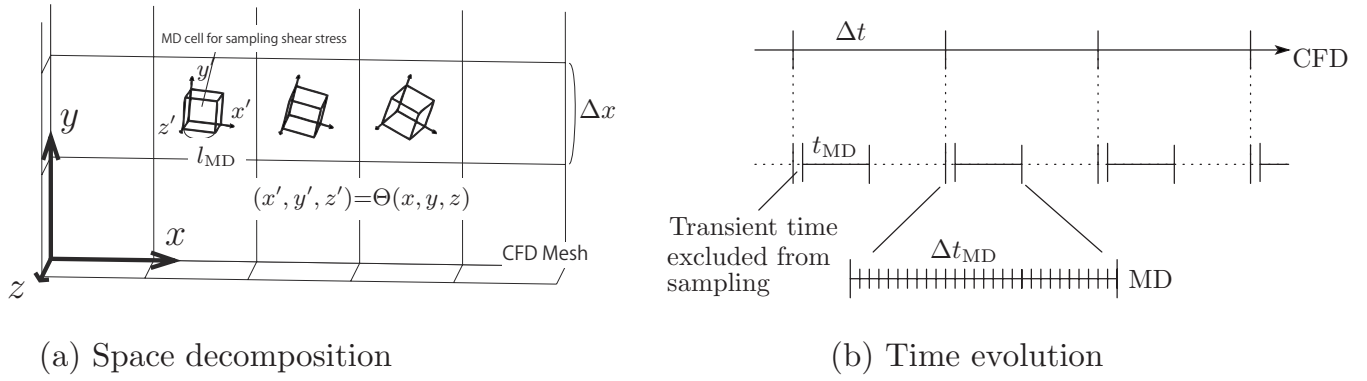
FIG. 2. Schematic for the hybrid scheme. (a) CFD simulations are performed in a reference coordinate (x, y, z) , while MD simulations are performed in a rotated coordinate (x', y', z') so that the diagonal components of E'_{\alpha\beta} all become zero with the procedure described in Sec. II B. The CFD system is discretized into cubic subsystems whose side length is \Delta x . Each subsystem is associated with a MD cell, whose side length is l_{MD} , with Lees–Edwards periodic boundary condition under shear deformation. Note that three-dimensional MD simulations are used at the microscopic level even for the problems that 1D or 2D analysis is applied at the macroscopic level. (b) A schematic time evolution of our multiscale method. The CFD simulation proceeds with a time step of \Delta t , and the MD simulation is carried out for a lapse of time t_{MD} only to sample the local stress T'_{\alpha\beta} at each node point and time step of CFD.
