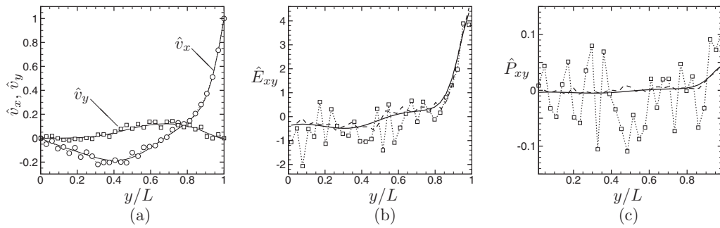
FIG. 8. Comparisons between the instantaneous profiles obtained by the hybrid simulation and those by CFD for the cavity flow for Re=235 . The velocity U\hat{u}_\alpha , strain rate (U/L)\hat{E}_{xy} , and shear stress (\rho U^2)\hat{P}_{xy} on the line of x/L=0.5 are plotted. The symbols show the results of the hybrid simulation and the solid lines those of CFD. The dashed lines in (b) and (c) show the time averages over t/\Delta t=[900, 1000] .
