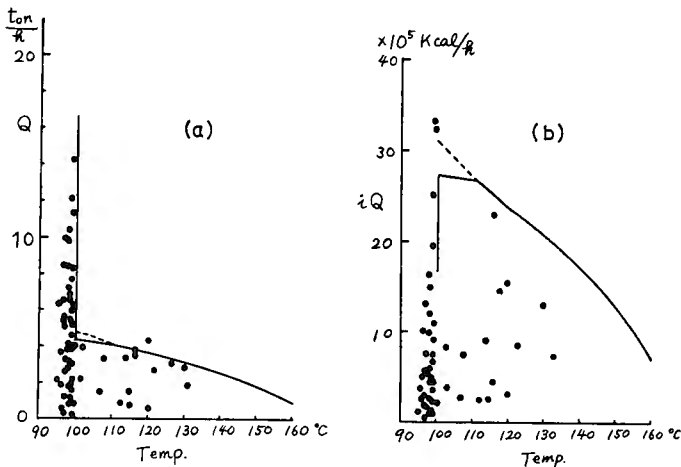
Fig. 3. Comparisons of observed fluxes through boiling and steam wells in Beppu (Yuhara [1965]) and the highest limits theoretically expected under the pressure of 1 atm.
