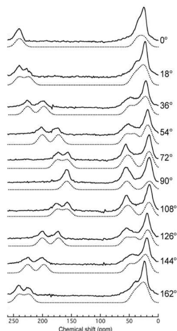
Fig. 1 ^{13}\text{C} CP spectra of L-alanine microcrystals in a suspension under the modulated rotating magnetic field. The spectra simulated from the single-crystal data are also shown as dashed lines.
