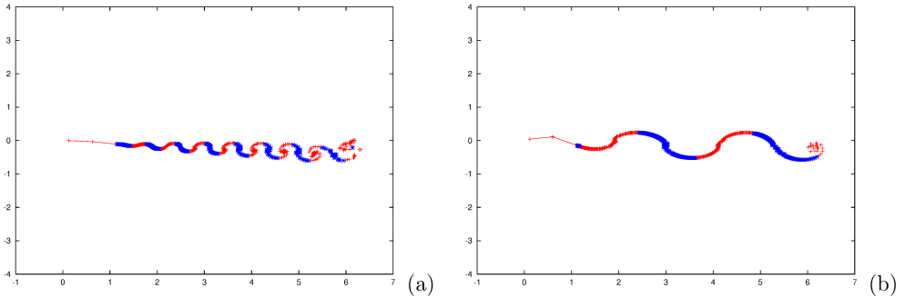
Figure 2: (a) Vibrating flag (plate) at a low flow speed. (b) The flag at the threshold of flutter. (In color (pdf/online), red points represent counter-clockwise rotating vortices, and blue clockwise rotating vortices.)
