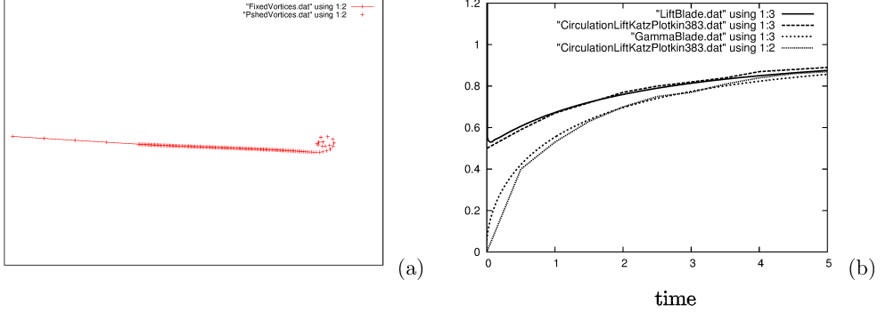
Figure 1: (a) A plate impulsively started from rest. (b) Comparison between discrete vortex results and Theodorsen's solution.
