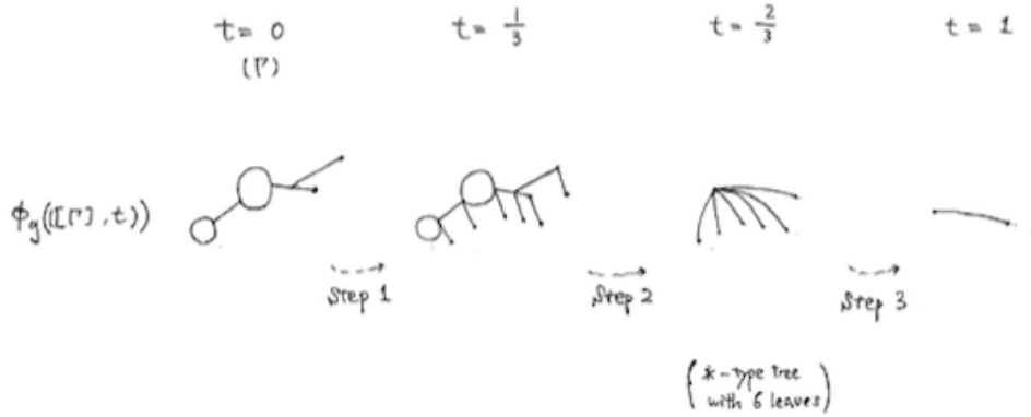
FIGURE 2. Picture proof of Theorem 4.4
