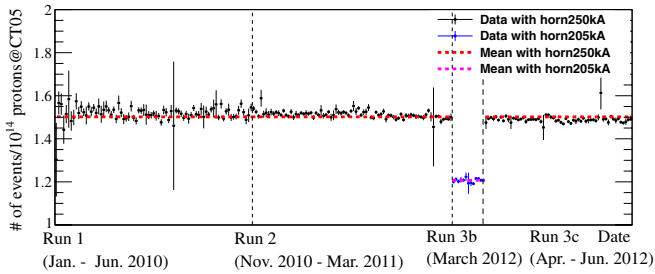
FIG. 12 (color online). Neutrino events per 10^{14} POT measured by INGRID (points) overlaid with mean value (dashed lines). The error bar represents the statistical error on the INGRID measurement.
