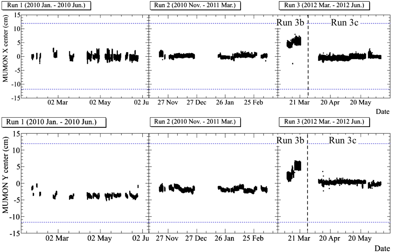
FIG. 11 (color online). Time history of the measured muon profile center at MUMON in all run periods. A top and bottom figure shows the profile center in the horizontal (X) and the vertical (Y), respectively. A dashed line corresponds to 1 mrad at MUMON. Both directions are controlled within 1 mrad.
