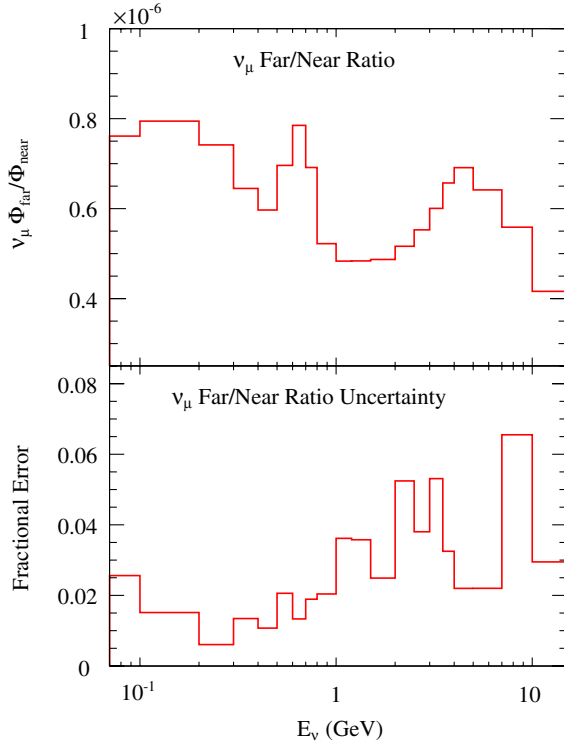
FIG. 45 (color online). The far/near ratio for the \nu_\mu flux prediction (top) and the uncertainty on the ratio (bottom).
