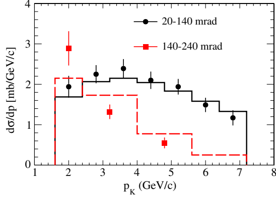
FIG. 30 (color online). The BMPT fits to the NA61/SHINE K^+ data.
