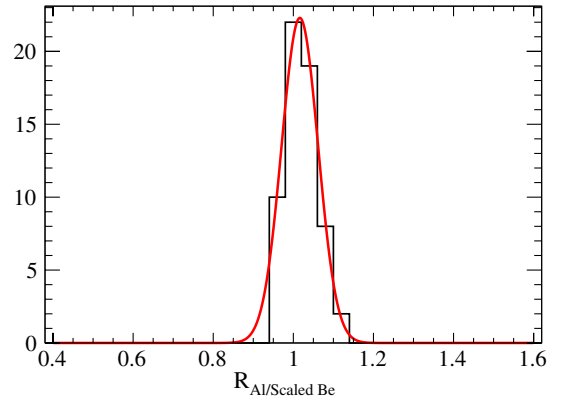
FIG. 33 (color online). Distribution of the ratios of Al to scaled Be yields, R_{\text{Al/Scaled Be}} , for the [27] K^+ data. The fit (Gaussian function), which extracts the mean and r.m.s. of the distribution, is overlaid.
