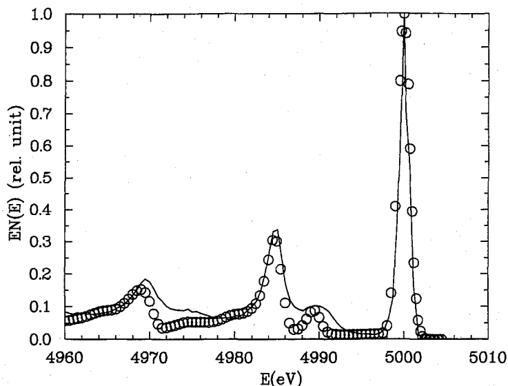
Fig. 4. Electron spectra backscattered from the amorphous aluminum sample near the elastic peak: — measured by Némethy et al. (Ref. 15); ○ calculated (The spectrum was convoluted for finite relative energy resolution, E=5 keV and \Delta E/E=0.035\% .)
