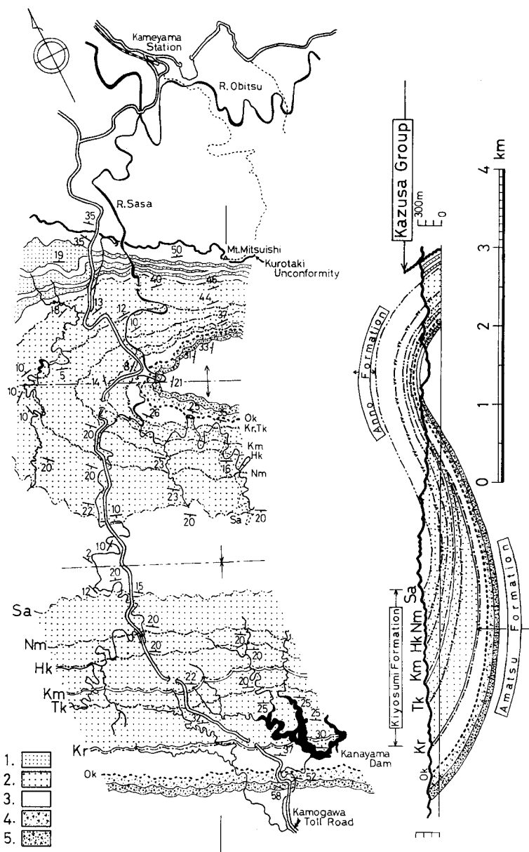
Fig. 4. Localities of the main six tuff marker-beds along the type route (Kamogawa Toll Road and Sasa River).
