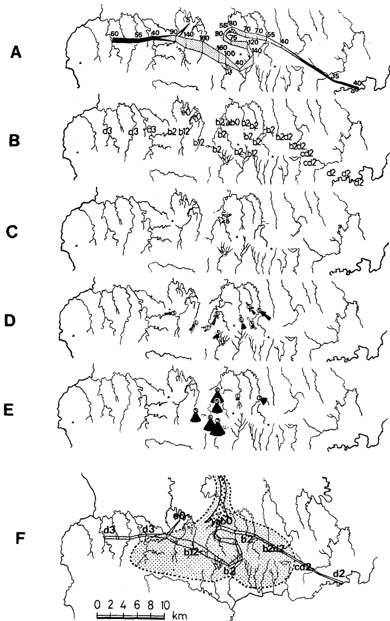
Fig. 20. Summary of some basic sedimentological data on the Hk-Km unit (A-E) and an inferred depositional pattern of the unit (F).
