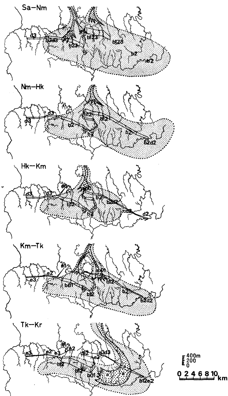
Fig. 22. Inferred depositional process of the Kiyosumi Formation.
