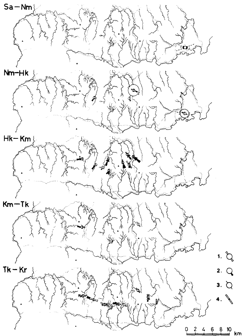
Fig. 16A. Paleocurrent directions measured by some sedimentary structures indicating distinct orientation.
