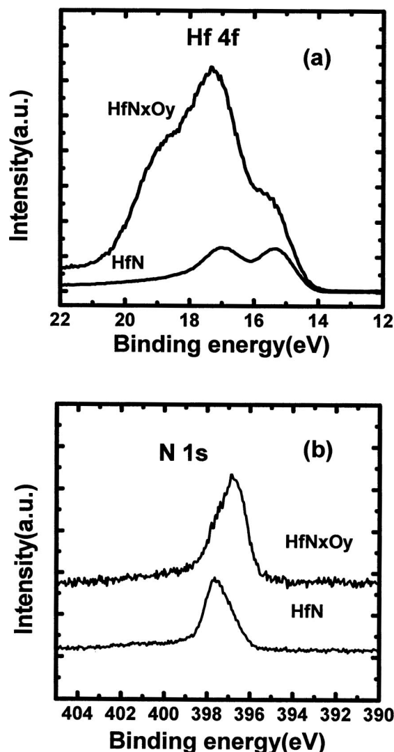
FIG. 1. X-ray photoelectron spectra of Hf 4f (a) and N 1s (b) from a \text{HfN}_x\text{O}_y film compared with HfN.
