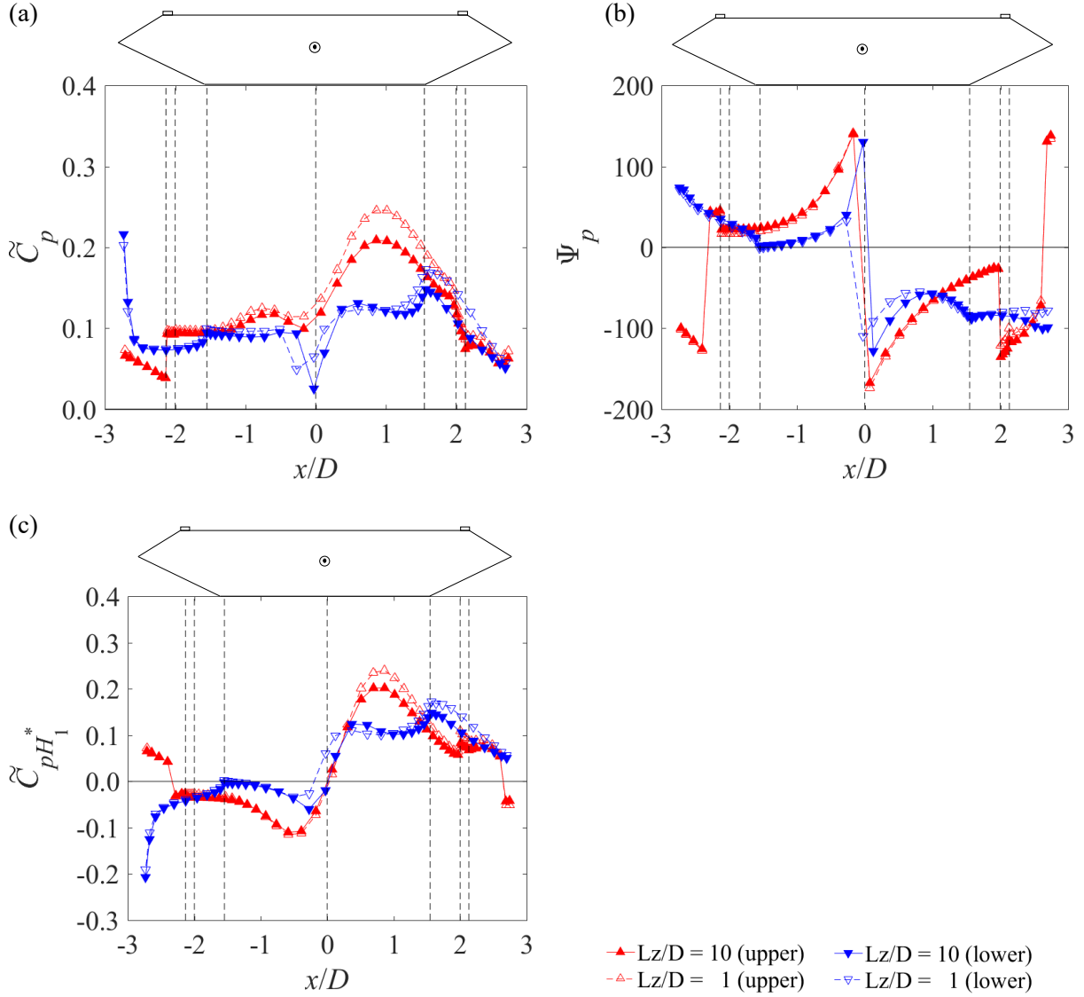
Fig. 12. Effects of spanwise domain size on unsteady pressure at each location. (a) amplitude ( \tilde{C}_p ) of unsteady pressure, (b) phase lag ( \Psi_p ) of unsteady pressure, (c) aerodynamic damping ( \tilde{C}_{pH_1^*} ).
