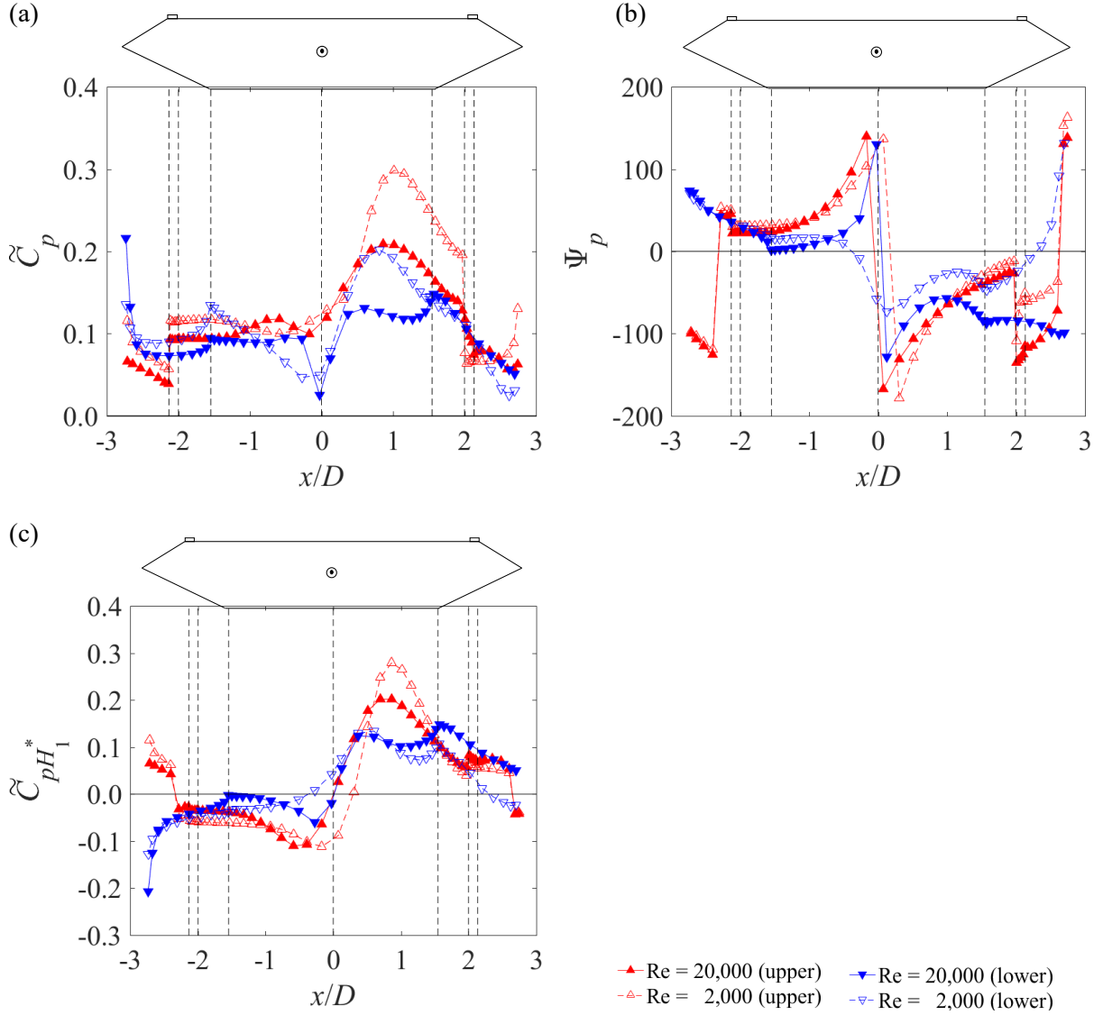
Fig. 15. Effects of Reynolds number on unsteady pressure. (a) amplitude ( \tilde{C}_p ) of unsteady pressure, (b) phase lag ( \Psi_p ) of unsteady pressure, (c) aerodynamic damping ( \tilde{C}_{pH_1^*} ).
