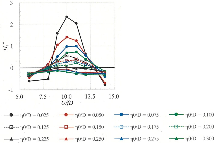
Fig. 7. Flutter derivatives of heaving aerodynamic damping ( H_1^* ) for each nondimensional oscillation half amplitude ( \eta_0/D ) as a function of reduced wind speed ( U/fD ).
