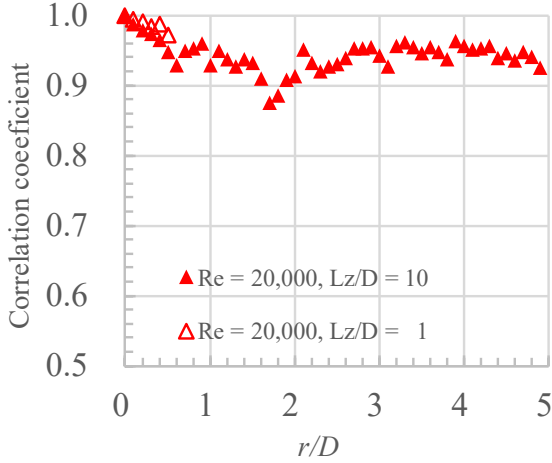
Fig. 13. The correlation coefficient of pressure along the span at x/D = 0 .
