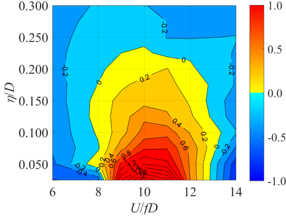
Fig. 8. Contour figure of aerodynamic damping ( H_1^* ) as a function of reduced wind speed ( U/fD ) and nondimensional oscillation half amplitude ( \eta_0/D ).
