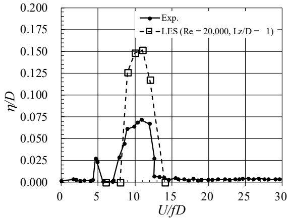
Fig. 10. Velocity–amplitude diagram obtained by the wind tunnel tests and LES.
