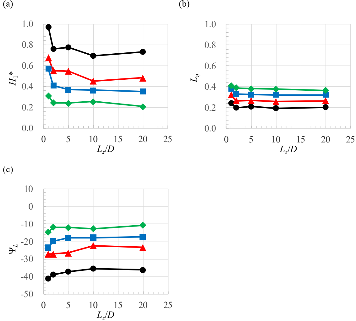
Fig. 11. Effects of spanwise domain size on unsteady lift force. (a) aerodynamic damping ( H_1^* ), (b) amplitude ( L_\eta ) of unsteady lift force, (c) phase lag ( \Psi_L ) of unsteady lift force.
