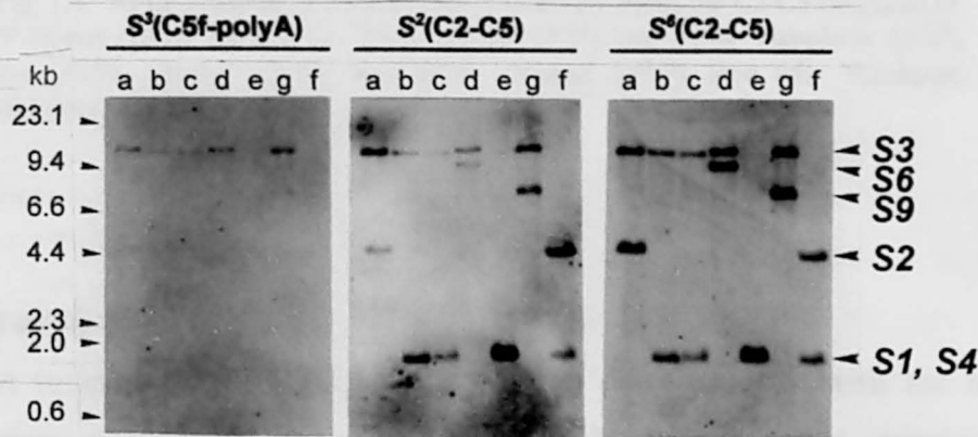
Fig. 1.7. Genomic DNA blot analysis using the C5f-polyA and C2-C5 fragments of the cDNAs encoding S^2 , S^3 , and S^6 -RNases of sweet cherry. (a) Velvet ( S^2S^3 ), (b) Van ( S^1S^3 ), (c) Napoleon ( S^3S^4 ), (d) Satonishiki ( S^3S^6 ), (e) Rainier ( S^1S^4 ), (f) Peggy Rivers ( S^2S^4 ), and (g) Burlat ( S^3S^9 ).
