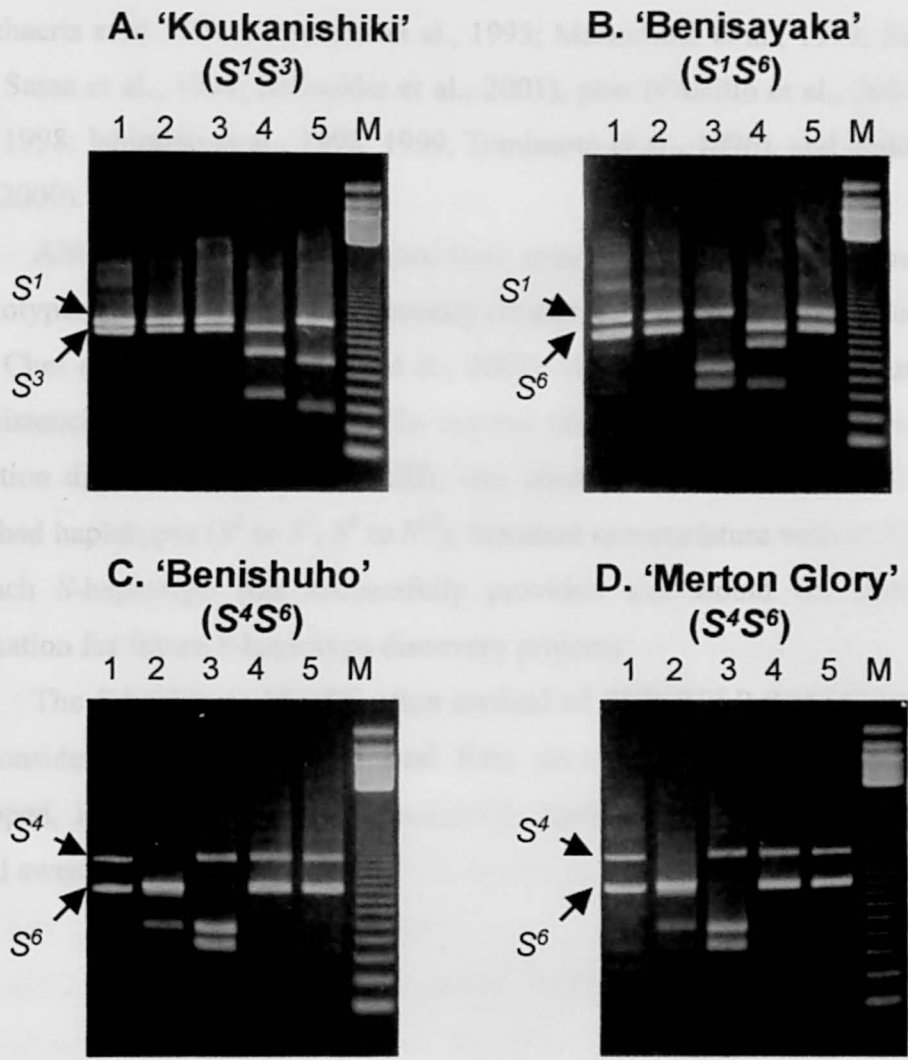
Fig. 2.5. S -haplotype typing of 4 cultivars, 'Koukanishiki' (A), 'Benisayaka' (B), 'Benishuho' (C), and 'Merton Glory' (D) by PCR-RFLP analysis. PCR products obtained using Pru-T2 and Pru-C4R primers were digested with: Lane 1: uncut, lane 2: Apa LI, lane 3: Ava I, lane 4: Ban II, and lane 5: Nru I. Lane M: 123 bp ladder.
