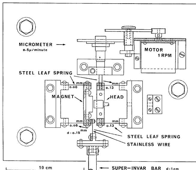
Fig. 2 Detector of strainmeter (magnetic sensor type)
