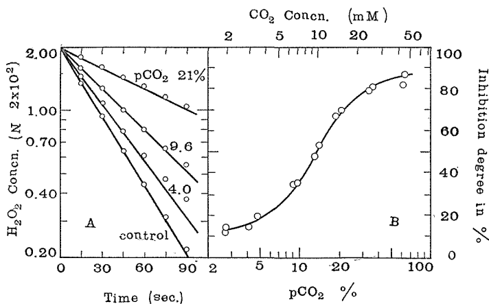
Fig. 2. Effects of carbon dioxide on the catalatic activity.
