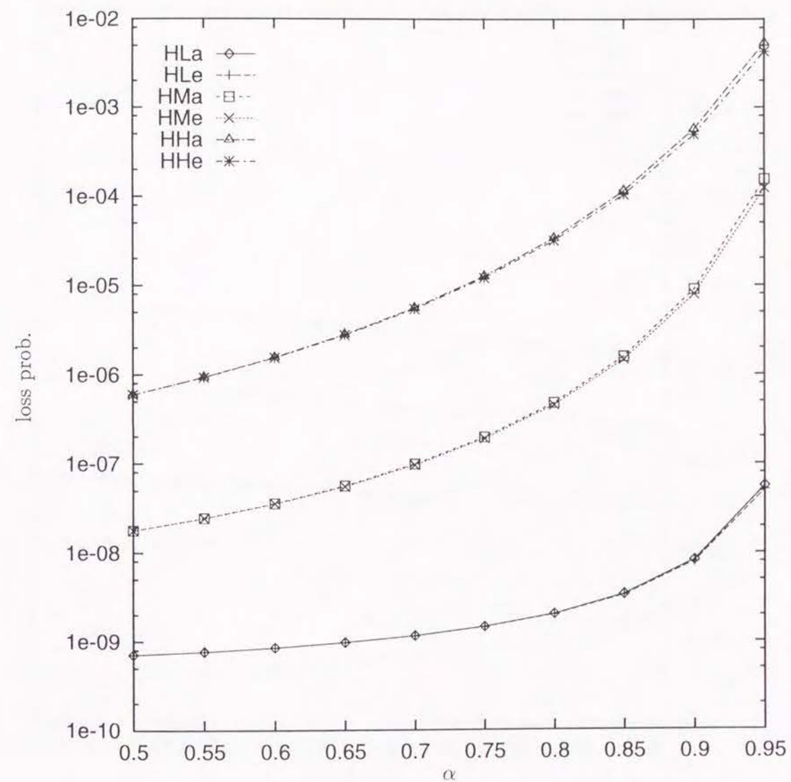
Figure 3.3: Loss Probability Approximation as a Function of \alpha (Early Arrival Model, N = 91 , \rho = 0.8 )
