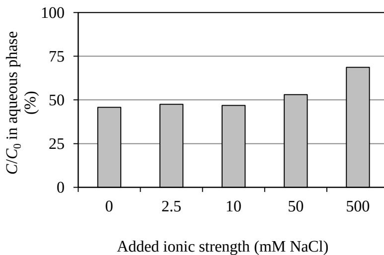
Fig. 4. 2. 11 nC_{60} adsorption on activated sludge as a function of ionic strength.
