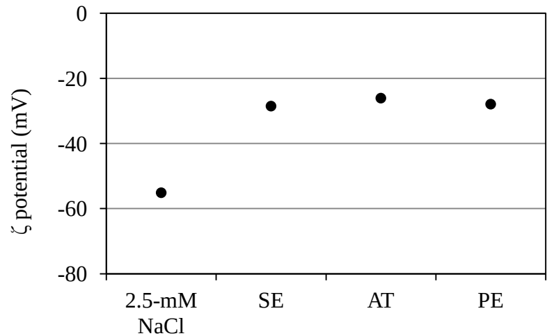
Fig. 4. 1. 4 \zeta potential of nC 60 in water samples. PE: primary effluent; AT: aeration tank liquor; SE: secondary effluent
