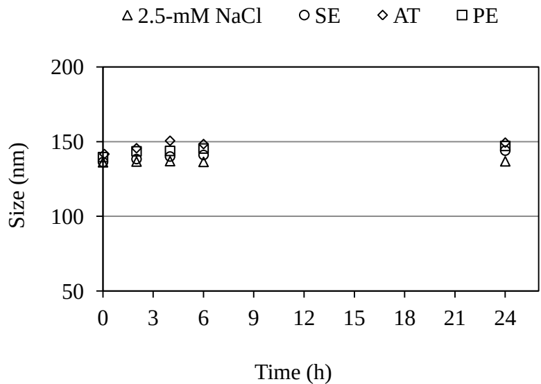
Fig. 4. 1. 3 Time profile of nC 60 aggregation in water samples. PE: primary effluent; AT: aeration tank liquor; SE: secondary effluent
