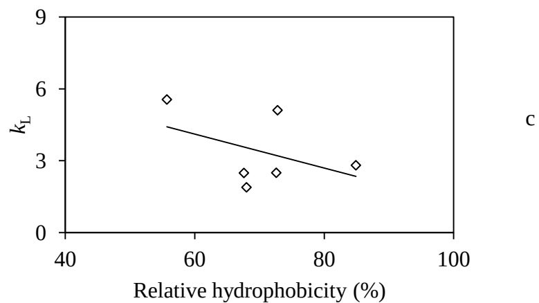
Fig. 4. 2. 19 Correlation of Langmuir coefficient ( k_L ) and surface properties of activated sludge: (a) \zeta potential, (b) size, and (c) relative hydrophobicity.
