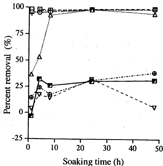
Fig. 1. Percent removal of mercury after soaking carbonized Japanese cedar wood powder in 5 ppm mercuric chloride solution. Legend: ..... \triangle ..... 400°C*, ..... \square ..... 1,400°C*, .....+..... 600°C*, ..... \blacksquare ..... 1,600°C*, ..... \circ ..... 1,000°C*, ..... \oplus ..... 2,000°C*, ..... \diamond ..... 1,200°C*, ..... \nabla ..... 2,400°C*. Note: *-carbonization temperature.
