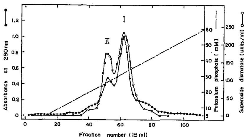
FIG. 1. Linear gradient chromatography of the soluble superoxide dismutase isozymes from Euglena on DEAE Sephadex. Details are given in the text.
