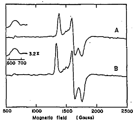
Fig. 9. Electron paramagnetic resonance spectra of Azotobacter Fe-SOD. A, 0.80 mM Native enzyme in 0.1 M Tris-HCl, pH 7.8; B, 0.87 mM reconstituted 57 Fe-enzyme in the same buffer. The spectra were recorded at 4.2K with the following instrumental setting: microwave power, 0.5 mW; microwave frequency, 9.274 GHz; modulation amplitude, 1 G; receiver gain, 10 4 ; field modulation, 100 kHz; time constant, 0.3 sec; and sweep rate, 500 G/min. The signals at g = 9.8 were similarly obtained except that the modulation amplitude and time constant were 3.2 G, and 1 sec, respectively.
