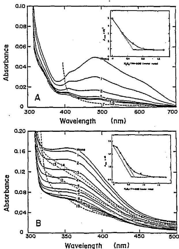
Fig. 3. Spectroscopic titration of Mn- and Fe-SOD by hydrogen peroxide. Porphyrin Mn-SOD (50.6 \mu\text{M} ) (A) in 0.7 ml of 10 mM potassium phosphate, pH 7.8, and Azotobacter Fe-SOD (94.6 \mu\text{M} ) (B) in 0.9 ml of the same buffer were successively titrated with 5 or 10 \mu\text{l} of 2 mM \text{H}_2\text{O}_2 , respectively. (A) 1 to 5, each 5 \mu\text{l} \text{H}_2\text{O}_2 ; 6, 5 was standed for 15 min; 7, solid dithionite was added. (B) 1 to 6, each 5 \mu\text{l} \text{H}_2\text{O}_2 ; 7-11, each 10 \mu\text{l} ; 12, same as 11 except it was standed for 15 min; 13, 30 min; 14, 45 min; 15, solid sodium ascorbate was added. (Inserted), the bleachings of the absorption at 480 nm for Mn-SOD (A) and at 350 nm for Fe-SOD (B) were plotted as a function of molar ratio of \text{H}_2\text{O}_2 against the enzyme, respectively. The correction was made for the dilution due to the addition of \text{H}_2\text{O}_2 . Each spectrum was taken after 30 sec for Mn-SOD or 1 min for Fe-SOD after the addition of \text{H}_2\text{O}_2 .
