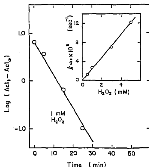
Fig. 2. Inactivation of Azotobacter Fe-SOD by hydrogen peroxide. The enzyme (2.84 \mu M) was incubated with H_2O_2 at 0.5, 1, 3, and 5 mM in 10 mM potassium phosphate, pH 7.8, at 25°C and the remaining activity was measured using 10 \mu l sample at the indicated intervals in the assay system containing 500 units catalase. The pseudo-first order rate constants for the inactivation were obtained from the plots of \text{Log}(\text{Act}_t - \text{Act}_\infty) against time. Since the inactivation of the enzyme was incomplete leaving 3-9% of the initial activity, the final remaining activity was taken as the activity at infinite time ( \text{Act}_\infty ). A typical result for 1 mM H_2O_2 is indicated. (Inserted), the observed pseudo-first order rate constants were plotted as a function of H_2O_2 concentration. The second order rate constant for the inactivation was obtained from the slope.
