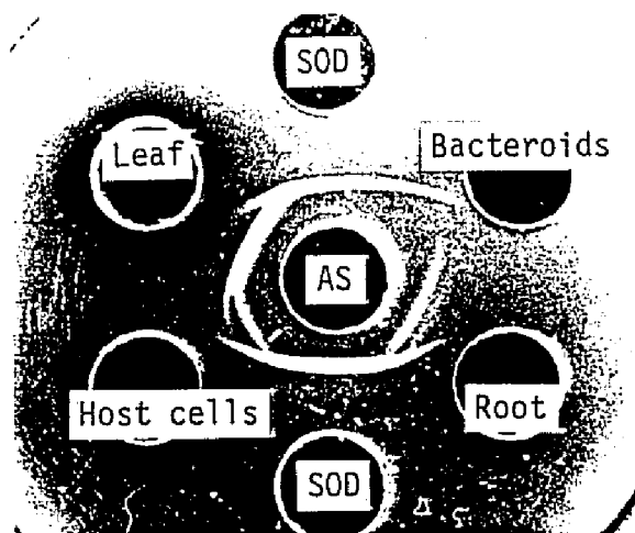
Fig. 1. Ouchterlony double immunodiffusion plate of the spinach Cu,Zn-superoxide dismutase antiserum and superoxide dismutase in cell-free extracts from soybean tissues and bacteroids in soybean root-nodules. Center well (AS) contained 260 \mu g of the antiserum to spinach Cu,Zn-enzyme, Outer wells; cell-free extracts containing 3 to 7 units of enzyme from leaves and roots of the soybean and from host cells and bacteroids of the root-nodules, SOD; spinach Cu,Zn-superoxide dismutase (1.1 \mu g, 3 units).
