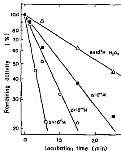
FIG. 7. Inactivation of Chromatium superoxide dismutase by hydrogen peroxide. Chromatium superoxide dismutase (1.63 \mu\text{M} ) in 50 mM sodium carbonate, pH 10.0, was incubated at 25°C with various concentrations of hydrogen peroxide, and aliquots (10 \mu\text{l} ) were withdrawn at intervals and assayed for residual enzymatic activity under standard assay conditions.
