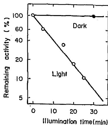
FIG. 6. Inactivation of Chromatium superoxide dismutase by photooxidation. The purified enzyme (67 \mu\text{g}/200\ \mu\text{l} ) in 50 mM potassium phosphate, pH 7.8, was exposed to a tungsten lamp (Light) or kept in the dark (Dark) in the presence of 0.005% methylene blue at 25°C. Light intensity was 460 \text{W}/\text{m}^2 . Aliquots (20 \mu\text{l} ) were removed at intervals and, after a 20-fold dilution with 10 mM potassium phosphate, pH 7.8, the remaining activity was measured using an aliquot (30 \mu\text{l} ) of the diluted solution under standard assay conditions. Although methylene blue at a high concentration stimulated the reduction rate of cytochrome c by \text{O}_2^- , under the above conditions this effect was negligible.
