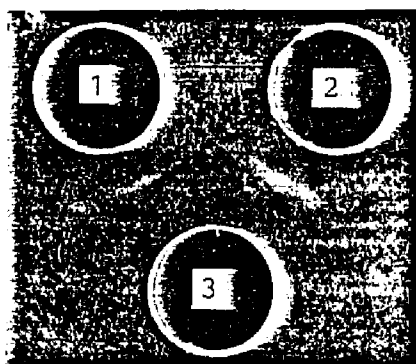
Fig. 3 Ouchterlony double immunodiffusion of Spirogyra Cu,Zn-SOD with anti- Equisetum and anti-spinach Cu,Zn-SOD sera. 1, Anti-spinach SOD serum (390 µg); 2, anti- Equisetum SOD serum (195 µg); 3, Spirogyra Cu,Zn-SOD (2 µg). Each well contained 15 µl of serum or enzyme. Diffusion was conducted at 37°C for 12 hours.
