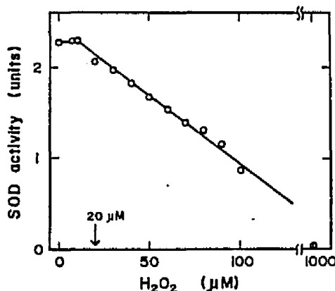
Fig. 9. Titration of Fe-SOD by hydrogen peroxide for its activity. Fe-SOD ( 20 \mu\text{M} ) was incubated with indicated concentrations of \text{H}_2\text{O}_2 in 100 \mu\text{l} of 10 \text{ mM} potassium phosphate, \text{pH } 7.8 , for 24 hours at 0^\circ\text{C} . After incubation, the aliquot was diluted with above buffer, and 10 \mu\text{l} of sample was measured for the remaining activity in the xanthine-xanthine oxidase-cytochrome c assay system.
