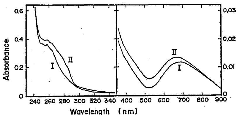
Fig. 6. Absorption spectra of rice Cu,Zn-SOD-I and -II. Spectra were recorded at 0.93 (Cu,Zn-SOD-I), and 0.99 mg/ml (Cu,Zn-SOD-II), respectively, in 10 mM potassium phosphate, pH 7.8, at 25°C. The light path was 10 mm. I, Cu,Zn-SOD-I; II, Cu,Zn-SOD-II.
