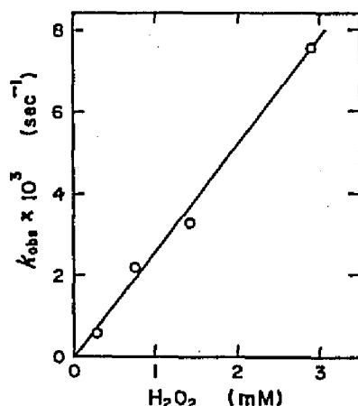
Fig. 6. Apparent second order rate constant for absorbance change at 315 nm of Fe-SOD caused by hydrogen peroxide. The reaction was started by adding indicated amount of \text{H}_2\text{O}_2 into 72 \mu\text{M} Fe-SOD in 10 mM potassium phosphate, pH 7.8, at 25°C, under the conditions of pseudo-first order reaction. The observed pseudo-first order rate constant ( k_{\text{obs}} ) was replotted against [\text{H}_2\text{O}_2] .
