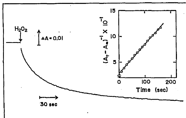
Fig. 4. The bleaching at 480 nm of Mn-SOD by hydrogen peroxide. The reaction was started by adding 54.7 \mu\text{M} \text{H}_2\text{O}_2 into 0.9 ml of 10 mM potassium phosphate, pH 7.8, containing 53.8 \mu\text{M} enzyme at 25°C. The absorbance change was recorded several second after mixing. (Inserted), the second order reaction plot. The apparent second order rate constant was calculated from a slope according to the equation, (A_t - A_\infty)^{-1} = kt + (A_0 - A_\infty)^{-1} , where A_t is absorbance at 480 nm at time t , A_0 is the initial absorbance and A_\infty is the final absorbance. A_\infty was taken as the value of 0.0165 at 72 min.
