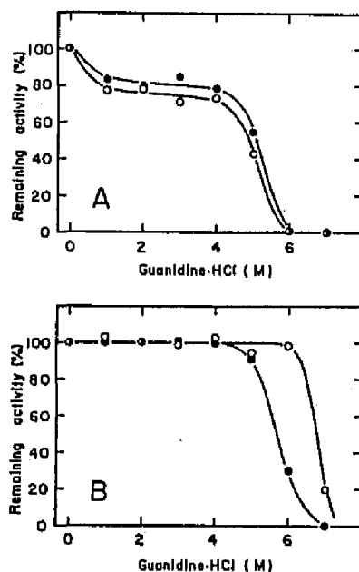
FIG. 4. Effect of guanidine on Fe-superoxide dismutases from Euglena and from procaryotes. Fe-superoxide dismutases from Euglena , Chlorobium , and Chromatium , each about 5 \mu g, were incubated for 1 h at 25°C with 50 mM potassium phosphate, 0.5 mM EDTA, and guanidine hydrochloride as indicated, in a total volume of 80 \mu l. The pH of the mixture had been adjusted to 7.8 with KOH before incubation. The remaining activity was determined using a sample (about 4 \mu l) under standard assay conditions. Introduction of guanidine to the assay mixture under the present conditions did not disturb the assay. (A) ○, Euglena isozyme-I; ●, Euglena isozyme-II. (B) ○, Chlorobium ; ●, Chromatium .
