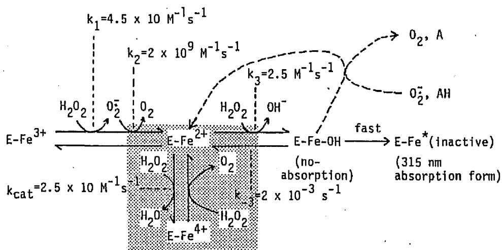
Fig. 10. Proposed reaction scheme of Fe-SOD with \text{H}_2\text{O}_2 . ■, Catalytic \text{H}_2\text{O}_2 -decomposing activity; -\rightarrow , possible reaction; AH, reductant (such as ascorbate, NADPH, glutathione, etc.).
