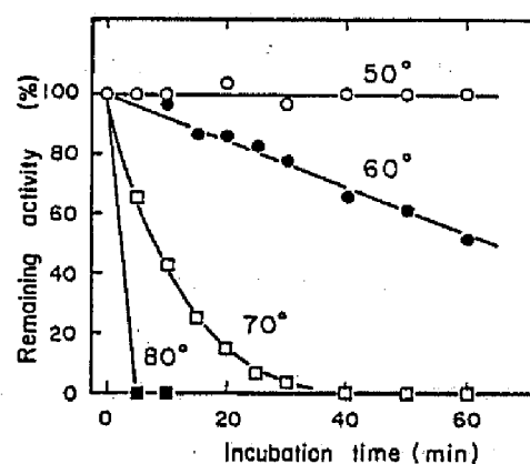
FIG. 3. Temperature stability of Chromatium superoxide dismutase. The purified enzyme (13.4 \mu\text{g/ml} ) in 10 mM potassium phosphate, pH 7.8, was incubated at the indicated temperatures. Aliquots were withdrawn at intervals and then assayed for the remaining enzyme activity under standard conditions at 25°C as described under Materials and Methods.
