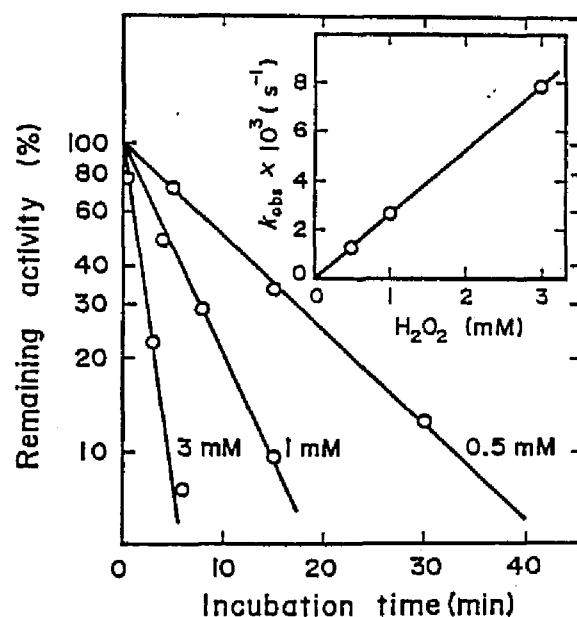
Fig.2 Inactivation of SOD from the cultured cells by \text{H}_2\text{O}_2 . The extract in 10 mM potassium phosphate, pH 7.8, containing 0.1 mM EDTA was incubated at 25^\circ\text{C} with \text{H}_2\text{O}_2 at various concentrations, and aliquots were withdrawn at intervals and assayed for residual enzymatic activity in the standard assay system containing 500 units catalase.
