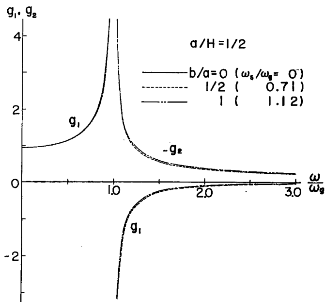
Fig. 5 Dynamic Effects of Horizontal Earth Pressure (in the Direction of Minor Axis)
