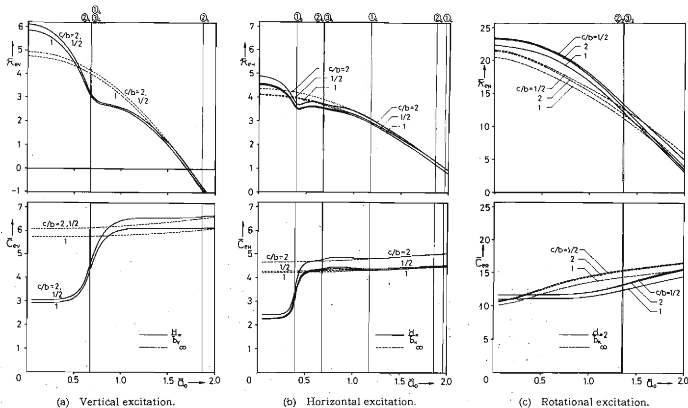
Fig. 9. Equivalent coefficients of Dynamical Ground Compliance for various shapes of foundation. (\nu=1/4, \lambda'/\mu'=1, \bar{\eta}=0.5, \text{ and } H/b_1=4 \text{ in Figs. 9(a) and 9(b) and } 2 \text{ in Fig. 9(c), respectively.})
