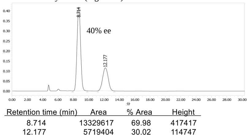
Figure S2 | Chiral HPLC chromatograms of kinetic resolution of racemic- 13 on a preparative scale (Figure 53). Conditions for HPLC: CHIRALPAK IC column (4.6×250 mm); eluent 1:60 EtOH/CH 2 Cl 2 ; flow rate 0.7 ml/min; detection 254 nm, temperature 20 °C. (A) Crude product of a kinetic resolution of racemic- 13 on a preparative scale. (B) Isolated recovered- 13 . (C) Isolated acylate 14 .
