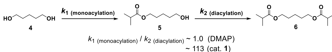
Figure 12 | Relative rate for acylation ( k_1 (monoacylation) / k_2 (diacylation)) between diol 4 and monoool 5.
