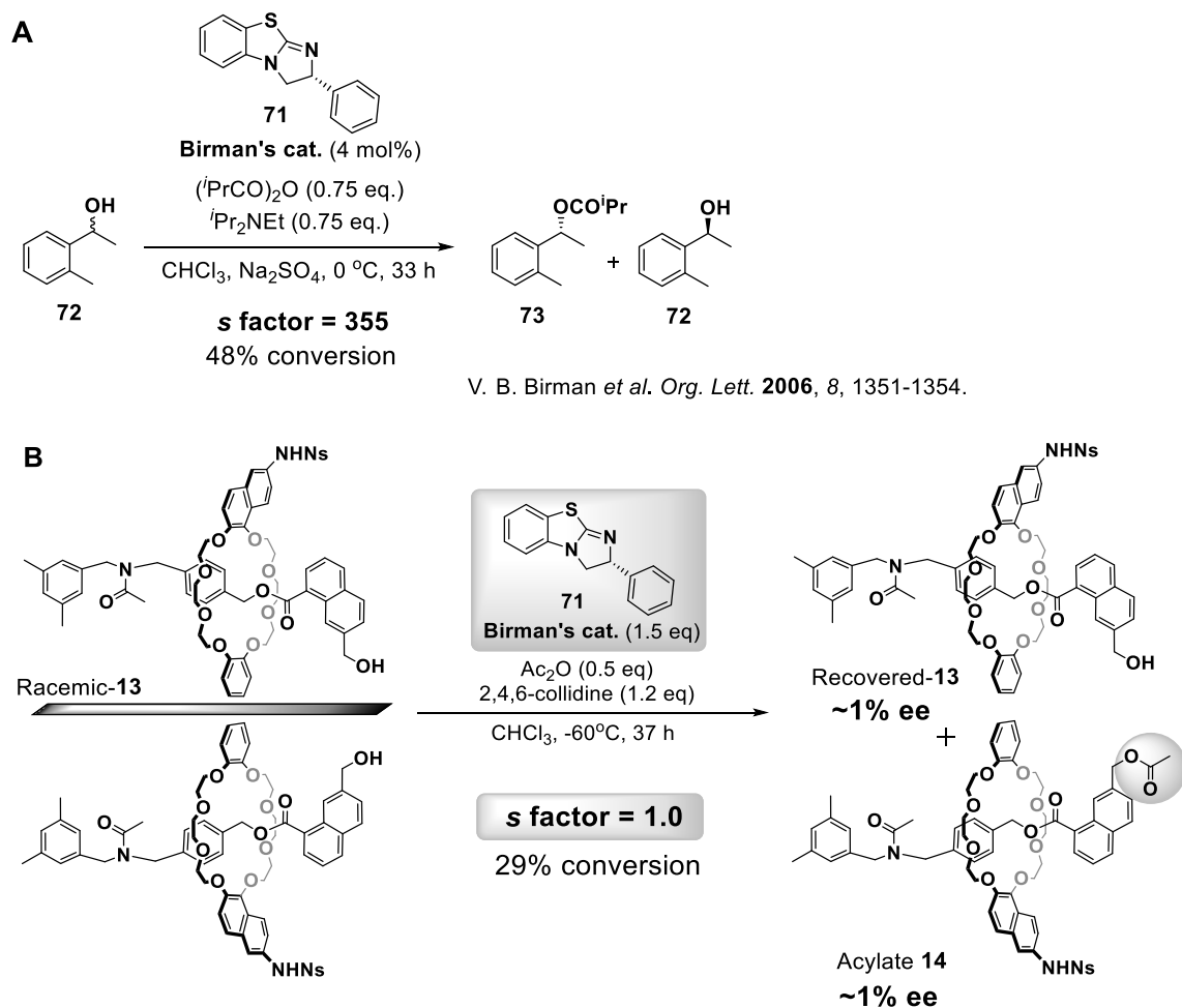
Figure 54 | Acylative kinetic resolution of alcohols with Birman's catalyst 71 . (A) Highly selective acylative kinetic resolution of alcohols 72 with Birman's catalyst 71 . (B) Kinetic resolution of topologically chiral racemic rotaxane 13 with Birman's catalyst 71 .
