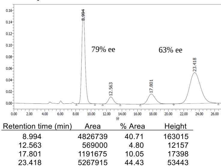
Figure S1 | Chiral HPLC chromatograms of kinetic resolution of racemic-4 on an analytical scale (Figure 50, entry 5). Conditions for HPLC: CHIRALPAK IC column (4.6×250 mm); eluent 1:60 EtOH/CH 2 Cl 2 ; flow rate 0.7 ml/min; detection 254 nm, temperature 20 °C. (A) Racemic-13. (B) Racemic-14. (C) Crude product of a kinetic resolution of racemic-13 on an analytical scale (Figure 51, entry 5).
