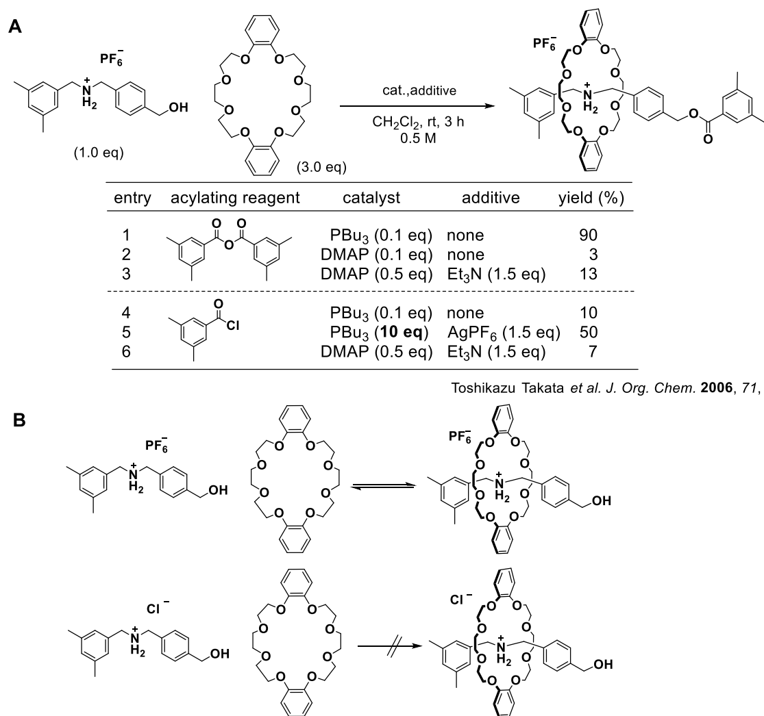
Figure 25 | DMAP-catalyzed synthesis of rotaxanes. (A) Reported synthesis of a rotaxane by DMAP catalysis or tributylphosphine catalysis. (B) Effects of the counter anion of the ammonium salts on the formation of pseudorotaxanes.
