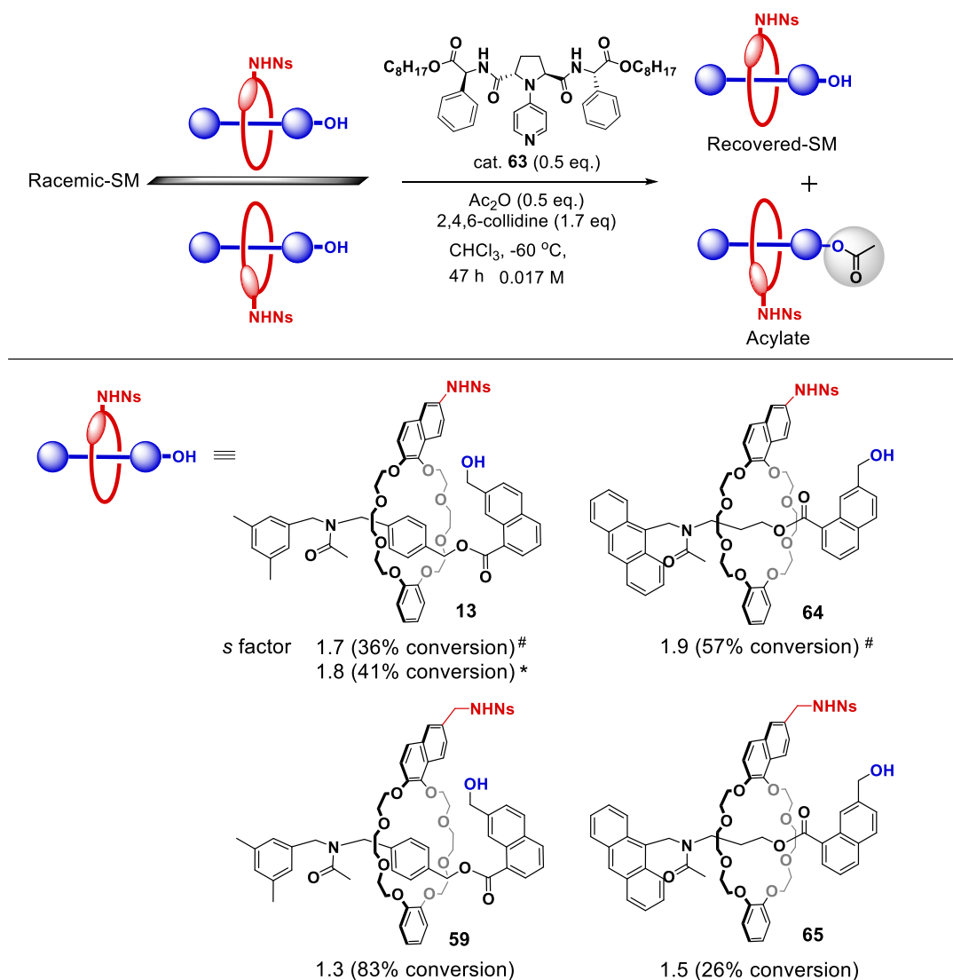
Figure 48 | Initial screening of structure of substrates. #Run in 0.007 M solution. *Reactions performed with 0.1 equivalents of catalyst 3 in 0.07 M solution for 6 days. (i\text{-PrCO})_2\text{O} (0.9 equivalents) was used instead of acetic anhydride.
