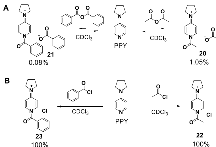
Figure 27 | Formation of acylpyridinium ion pairs. (A) Formation of acylpyridinium ion pairs from acid anhydride. Conditions: PPY (0.015 M), acid anhydride (0.005 M), -60^\circ\text{C} . (B) Formation of acylpyridinium ion pairs from acyl chloride. Conditions: PPY (0.07 M), acyl chloride (0.07 M), 20^\circ\text{C} .
