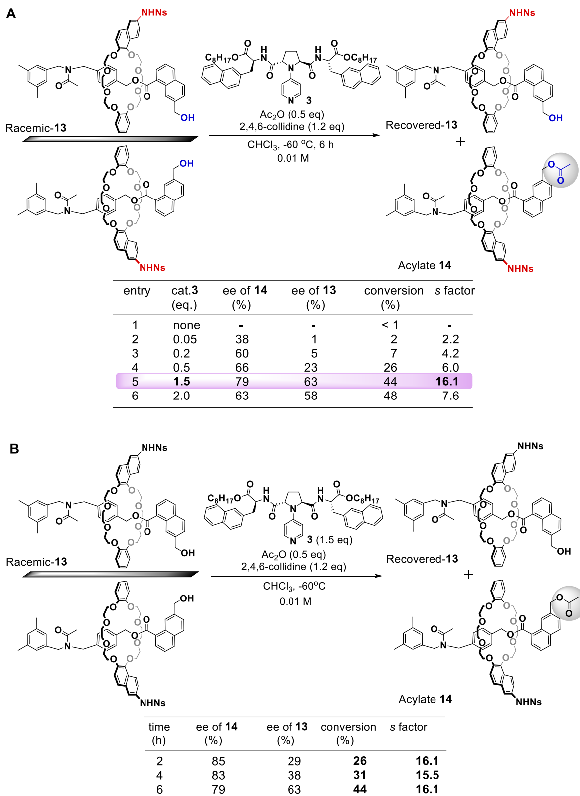
Figure 51 | Effects of catalyst/substrate ratio. (A) Effects of catalyst/substrate ratio on selectivity factors. Both % conversion (C) and selectivity factor (s) were calculated from ee's of the product and the recovered starting material: C = \frac{ee_{\text{recovered SM}}}{(ee_{\text{recovered SM}} + ee_{\text{product}})} , s = \frac{\ln[(1-C)(1-ee_{\text{recovered SM}})]}{\ln[1-C(1+ee_{\text{recovered SM}})]} = \frac{\ln[1-C(1+ee_{\text{product}})]}{\ln[1-C(1-ee_{\text{product}})]} . (B) Effects of conversion on selectivity factors.
