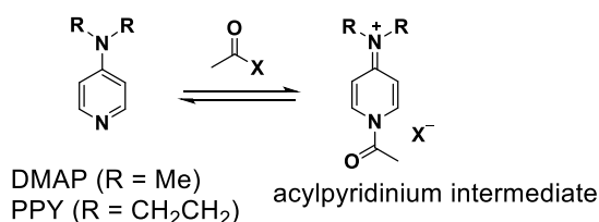
Figure 26 | Acylpyridinium intermediate.
