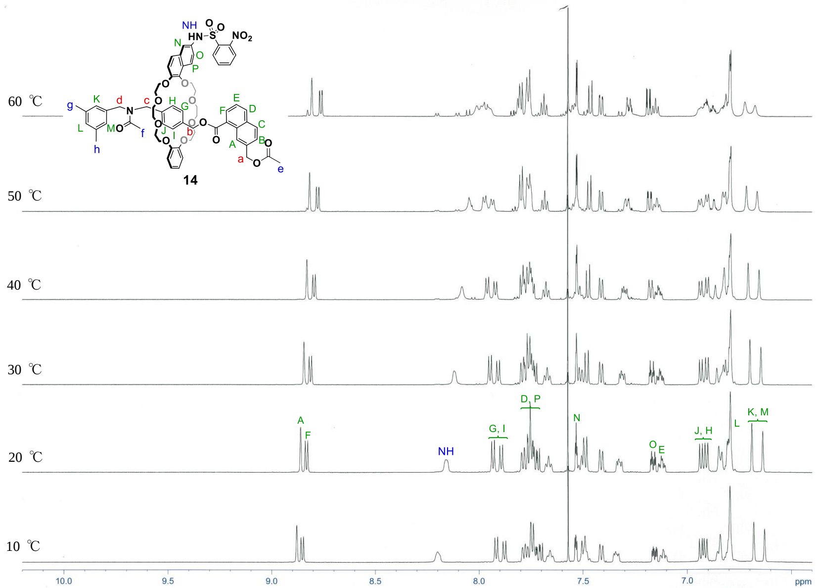
Figure 40 | Variable-temperature NMR spectra of rotaxane 14 . Conditions: Heating a CD 3 CN solution of rotaxane 14 from -40 °C to 60 °C.
