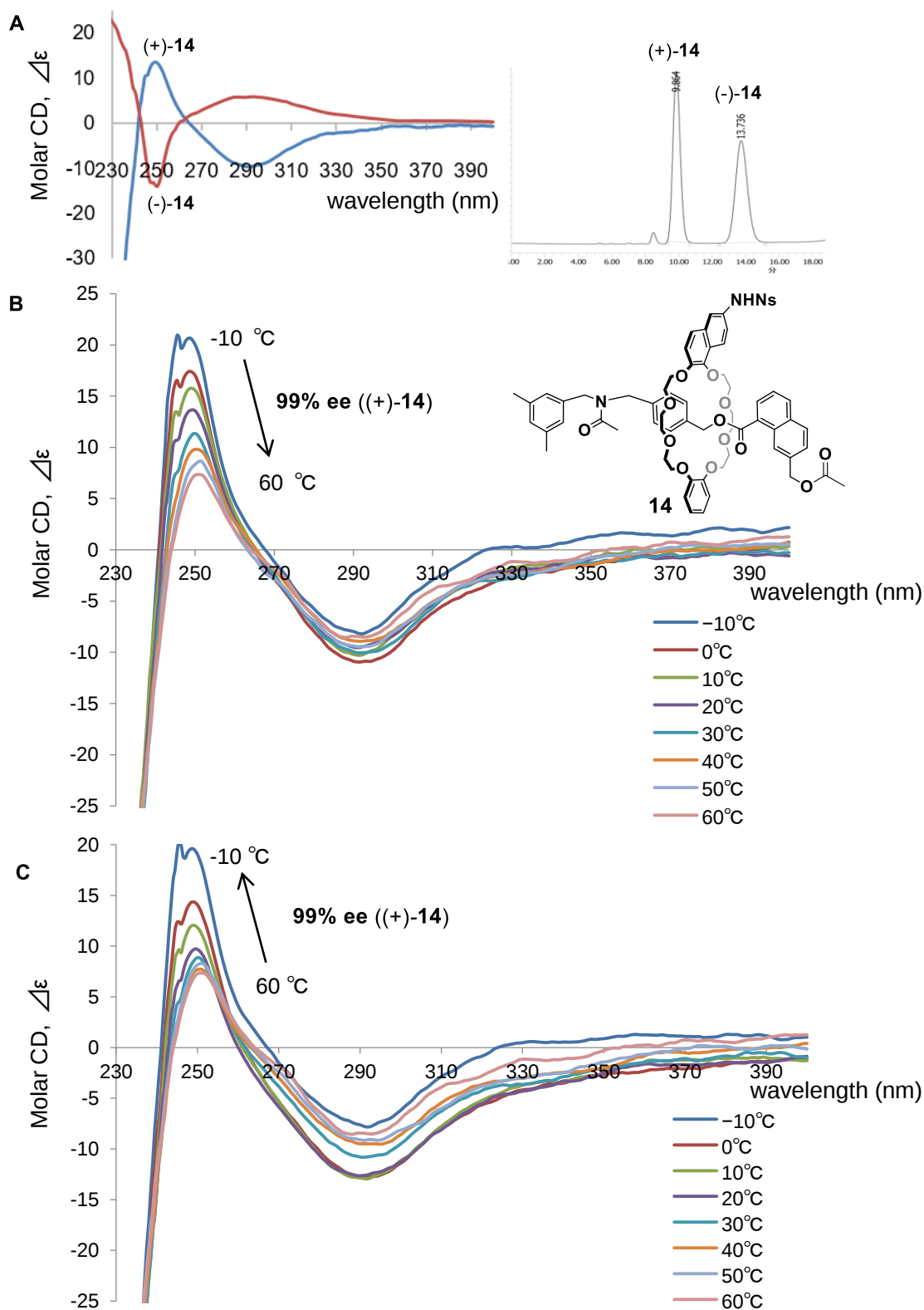
Figure 38 | CD spectra of rotaxane 14. (A) CD spectra and chiral HPLC chromatograms of a pair of enantiomers of rotaxane 14 . CD spectra were recorded in 1.38 \times 10^{-5} M MeCN at 20 °C. Conditions for HPLC: CHIRALPAK IC column ( 4.6 \times 250 mm); eluent 1:60 EtOH/CH 2 Cl 2 ; flow rate 0.7 ml/min; detection 254 nm, temperature 20 °C. (B, C) Variable-temperature CD spectra of (+)- 14 measured by heating (B), or cooling (C) a solution. Recorded in 1.38 \times 10^{-5} M MeCN.
