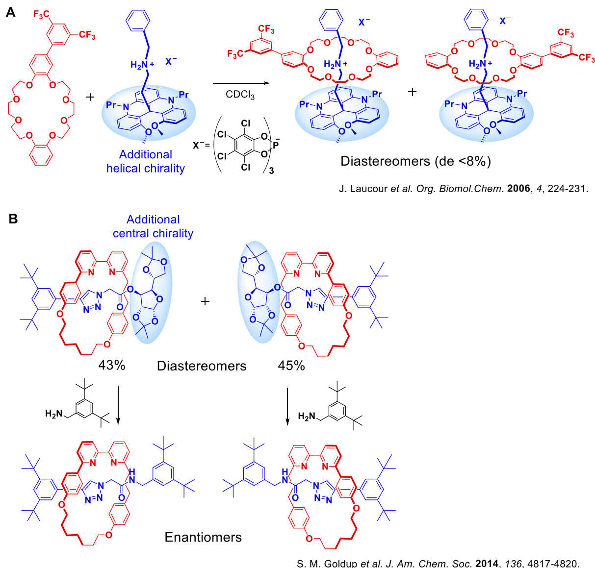
Figure 35 | Diastereomeric rotaxanes with a topological chirality and an additional chirality. (A) Attempts to diastereoselective synthesis of pseudorotaxanes. (B) Separation of diastereomers for preparation of topologically chiral rotaxanes. Diastereomers consist of a topological chirality and a central chirality.
