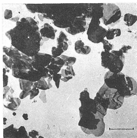
(6) Sericite ( \times 10,000 )
