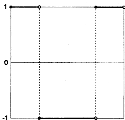
w_3(x)
